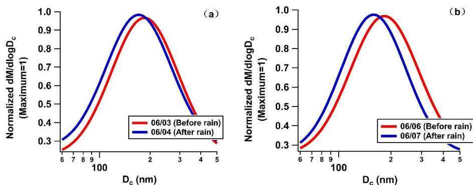
40 Figure S7 Size distribution of the rBC core before and after the typical rain cases.
