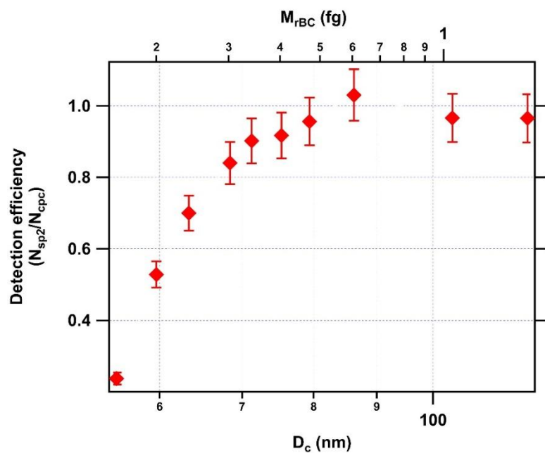
Figure S3 Calibration curve for SP2's detection efficiency.
