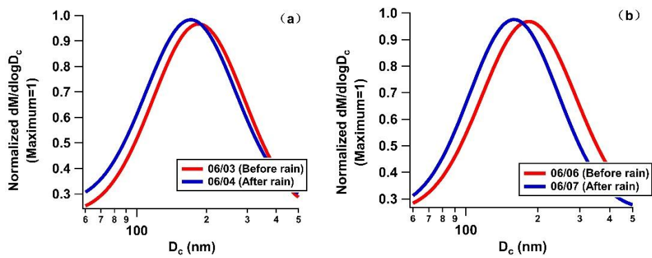
Figure S7 Size distribution of the rBC core before and after the typical rain cases.
