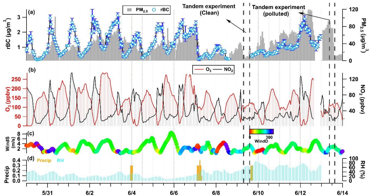
Figure 3. Time series of aerosol/gaseous pollutants and meteorological conditions during the observation period.
