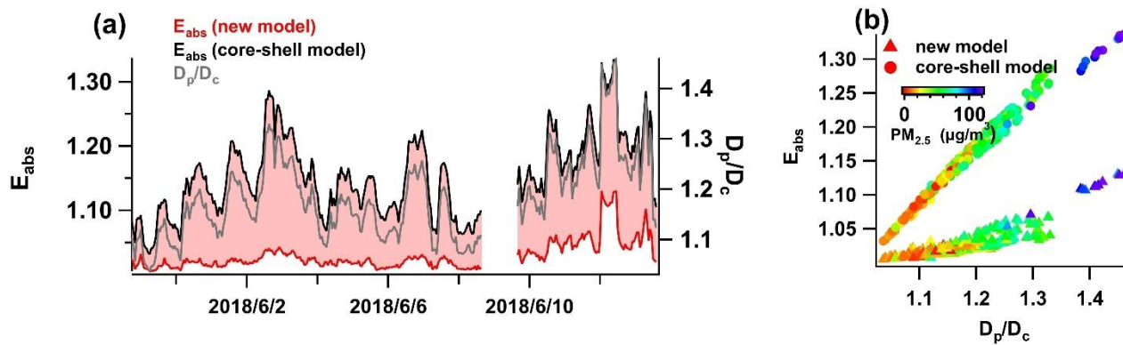
750 Figure 12. (a) Time series of D_p/D_c with D_c=180\pm10 nm and E_{abs} at 550 nm wavelength with D_c=180\pm10 nm using the core-shell model and the morphology-dependent model. (b) Relationship between E_{abs} and D_p/D_c . Circles denote the E_{abs} derived from the core-shell model, and triangles denote the E_{abs} derived from the morphology-dependent model.
