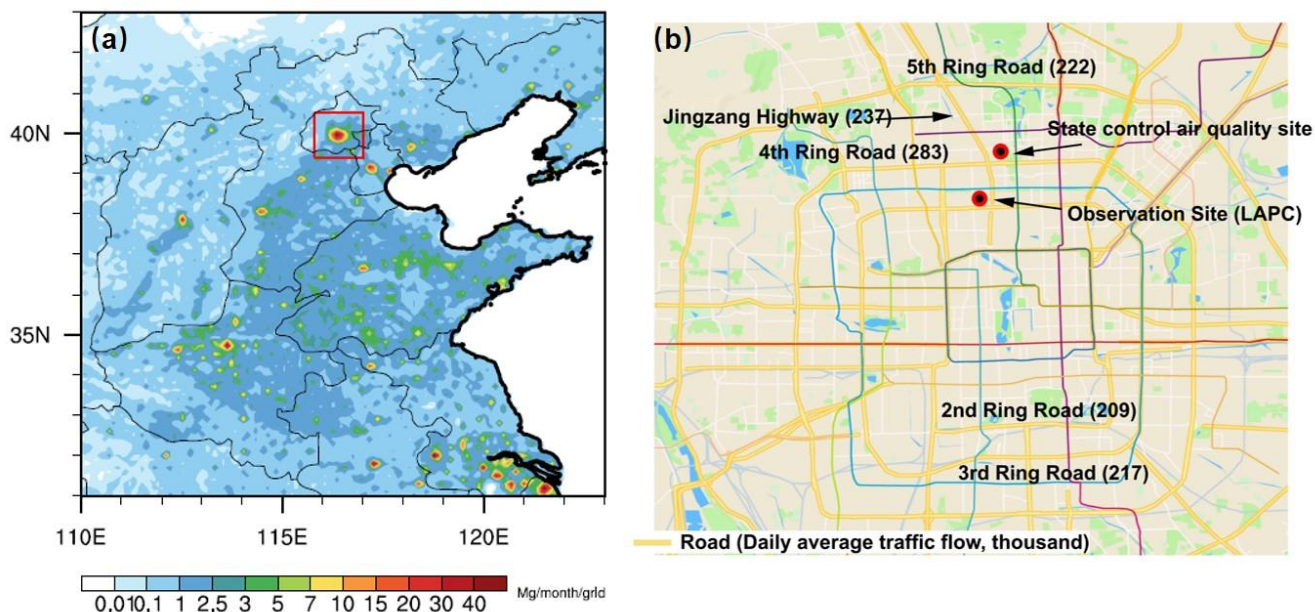
Figure 1. (a) Monthly emissions of BC from traffic in June in east-central China. The red box denotes the geographical location of the observation site, the map is extracted from NCL software (© 2019 NCL, www.ncl.ucar.edu). (b) Road map and traffic flow rate of Beijing. The red circle denotes the observation site, the map is extracted from google map (© 2019 Google, www.google.com/maps).
