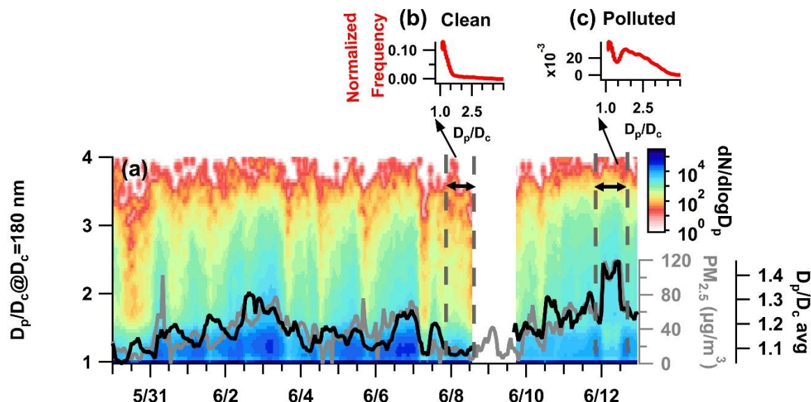
Figure 7. (a) Temporal variation in D_p/D_c , with D_c=180 nm, the image plot denotes the frequency ( dN/d\log D_p ) of rBC-containing particles with varied D_p/D_c . The black line denotes the average D_p/D_c for each hour and the gray line denotes the average concentration of PM_{2.5} for each hour. (b) The normalized dN/d\log D_p versus D_p/D_c for the clean period before the tandem experiment. (c) The normalized dN/d\log D_p versus D_p/D_c for the polluted period.
