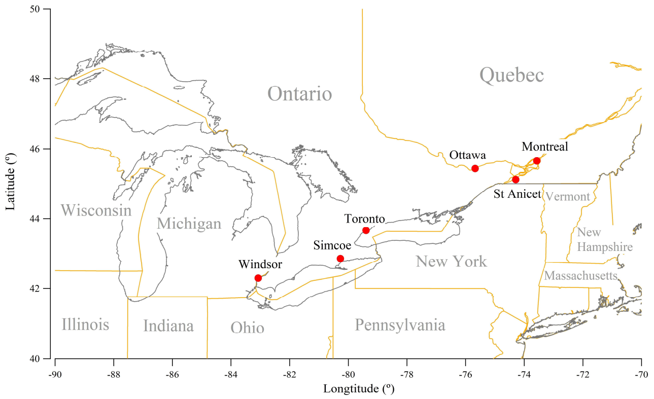
Figure 1. Six NAPS monitoring sites chosen for this study: Toronto, Ottawa, Windsor, Montreal, Simcoe and St Anicet.
