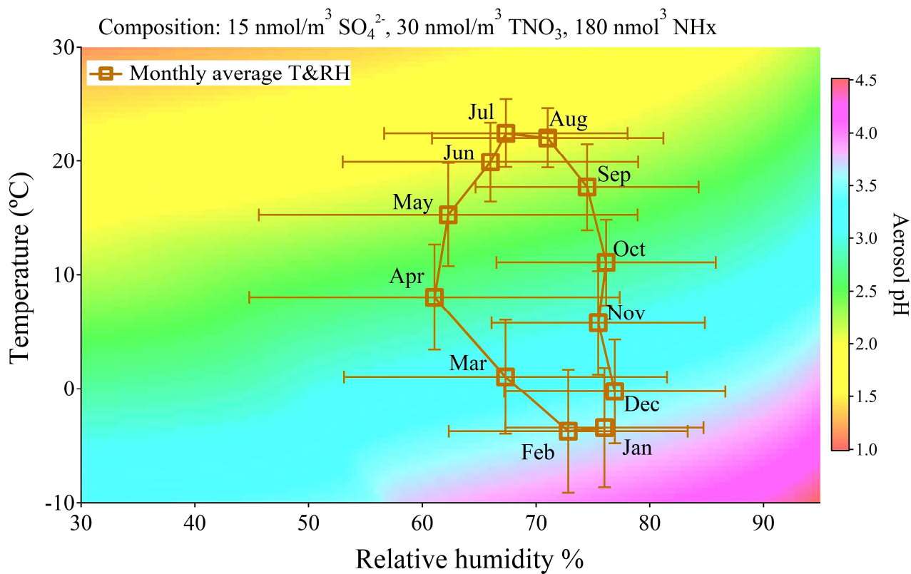
Figure 4. Plot of E-AIM calculated pH under different combinations of relative humidity (from 30%-95%) and temperature (from -10 °C to 30 °C) with the fixed input chemical compositions ( 15 \text{ nmol m}^{-3} sulfate, 30 \text{ nmol m}^{-3} \text{TNO}_3 and 180 \text{ nmol m}^{-3} \text{NH}_x ). The square plots on the graph represent monthly average of meteorological parameters in Toronto from 2007-2016 with standard deviations as error bars.
