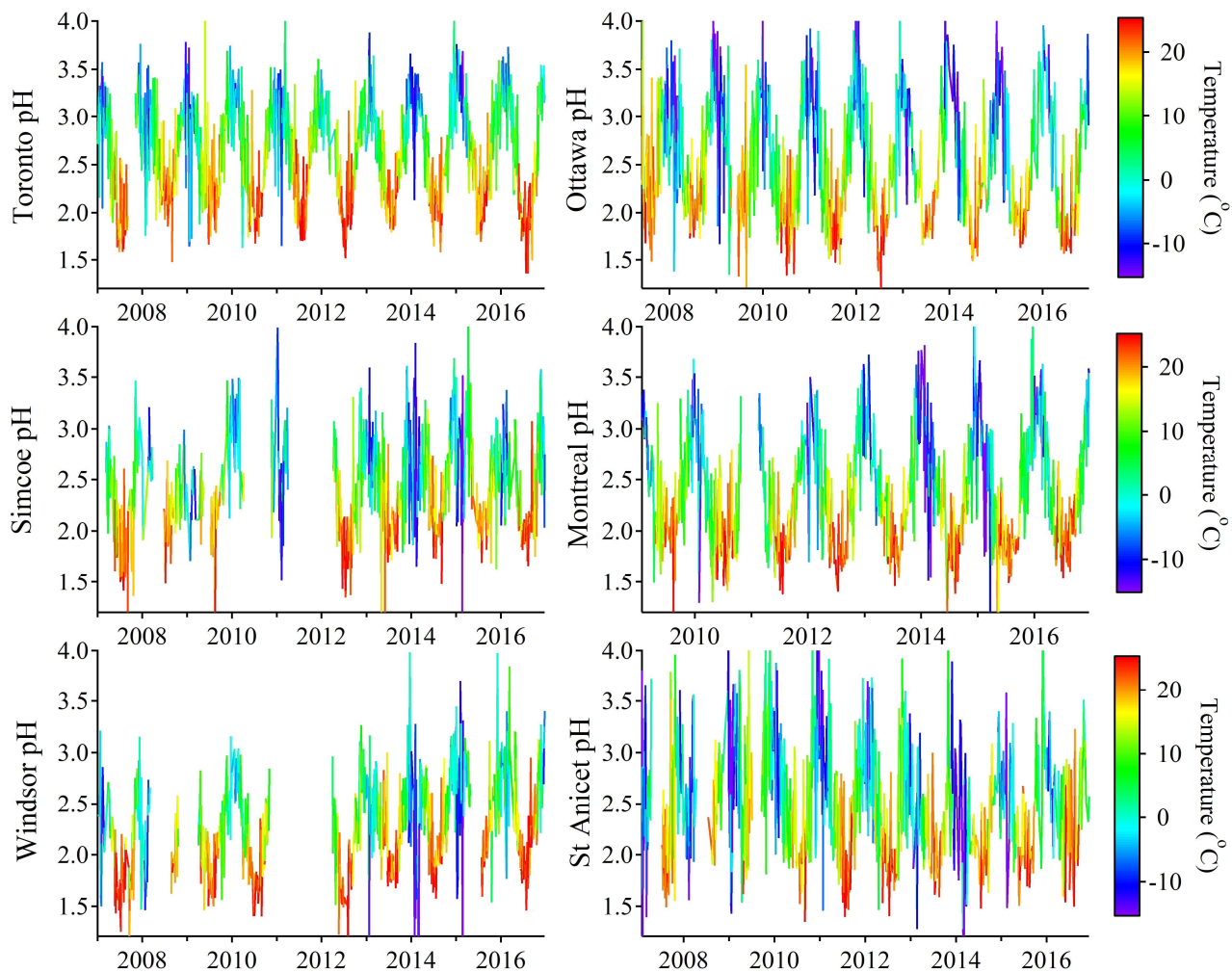
Figure 2. The time series of PM 2.5 pH at six sites colored by ambient temperature.
