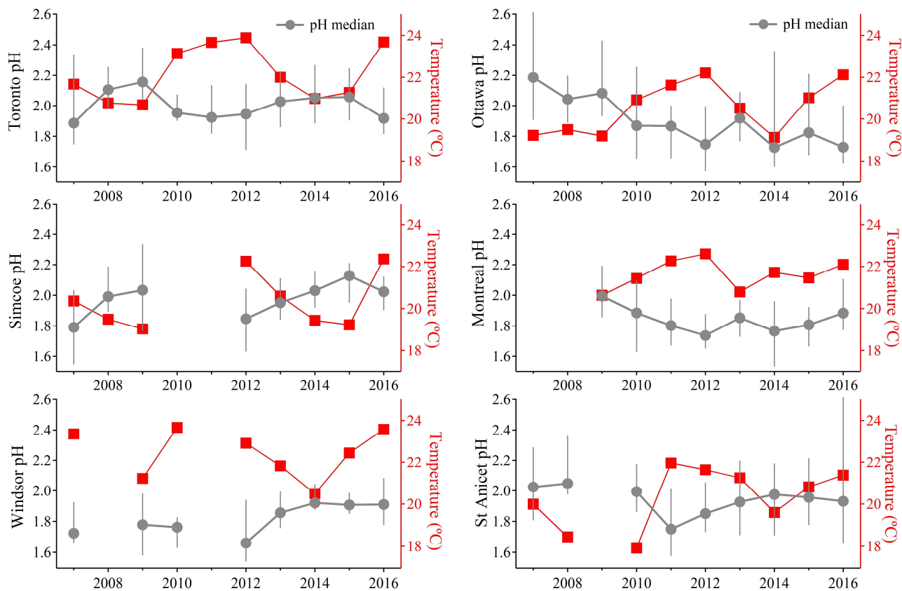
Figure 6. Median of aerosol pH in summertime (data on July and August) from year 2007 to 2016 in six monitoring sites. The error bars with median pH values represent the range from 25% to 75% percentile. Average ambient temperature in summertime (July and August) in each site is also plotted on right axis to illustrate the reverse trend of temperature with pH inter-annual variation.
