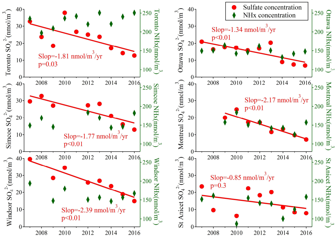
Figure 7. 10-year trends of summertime average concentrations of sulfate and \text{NH}_x in each site. Linear regressions of sulfate were illustrated on each graph to represent the reduction of particulate sulfate from 2007 to 2016.
