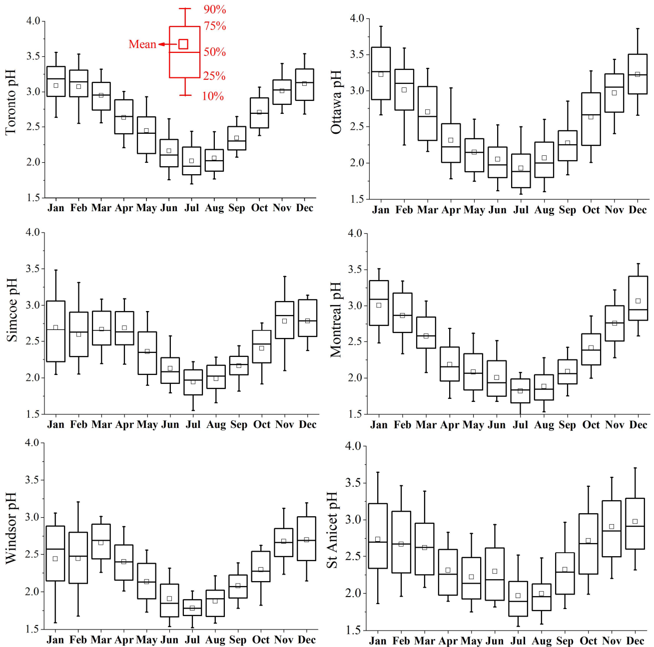
Figure 3. The box and whisker plot of aerosol pH in each month in six sites. In each box, the top, middle and bottom lines represent 75 th , 50 th and 25 th percentile of statistical data, the upper and lower whiskers represent 90 th and 10 th percentile, and the square mark represent the mean value.
