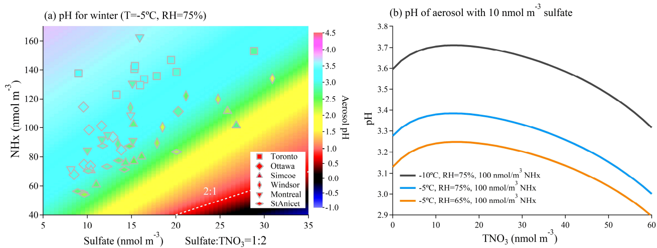
Figure 8. (a) The plot of aerosol pH under wintertime meteorological conditions ( -5^\circ\text{C} , \text{RH}=75\% ) under different combinations of sulfate and \text{NH}_x with more focused region compared to Figure 5(d). The markers on the graph represents the average wintertime (data from January and February) sulfate and \text{NH}_x concentrations in each year in each sampling site with color indicating average pH value. (b) pH of aerosol with 10 \text{ nmol/m}^3 sulfate under different combinations of temperature and relative humidity as the function of \text{TNO}_3 in the system.
