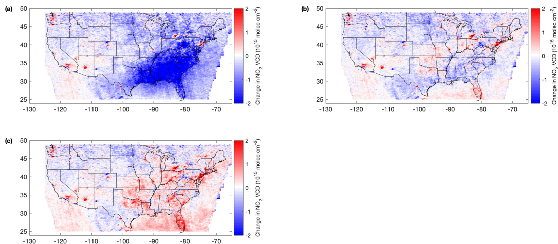
Figure 4. Difference in \text{NO}_2 VCD between BEHR retrievals and WRF-Chem. (a) excludes \text{LNO}_x in model simulation, (b) adds \text{LNO}_x emission with production rate of 500 \text{ mol NO flash}^{-1} . (c) includes the same \text{LNO}_x emission as (b) but uses \text{NO}_2 profiles scaled upward by 60% at pressure lower than 400 hPa. The average time covers May 13 to June 23, 2012. Pixels with cloud fraction larger than 0.2 are filtered out in the analysis.
