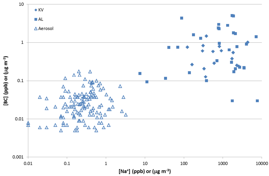
Fig. S3: BC vs. sodium concentrations in snow pit KV (filled diamonds) and AL (filled squares), and in aerosols (open triangles). BC in the snow pits corresponds to rBC, while the BC in aerosols corresponds to eBC.
