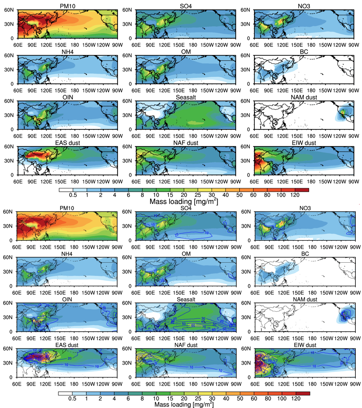
5 Figure 3 Spatial distribution of aerosol composition column mass loading from WRF-Chem averaged for 2010-2014. The trans-Pacific transport aerosol mass spatial distribution is denoted by PM10 and the dust from North America, East Asia,
