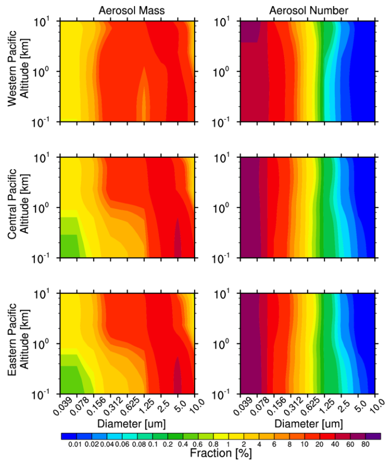
Figure 7. Vertical distribution of fractional contributions to the size of aerosol mass and number over the western, central
