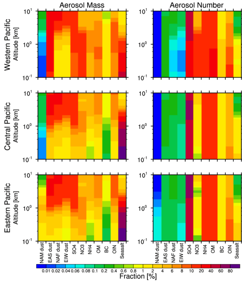
Figure 6. Vertical distribution of fractional contributions to aerosol composition mass and number over the western, central 5 and eastern Pacific from the WRF-Chem simulation averaged for 2010-2014.
