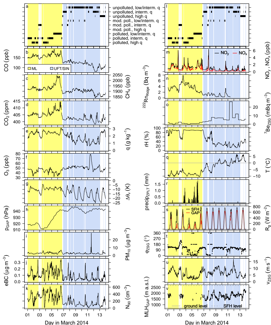
Figure S2. Time series of air mass regimes (a,l), input variables for the classification (b–i), and validation variables (j,k,m–v) from 1 to 13 March 2014. Unless labeled differently, the data was measured at the UFS except for \Delta\theta_v that represents the maximum difference among the sites. The color shading highlights the most important air mass classes. Symbols are explained in Sect. 2.2 and 2.3 of the main article.
