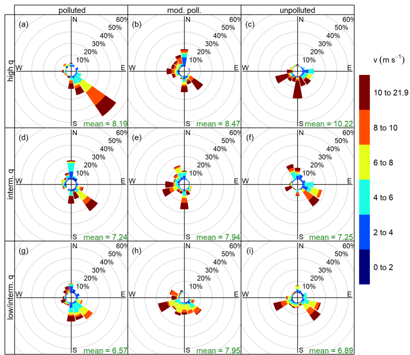
Figure S1. Windrose plots showing the frequency of counts by wind direction and velocity ( v ) at Zugspitze summit for the nine air mass regimes in February and March 2014.
