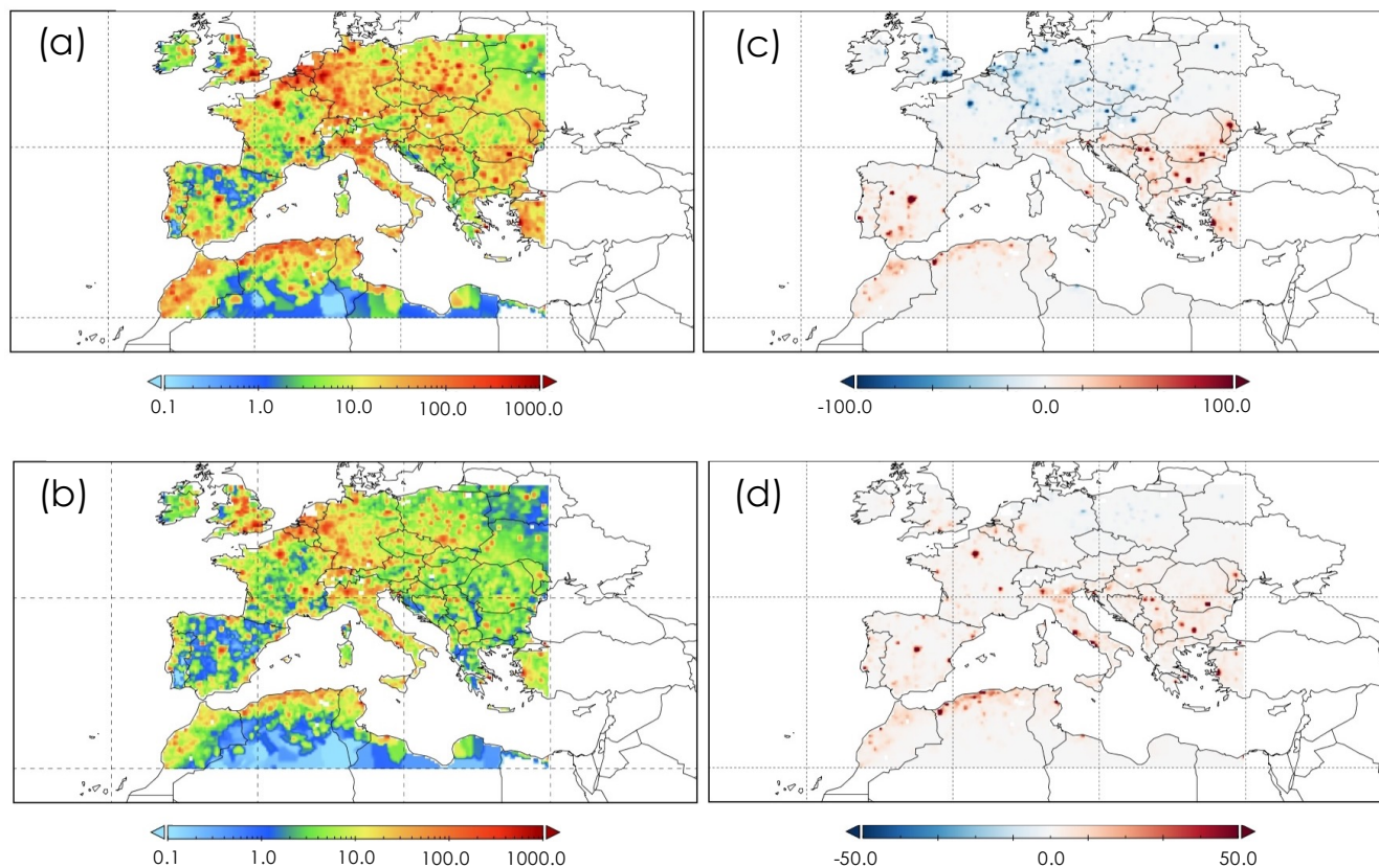
Figure 7. (a) Present cases of Premature Deaths (PD) and (b) associated costs, in M€. (c) Changes projected in PD and (d) changes in costs (M€) under the RCP8.5 scenario (2071-2100).
