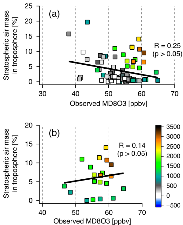
5 Figure 10. Relationship between observed MD803 at the surface and the estimated stratospheric air mass contributed to total tropospheric O 3 column as monthly-average during April 2010. The points are color coded based on elevation of each site. (a) All CASTNET sites (except Alaska), and (b) elevated CASTNET sites defined as having an elevation greater than 1000 m (see also Table S3).
