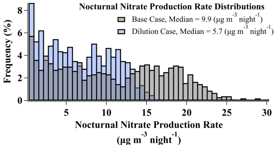
Figure 9. Histograms of nocturnal nitrate production rates ( \mu\text{g m}^{-3} \text{night}^{-1} ) predicted by base case simulations and simulations incorporating a first-order dilution loss process with rate constant k_{\text{dilution}} = 1.3 \times 10^{-5} \text{ s}^{-1} .
