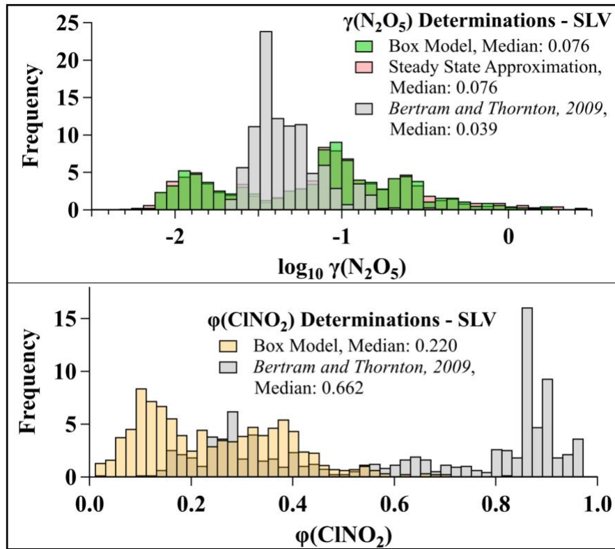
Figure 8. (Top) Histograms of \gamma(\text{N}_2\text{O}_5) determinations from the SLV during pollution events, calculated with the box model (green), steady state approximation (pink), and parameterization from Bertram and Thornton (2009). (Bottom) Histograms of \phi(\text{CINO}_2) determinations from the SLV during pollution events calculated with the box model (gold) and parameterization from Bertram and Thornton (2009) (gray).
