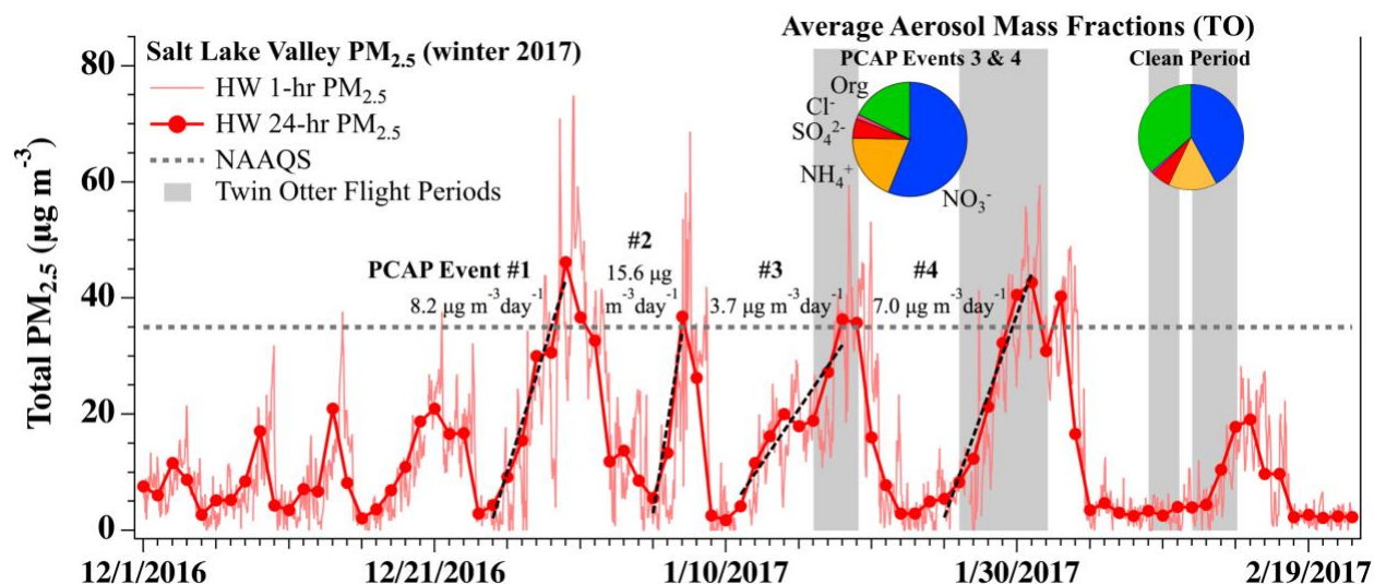
5 Figure 4. Time series of total \text{PM}_{2.5} mass ( \mu\text{g m}^{-3} ) (1-hr and 24-hr averages) for the 2016-2017 winter, measured at the Hawthorne (HW) UDAQ site in the SLV. Dashed black lines are daily \text{PM}_{2.5} accumulation rates (rates given in Figure). The 24-hour EPA national ambient air quality standard for \text{PM}_{2.5} ( 35 \mu\text{g m}^{-3} ) is shown by the dashed gray line. Gray shading indicates days when the TO aircraft was flying during UWFPS. Average aerosol mass fractions measured by the AMS aboard the TO are given in pie charts for polluted and clean conditions. Aerosol components are colored by nitrate (blue), ammonium (gold), sulfate (red), non-refractory chloride (pink), and organics (green).
