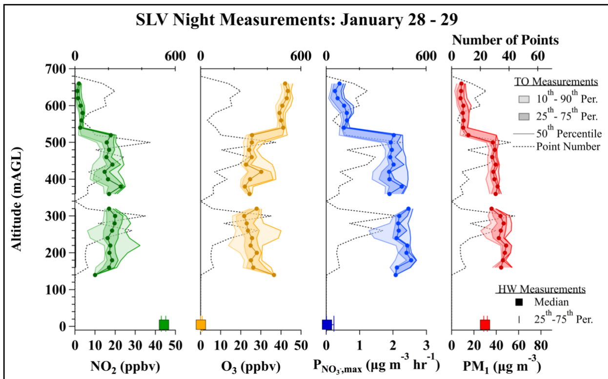
Figure 7. Vertical Profiles of NO 2 , O 3 , P NO 3 ,max (1-second data), and PM 1 (10-second data) measured from the TO aircraft during 5 box patterns, flown over the SLV urban core between 21:20 and 00:30 MST on 28 and 29 January. Percentiles and number of points at each altitude are shown as in Figure 6. Square markers and error bars represent the median and 25 th -75 th percentile range of NO 2 , O 3 , P NO 3 ,max , and PM 2.5 measured concurrently at the HW ground site.
