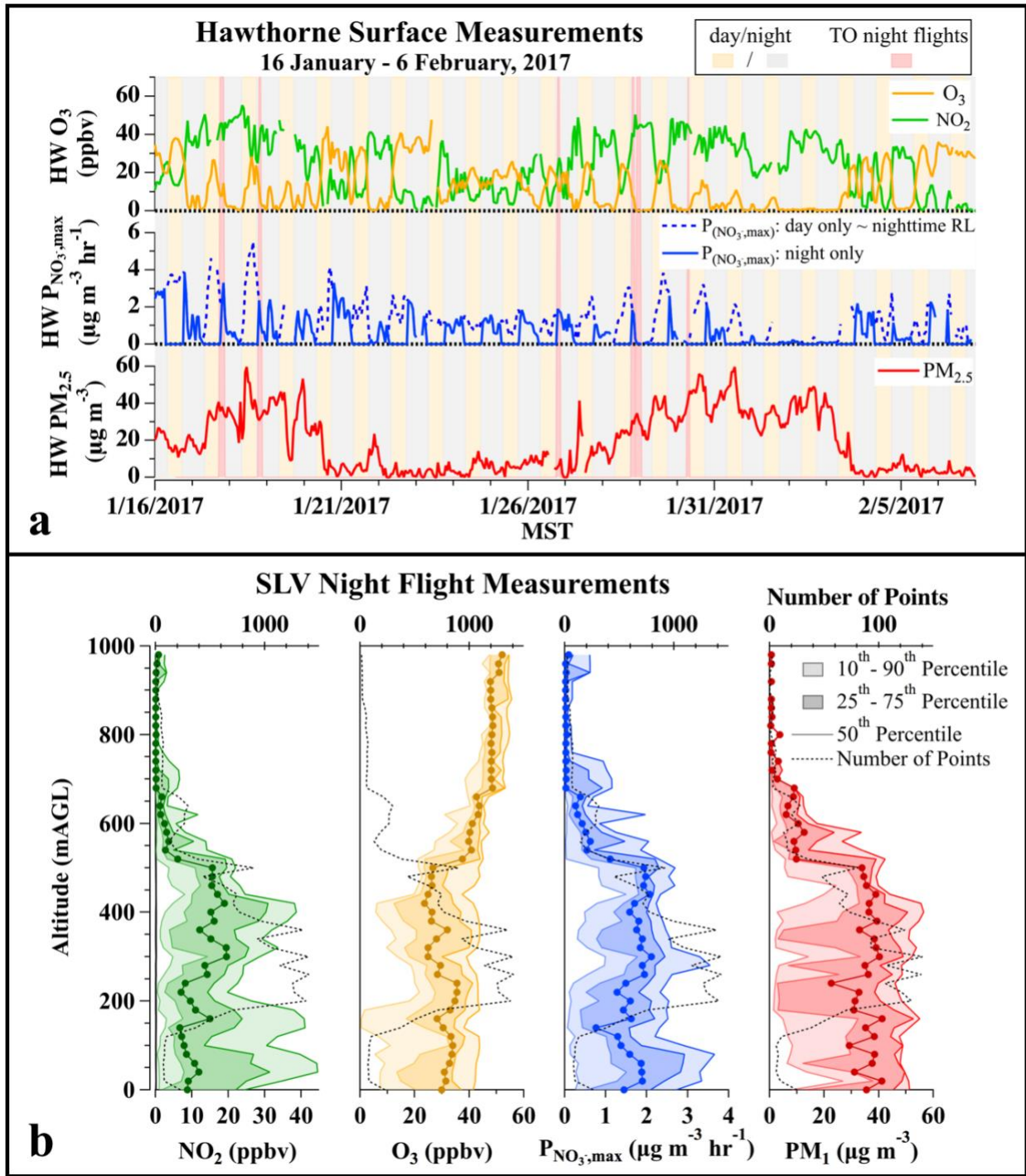
Figure 6. (a) Time series of \text{NO}_2 , \text{O}_3 (top), P_{\text{NO}_3^-}{}_{\text{max}} (middle, see text for definition), and \text{PM}_{2.5} (bottom) measured at the HW ground site during 16 January – 6 February 2017. \text{O}_3 data during the middle January pollution event were corrected to account for a 4.5 ppbv offset in the HW measurements, as shown in Figure S4. Aircraft flight times are shown by red shading. Dashed blue line shows the calculated P_{\text{NO}_3^-}{}_{\text{max}} rates that would occur during the day if this mechanism were operative. Solid blue line assumes nitrate production from this mechanism during the day is zero. Late afternoon P_{\text{NO}_3^-}{}_{\text{max}} at the surface (dashed line), is roughly equivalent to the P_{\text{NO}_3^-}{}_{\text{max}} expected in the RL at night. (b) Vertical profiles of \text{O}_3 , \text{NO}_2 , P_{\text{NO}_3^-}{}_{\text{max}} (1-second data) and \text{PM}_1 (10-second data) measured from the aircraft on all night flights over the SLV. In each panel, light shaded regions show the 10 th -90 th percentile ranges, dark shaded regions are the 25 th -75 th percentile ranges, and the solid lines are the 50 th percentile. Dashed black lines show the number of points at each altitude.
