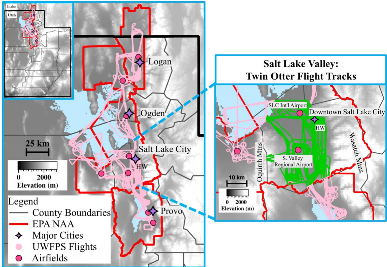
Figure 1. (Left) Elevation Map of Utah's Wasatch region (Utah State in insert), with the Great Salt Lake (north) and Utah Lake (south) shown in blue and county borders in black. U.S. EPA designated non-attainment areas (NAA) for PM 2.5 are shown by red boundaries. From north to south these NAAs include the Logan NAA: "Moderate" status, Salt Lake City NAA: "Serious" status, and Provo NAA: "Serious" status. UWFPS TO flight tracks are shown in pink. Purple markers indicate the locations of major cities, including Logan in the Cache Valley, Ogden and Salt Lake City in the SLV, and Provo in the Utah Valley. The location of missed approaches conducted with the aircraft are shown by dark pink circles. The Hawthorne (HW) measurement site in the SLV is labeled. (Right) Expanded view of the SLV, with analyzed flight tracks highlighted in green.
