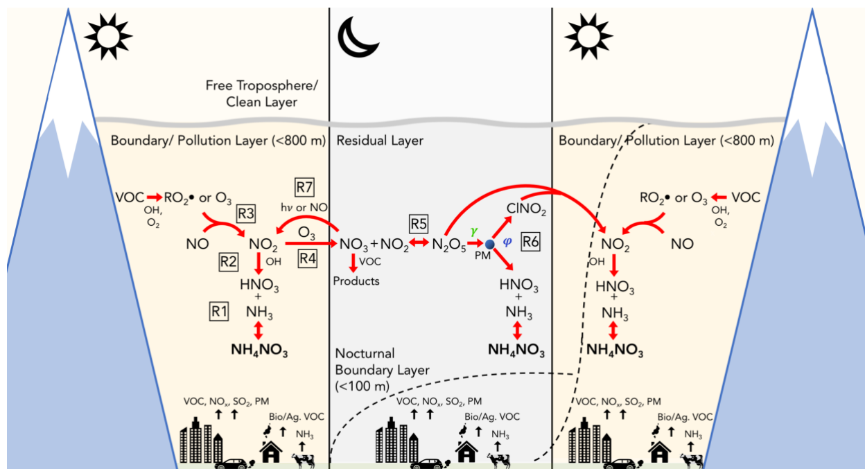
Figure 2. Illustration of the day-night dynamics and chemical cycles of reactive nitrogen oxides, O_3 , and NH_4NO_3 during PCAP conditions in the SLV. The development of the nocturnal boundary layer and morning growth and mix-out are illustrated by the dashed lines. Figure is not to scale. (R6) represents the reaction: N_2O_5 \xrightarrow{\gamma(N_2O_5), M} 2 * (1 - \phi) * HNO_3 + \phi * ClNO_2 .
