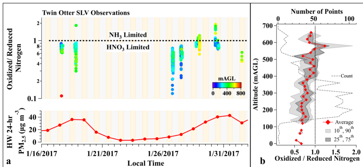
10 15 Figure 5. (a, top) Time series of ratio of total oxidized ( \text{HNO}_3 + \text{NO}_3^- ) to reduced ( \text{NH}_3 + \text{NH}_4^+ ) nitrogen between 16 January and 1 February 2017 (10s averages), calculated from TO observations over the SLV. Individual nitrogen ratios are colored by aircraft altitude (mAGL). Yellow and gray shading indicate times of day and night, respectively. (a, bottom) \text{PM}_{2.5} mass (24-hour average) measured at the HW ground-site (bottom). (b) Vertical profile of oxidized to reduced nitrogen ratios from panel (a). Diamonds represent the average values in each altitude bin and gray shading shows the 10 th -90 th (light gray) and 25 th -75 th (dark gray) percentiles. The number of points in each bin is shown by the gray dashed line. The vertical black line illustrates a nitrogen ratio of 1.
