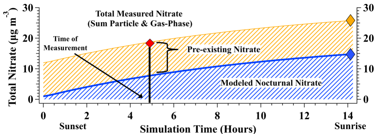
Figure 3. Example simulation of total nitrate production from sunset to sunrise for an air parcel sampled over the SLV on 28 January 2017. Model derived \gamma(N_2O_5) and \phi(ClNO_2) values were 0.05 and 0.21, respectively. Modeled nocturnal nitrate (blue) is the total nitrate produced by heterogeneous chemistry in the box model, with the nocturnal production rate ( \mu g m^{-3} night^{-1} ) represented by the blue diamond. Pre-existing nitrate (yellow) represents the nitrate present at sunset and is calculated as the difference between total measured nitrate from the aircraft (red diamond) and the model-predicted nitrate at the time of aircraft measurement (vertical black line). Assuming pre-existing nitrate is constant overnight (i.e. no deposition or dilution) and constant values of \gamma(N_2O_5) and \phi(ClNO_2) , the fractional contribution of nitrate production from a single night to the total observed is calculated as the ratio of modeled nitrate (blue diamond) to total nitrate (gold diamond) at sunrise.
