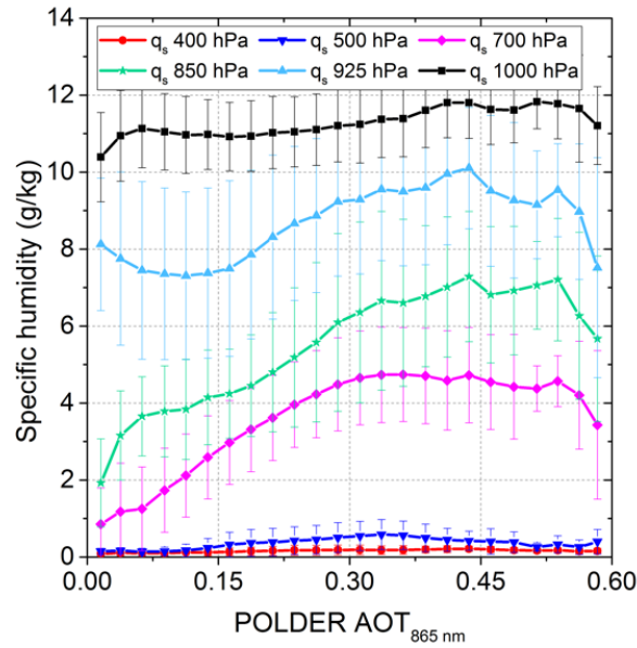
Figure 7: Mean specific humidity as a function of POLDER AOT 865nm retrieved at different pressure levels, within the selected region over June-August 2008. The vertical bars represent the standard deviation for the specific humidity.
