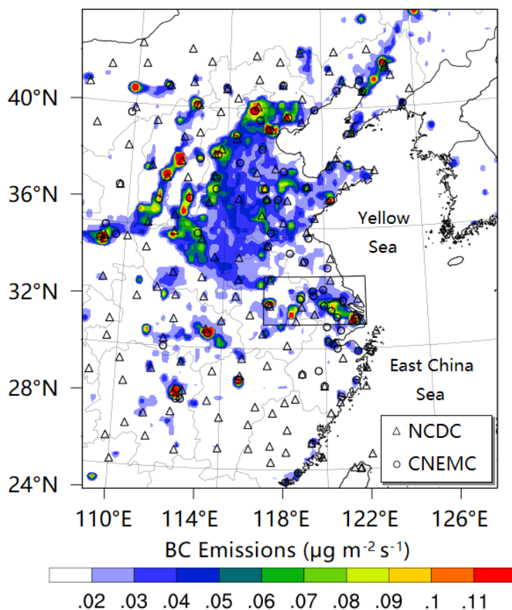
5 Figure 1: A map showing the WRF-Chem model domain, BC emission and observation sites for meteorological parameters and air pollutants. Color filled contours represent the BC emission from EDGAR-HTAP dataset. The triangles represent the locations of 153 meteorological stations over eastern China from NCDC, and the circles represent the locations of the 74 cities from where the pollutant observations are recorded. The rectangle denotes the YRD region.
