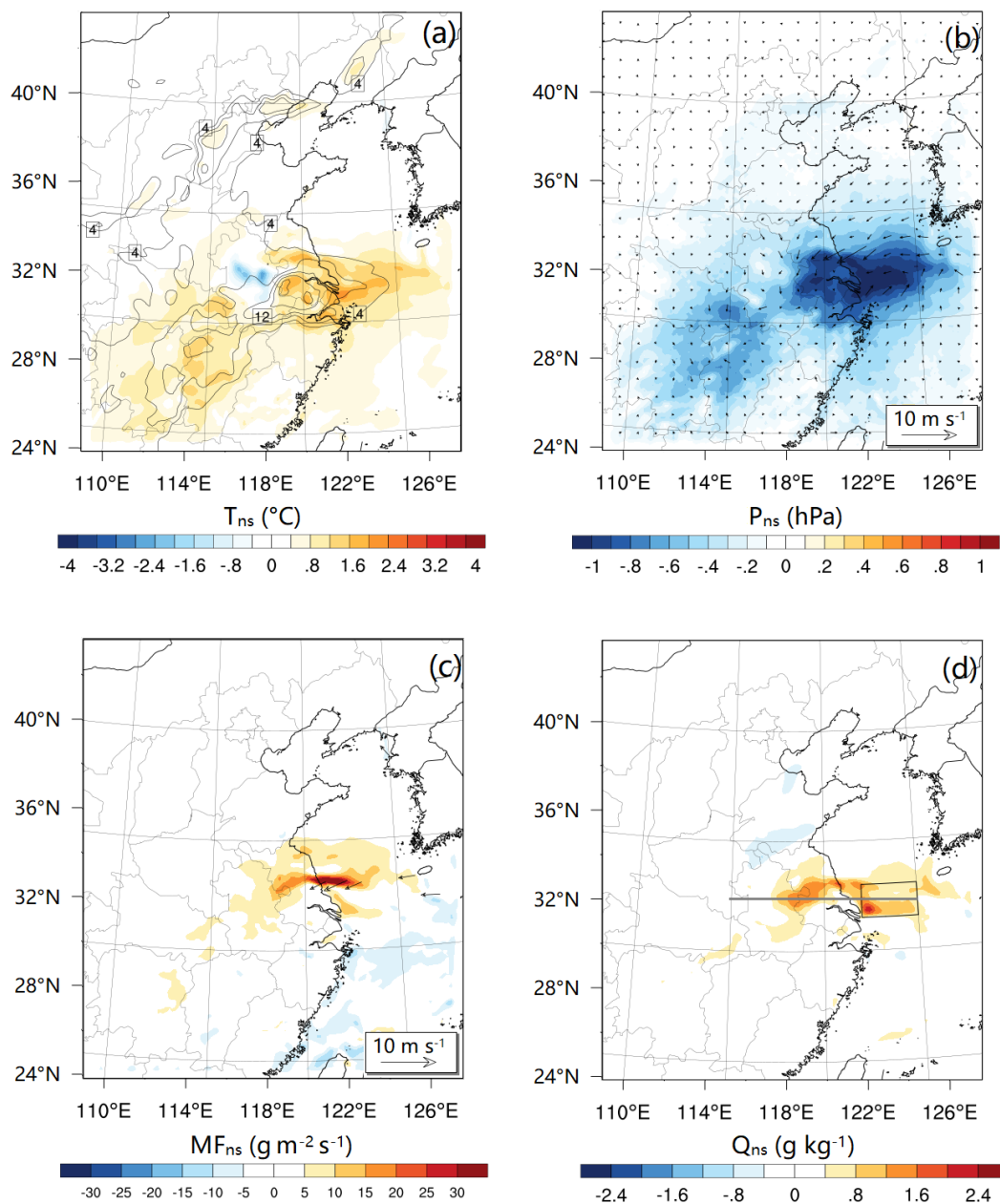
5 Figure 10. BC-introduced increase of air temperature (a), low-pressure perturbation and cyclonic anomaly in wind field (b), increase of moisture advection (c), and increase of water vapour mixture ratio (d) in the surface layer at 14:00 LST on 6 December. Arrows shown in (c) are the BC-induced velocity change with the magnitude larger than 3 \text{ m s}^{-1} , which are used to represent the direction of enhanced horizontal moisture flux. The line in (d) denotes the location where the cross-section of BC-induced increase of temperature and moisture (as well as the PBLH in different experiments) is plotted in Fig. S5, and the rectangle denotes the offshore area, in which the average profiles of potential temperature and water vapor mixture ratio in EXP_CTL and EXP_NOBC are calculated and plotted in Fig. S6.
