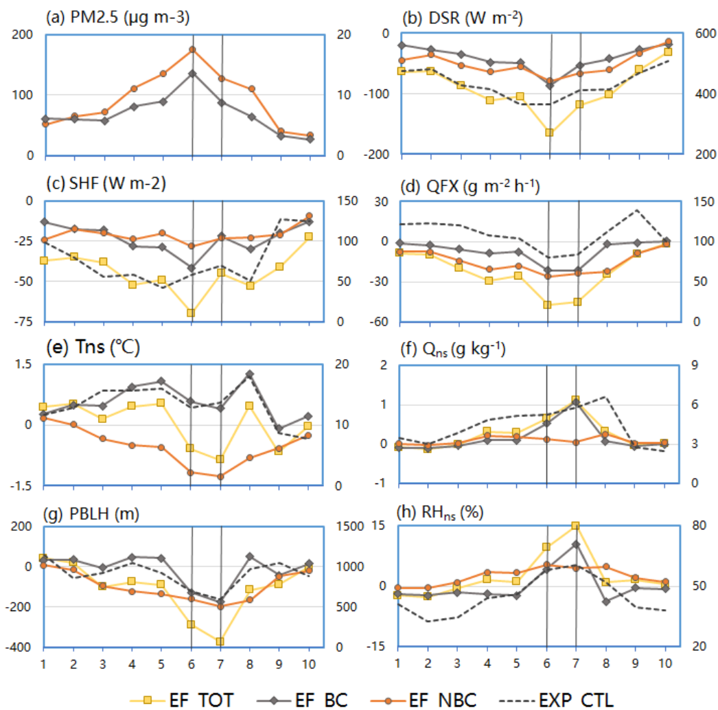
5 Figure 7. The contributions from EF_TOT, EF_BC, EF_NBC to the change in PM 2.5 concentration, DSR, SHF, QFX T ns , Q ns , PBLH and RH ns at 14:00 LST during 1-10 December 2013 (the magnitude is denoted by the left axis). The corresponding values from EXP_CTL (the magnitude is denoted by the right axis) are plotted for reference. The data are calculated from the simulated results at the lowest grid level over the YRD region, as marked in Fig. 1.
