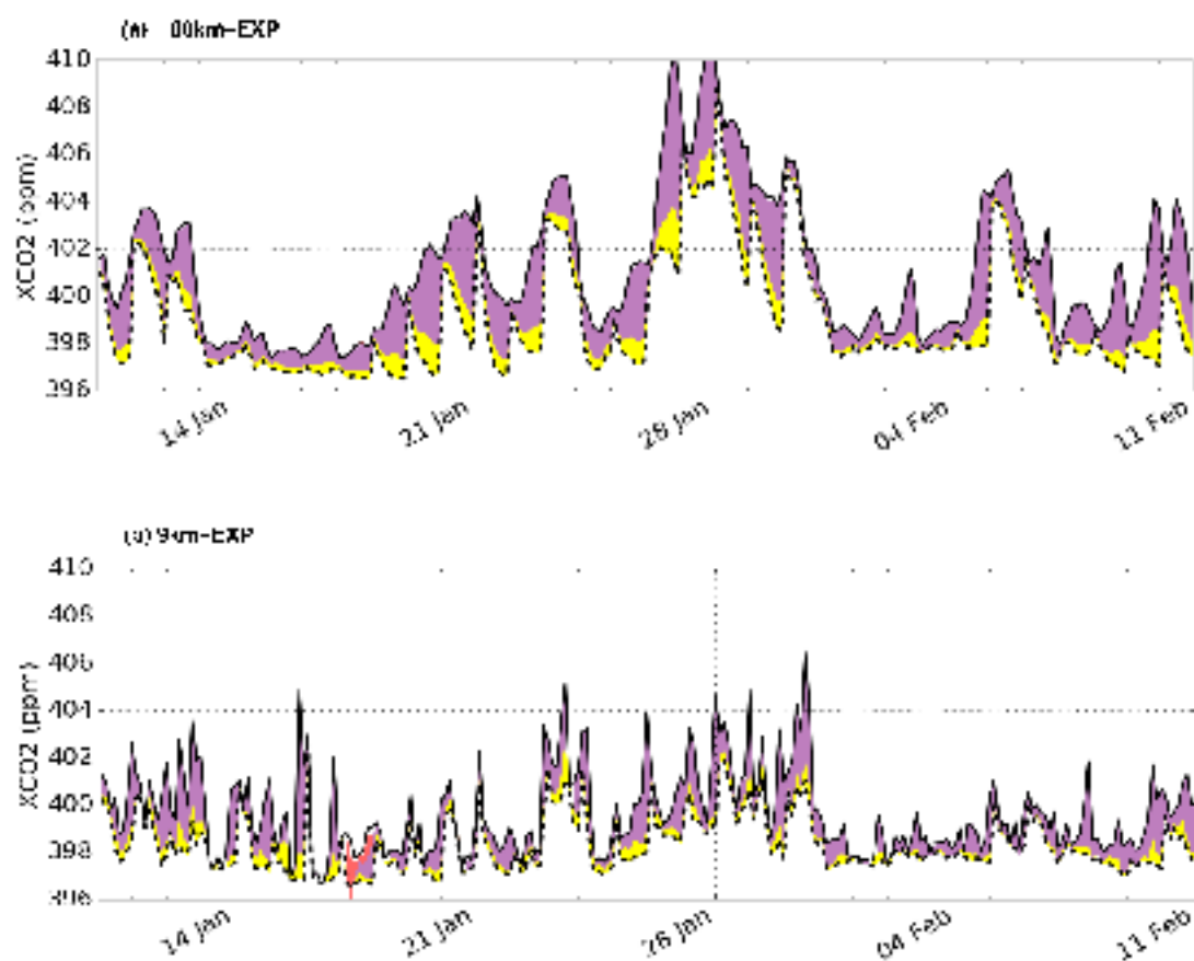
Figure S10. Modelled XCO 2 [ppm] from (a) 80km-EXP and (b) 9km-EXP simulations at the TCCON site of Pasadena (Tab.A3) responding to atmospheric transport and fluxes (solid line) and to only atmospheric transport (dash line). The XCO 2 enhancement associated with the different fluxes is coloured in purple (for anthropogenic emissions), yellow (for biogenic emissions) and red (for fires).
