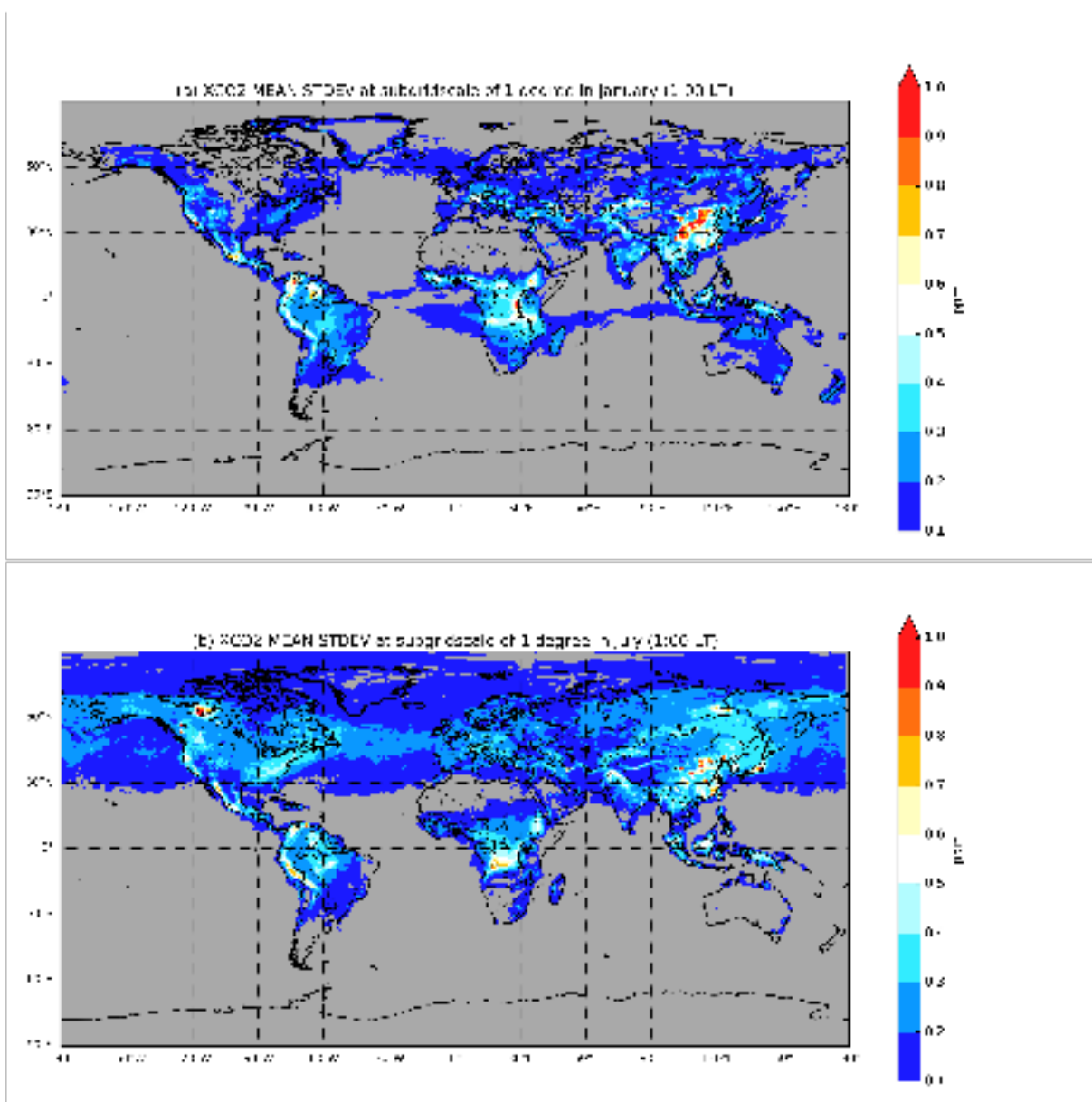
Figure 14. Monthly mean XCO 2 small-scale variability ( \sigma ) within 1 degree x 1 degree grid boxes [ppm] at 1:00 local time in (a) January and (b) July. Grey shading denotes \sigma < 0.1 .
