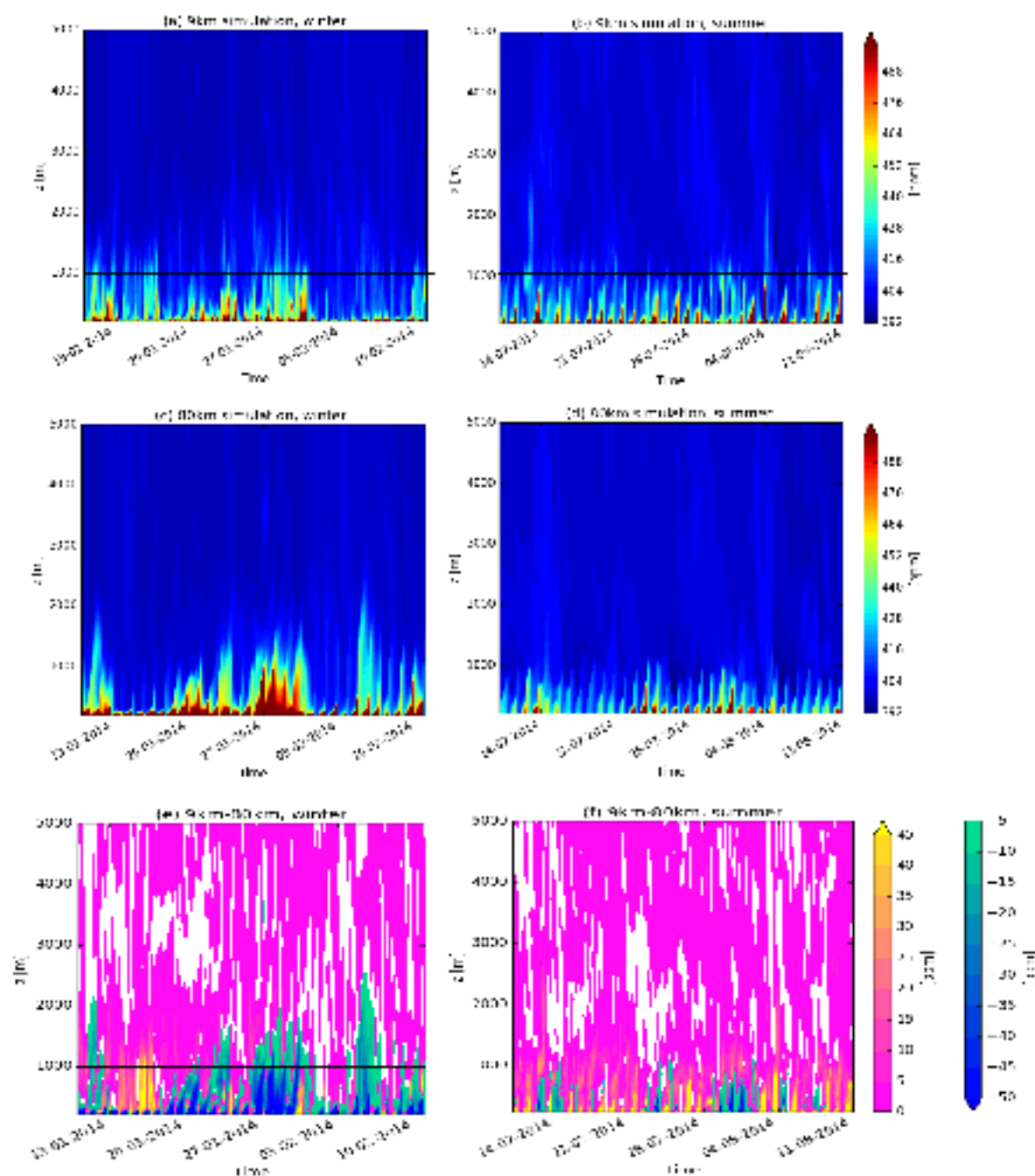
Figure S12. Modelled atmospheric CO 2 profile [ppm] showing 137 model levels at Pasadena from the 9-km resolution simulation and the 80-km resolution simulation. The horizontal black line shows the level approximately corresponding to 1000 m above the surface. In winter, the high CO 2 values are trapped below 1000 m in the boundary layer, except for certain synoptic episodes where boundary layer is ventilated as seen by high values (larger than 420 ppm) crossing the 1000 m line. While in summer the sea breeze circulation ventilates the boundary layer on a daily basis.
