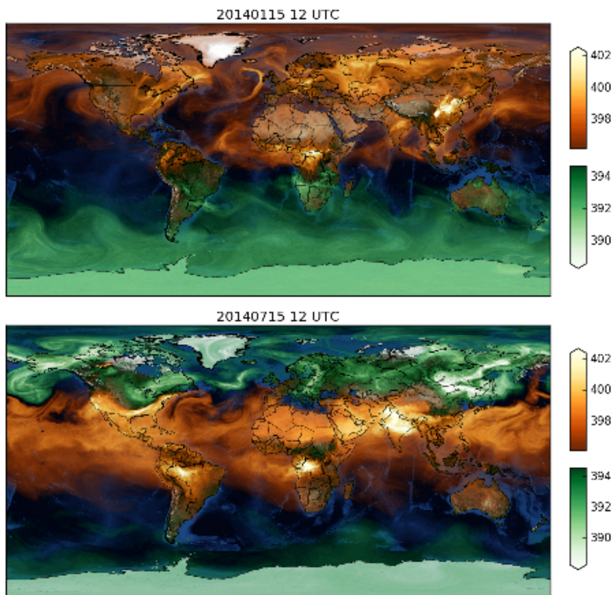
Figure 1. Snapshots of averaged-column \text{CO}_2 ( \text{XCO}_2 ) [ppm] above (in reds) and below (in greens) the global mean on 15 January (upper panel) and 15 July (lower panel) at 12 UTC from the Copernicus Atmosphere Monitoring Service global \text{CO}_2 forecast at high horizontal resolution (~ 9 km) .
