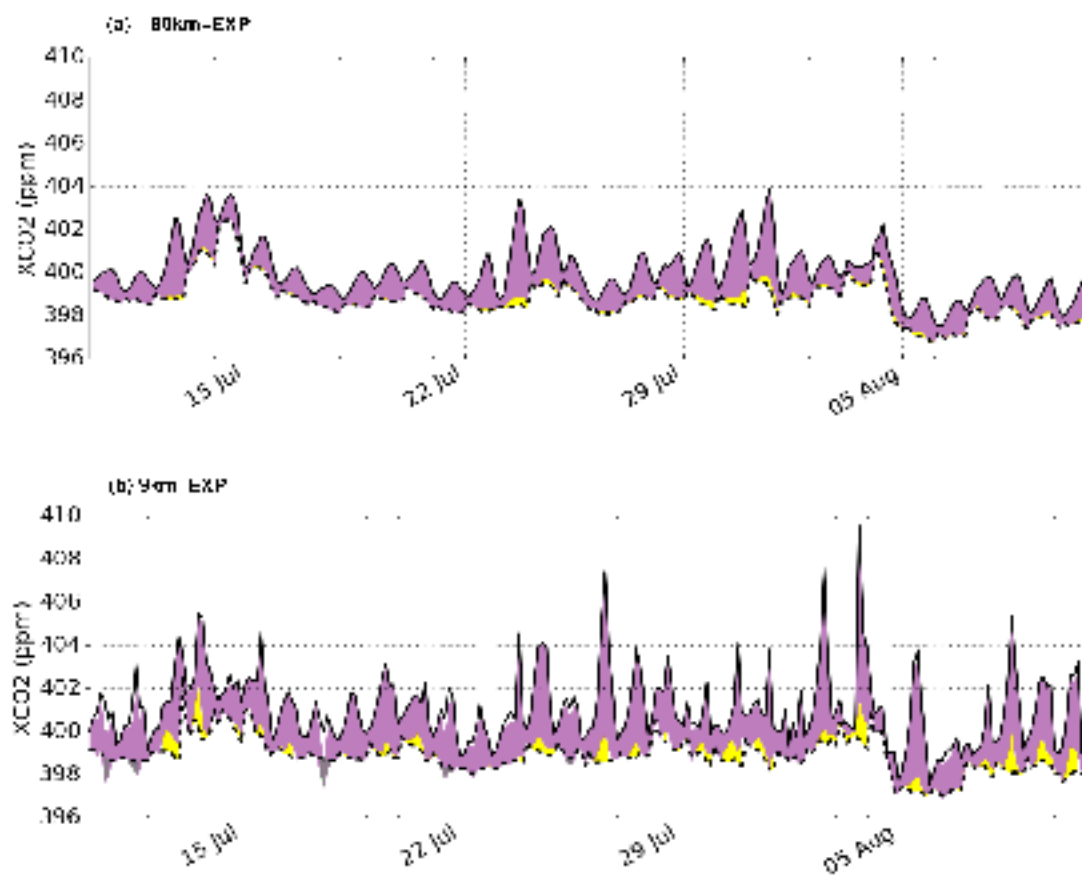
Figure S11. Same as Fig. 77 in July.
