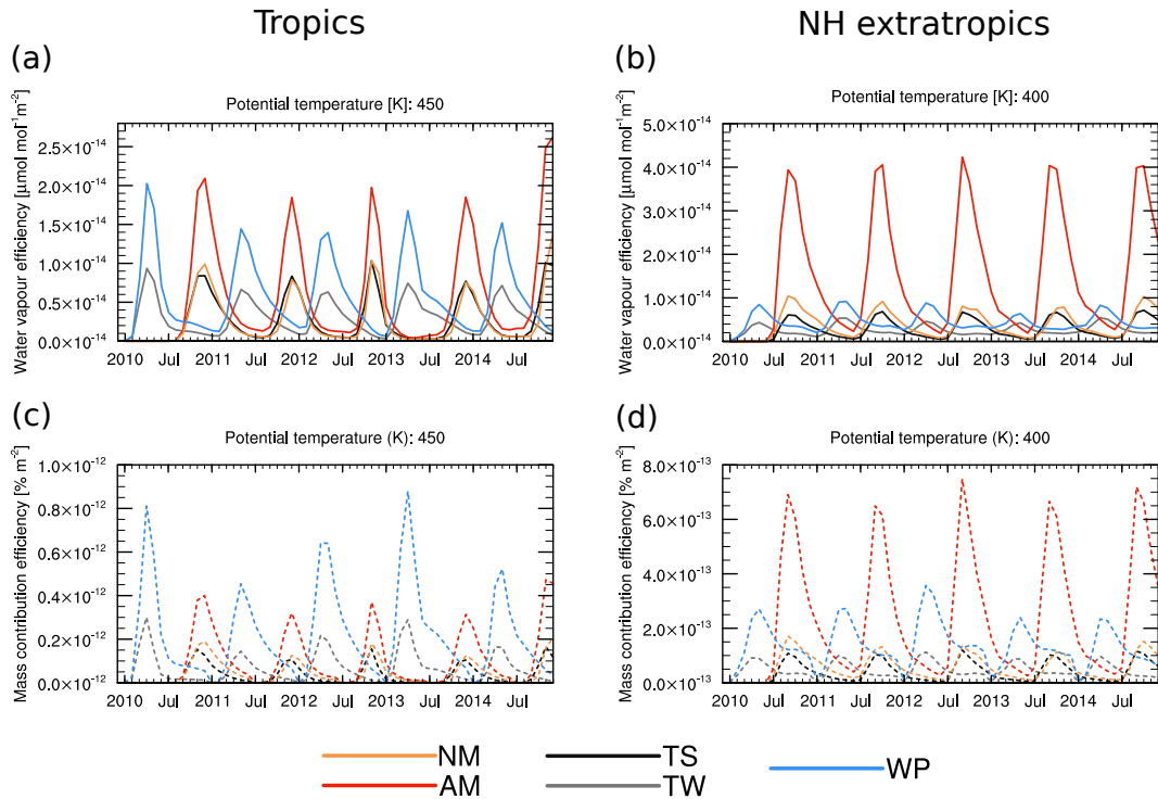
Figure 12. Time series of the H 2 O mean mixing ratios efficiency from the different source regions (all in \mu\text{mol mol}^{-1} \text{m}^{-2} ) (a) averaged over the region 10^\circ\text{S} – 10^\circ\text{N} at 450 K and (b) averaged over the region 50^\circ – 70^\circ\text{N} at 400 K. The colour coding of the source region is as follows: TS (black), TW (grey), WP (light blue), AM (red) and NM (orange). (c) and (d) as in (a) and (b) but for the mass contribution efficiency (in \% \text{m}^{-2} ). Multiplication of the efficiencies with the size of the respective source regions yields the contributions as shown in Figs. 6b and 7b.
