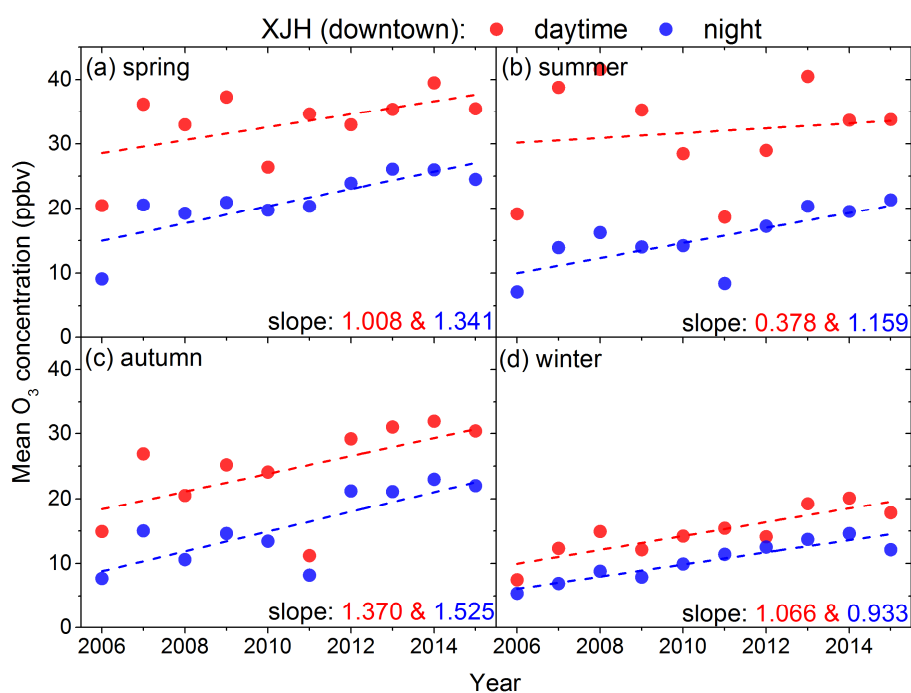
Fig.7 The variability of daytime and night O 3 concentration during 2006 to 2015 at XJH in (a) spring, (b) summer, (c) autumn, (d) winter respectively.
