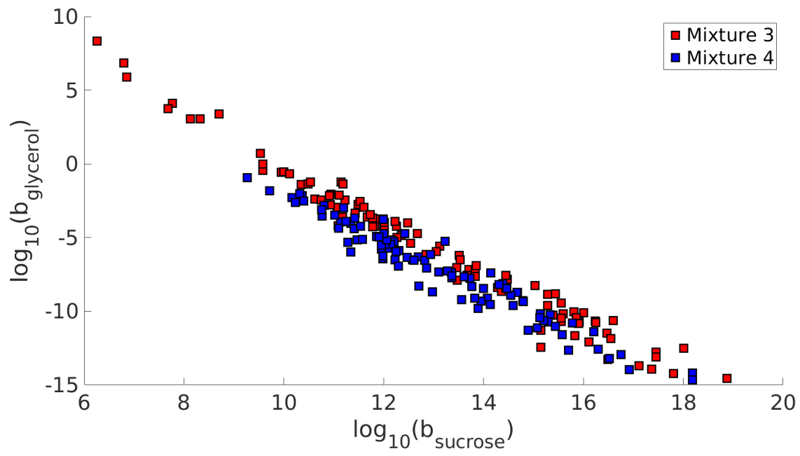
Figure S9: The correlation of estimated b -parameters for sucrose and glycerol in mixtures 3 and 4.
