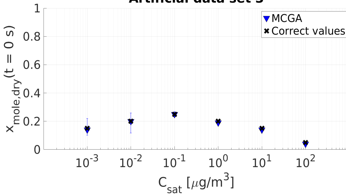
Figure 4: Parameter estimates for artificial data set 3; dry particle mole fraction at the start of the evaporation of six model compounds with predefined saturation concentration were optimized to match the data. Blue triangles show the MCGA estimates and black crosses the correct values. The whiskers show the 10th and 90th percentiles of the estimated variable distributions.
