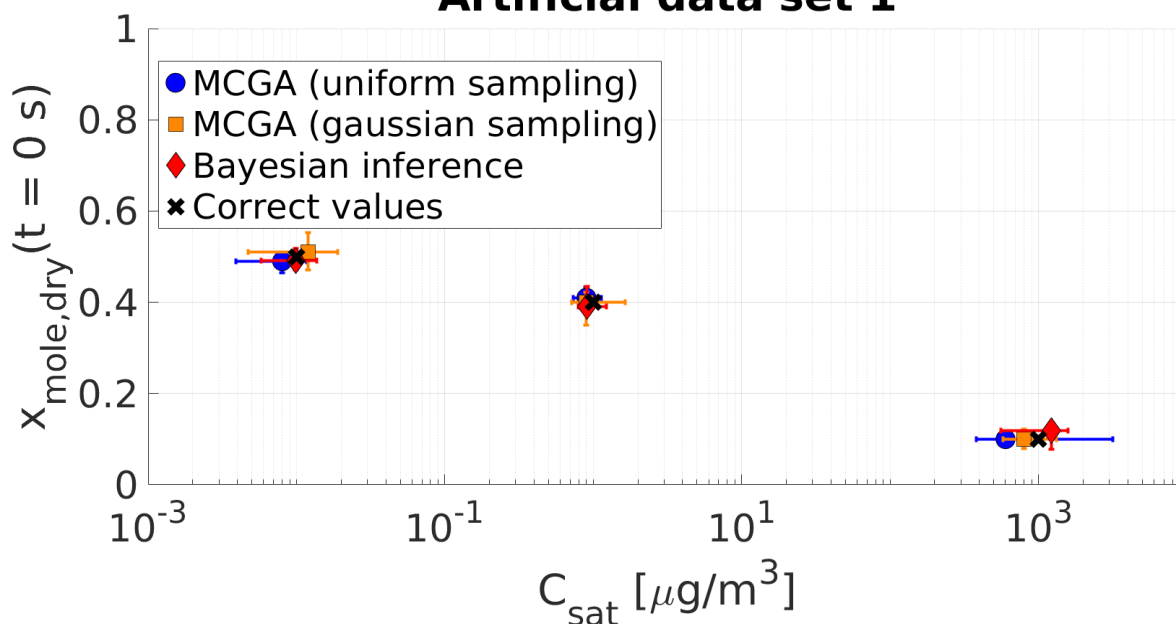
Figure 2: a) Parameter estimates from the three different optimization methods applied to artificial data set 1. Shown are MCGA with uniform sampling (blue circles), MCGA with sampling distributions similar to the Bayesian inference (Gaussian sampling, yellow squares) and Bayesian inference (red diamonds). The markers show the modes of the estimated variable distributions for MCGA methods and the maximum a posteriori estimate of the fitting variable distributions for the Bayesian inference. The whiskers show the 10 th and 90 th percentiles of the variable distributions for the MCGA methods and 90% credible interval for the Bayesian inference. b) The artificial data points which are the target of the optimization process and ten best fit simulations calculated with the LLEVAP model using the estimates from the MCGA optimization with uniform sampling.
