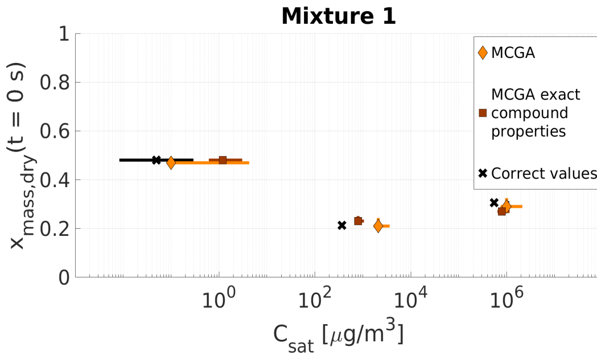
Figure 7: a) Parameter estimates for particles generated from mixture 1. Dry particle mass fraction at the start of the evaporation of three compounds and their saturation concentrations were optimized to match the evaporation data. Orange diamonds show the MCGA estimates calculated by assuming equal molar mass and particle phase density for all compounds and brown squares show the MCGA estimates calculated by setting the molar mass and particle phase density to their literature values. Black crosses show the literature values. The whiskers of the estimates show the 10th and 90th percentiles of the estimated variable distributions and the whiskers show the range of literature values (see Table 4 for references). b) The measured evaporation curve which is the target of the optimization process and ten best fit simulated evaporation curves calculated with the LLEVAP model using the estimates from optimization.
