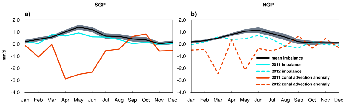
Fig. 1. Figure 1. The annual cycle of the moisture imbalance for the numerically calculated moisture tendencies (MFC(calculated)-(P-E)) averaged over the US a) SGP and b) NGP for the 1979-2018 climatology(soli
