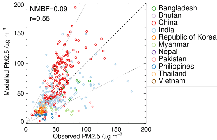
Figure 1. Simulated and measured annual mean surface PM 2.5 concentrations across South and East Asia. Observation data is from the World Health Organization database, 2016 & 2018. (a) Map of the simulated surface distribution of annual mean PM 2.5 for 2014 (underlying colours); overlying circles show measured annual mean PM 2.5 concentrations for available years (2009-2016). Regions in grey are outside the model domain. (b) Simulated versus measured annual mean PM 2.5 concentrations. Circles show measured annual mean PM 2.5 concentrations for the year 2014; diamonds show measured annual mean PM 2.5 concentrations for years other than 2014. All simulated annual mean PM 2.5 concentrations are for the year 2014. The normalised mean bias factor (NMBF; Yu et al., 2006) and Pearson's correlation coefficient (r) between simulated and measured values are displayed in the top left corner.
