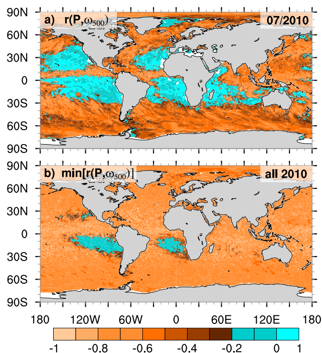
Figure 3. Maps of temporal correlation r(P, \omega_{500}) for each ERA5 gridbox for a) July 2010 and b) the minimal monthly correlation for the year 2010. Blue colored areas are weakly or positively correlated and are excluded from further analysis ( r > -0.2 ; Emori and Brown, 2005).
