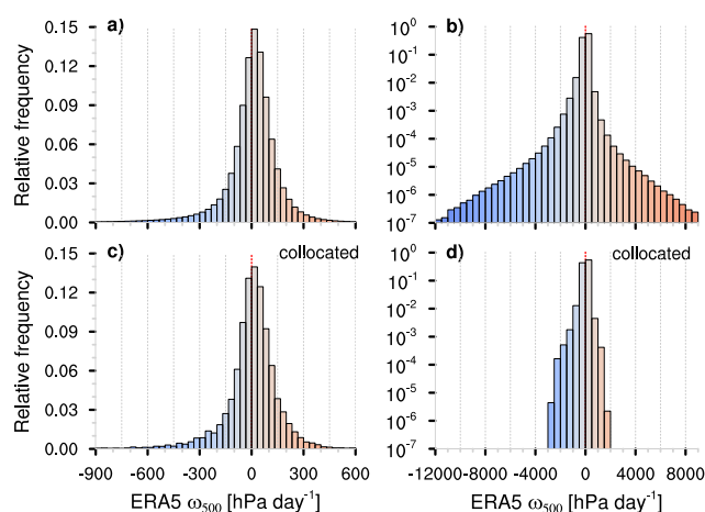
Figure 4. Histograms of relative frequency for \omega_{500} (blue: rising; red: subsiding motion) of (a),(b) all ERA5 gridboxes and (c),(d) for OceanRAIN–ERA5 collocated ERA5 gridboxes with (a),(c) linear ordinate and (b),(d) logarithmic ordinate for strong motion.
