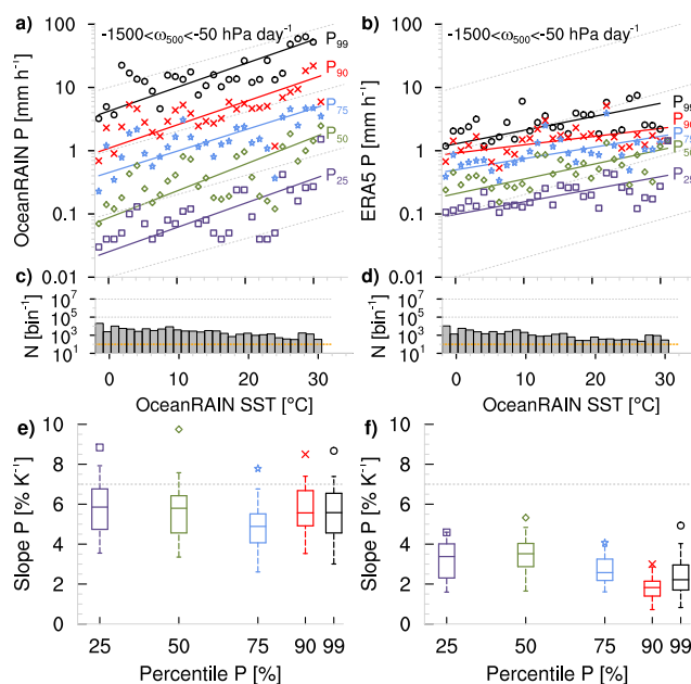
Figure 5. As Fig. 2 but for all OceanRAIN–ERA5 matched timesteps for (a),(c),(e) OceanRAIN and for (b),(d),(f) ERA5, both for rising motion ( -1500 < \omega_{500} < -50 \text{ hPa day}^{-1} ) and excluding regions of r(P, \omega_{500}) > -0.2 from Fig. 3.
