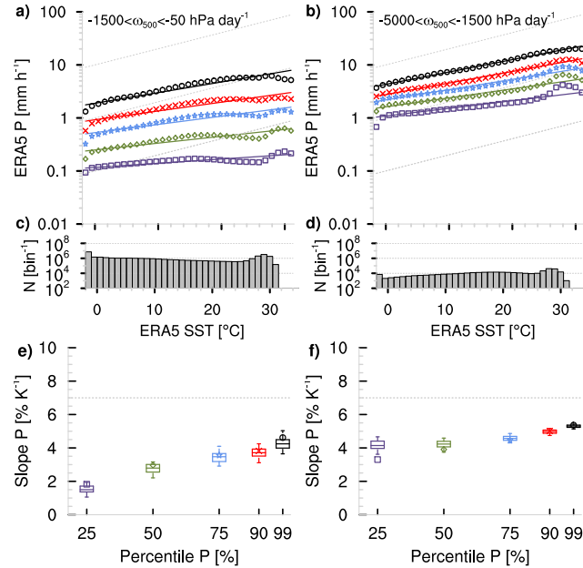
Figure 6. As Fig. 5 but for complete ERA5 period. Panels (a),(c),(e) are constrained by -1500 < \omega_{500} < -50 hPa \text{day}^{-1} and (b),(d),(f) by -5000 < \omega_{500} < -1500 hPa \text{day}^{-1} .
