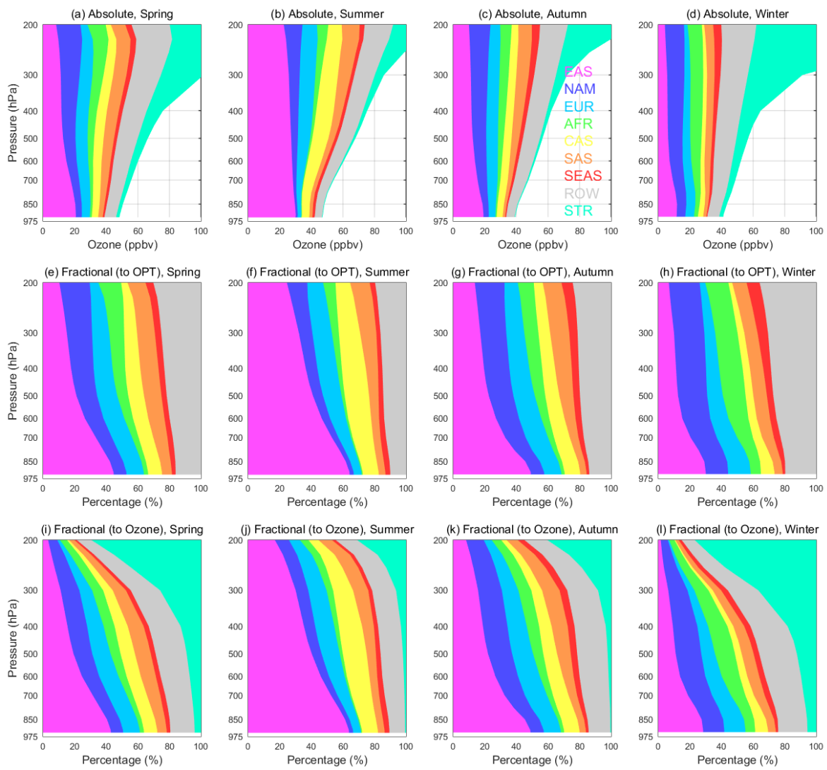
Figure 9. (a-d) Vertical variations of ozone (in ppbv) from native and foreign sources over East Asia by season. (e-h) The same as (a-d), but in terms of the fractional contributions (in %) to ozone produced in the troposphere (OPT). (i-l) The same as (a-d) but in terms of the fractional contributions (in %) to ozone over East Asia. All values are the means over East Asia at each altitude in 2005. The abbreviations are for East Asia (EAS), North America (NAM), Europe (EUR), Africa (AFR), central Asia (CAS), South Asia (SAS), Southeast Asia (SEAS), the rest of the world (ROW), and the stratosphere (STR).
