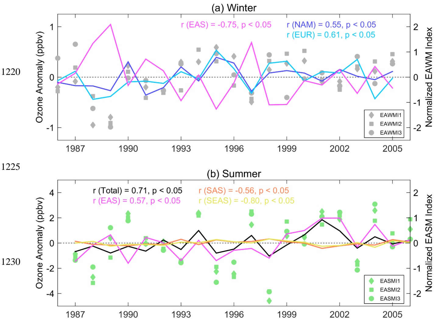
Figure 12. Interannual variations of the anomalies of foreign ozone (in ppbv, left y-axis) from various regions at the East Asian surface driven by meteorology (Tagged-Ozone) in winter (a) and summer (b). The values are averaged over 110-145 °E, 22-46 °N in winter and 95-130 °E, 22-46 °N in summer, where the correlations are the most significant. The correlation coefficients calculated with the three sets of monsoon indices in each season are averaged. The abbreviations are for East Asia (EAS), North America (NAM), Europe (EUR), South Asia (SAS), and Southeast Asia (SEAS).
