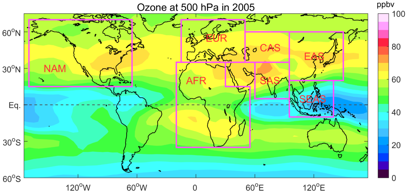
Figure 1. Annual mean ozone concentrations in the middle troposphere (500 hPa) in 2005 from GEOS- 980 Chem simulations. The purple boxed areas define seven regions, plus the rest of the world (ROW, all regions except the boxed regions). The seven regions include East Asia (EAS, 95 °E-150 °E, 20 °N-60 °N), North America (NAM, 170 °W-65 °W, 15 °N-70 °N), Europe (EUR, 15 °W-50 °E, 35 °N-70 °N), Africa (AFR, 20 °W-30 °E, 0-35 °N and 20 °W-55 °E, 35 °S-0), central Asia (CAS, 50 °E-95 °E, 35 °N-60 °N), South Asia (SAS, 60 °E-95 °E, 5 °N-35 °N), and Southeast Asia (SEAS, 95 °E-140 °E, 10 °S-20 °N).
