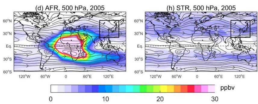
Figure 8. Horizontal distributions of ozone produced in different regions in the middle troposphere (500 hPa) averaged in 2005. The boxed area indicates East Asia. The abbreviations are for (a) East Asia (EAS), (b) North America (NAM), (c) Europe (EUR), (d) Africa (AFR), (e) central Asia (CAS), (f) South Asia (SAS), (g) Southeast Asia (SEAS), and (h) the stratosphere (STR).
