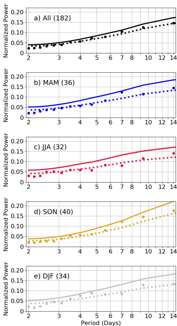
Figure 13: Normalized power spectra for 2-14 day cycles for the total aerosol number concentrations from the CPC for the entire period (a) and by season (b-e). The dots represent power associated with the data. The dashed lines represent an estimate of the red noise power spectrum for each data set, and the solid lines represent the 99% significance testing level, as described in the text. The values in the parentheses are the number of 28-day data chunks used in this analysis.
