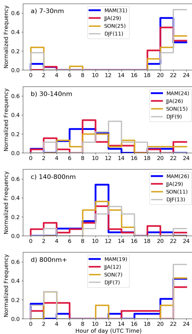
Figure 10: Normalized frequency of the daily time of peak concentrations associated with the 24-hour cycle in the different modes of the aerosol volume size distribution. (a-d) represent V_{7-30\text{nm}} , V_{30-140\text{nm}} , V_{140-800\text{nm}} , and V_{800\text{nm}+} , respectively. The description of the figure is the same as in Figure 6.
