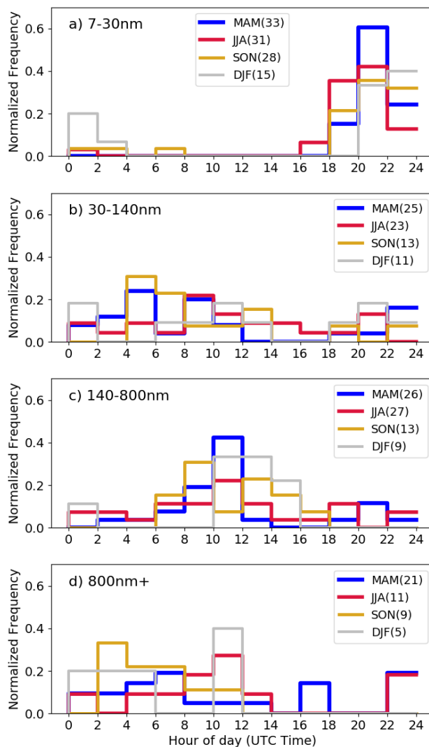
Figure 8: Normalized frequency of the daily time of peak concentrations associated with the 24-hour cycle in the different modes of the aerosol number size distribution. (a-d) represent N_{7-30\text{nm}} , N_{30-140\text{nm}} , N_{140-800\text{nm}} , and N_{800\text{nm}+} , respectively. The description of the figure is the same as in Figure 6.
