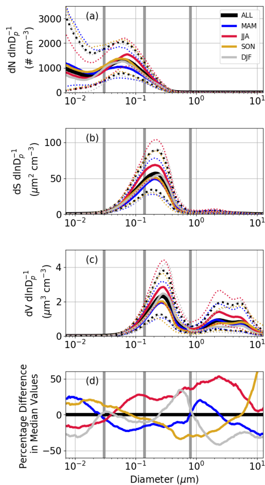
5 Figure 2: Aerosol size distributions for the entire time period and by season. (a) represents the number size distributions ( \# \text{ cm}^{-3} ), (b) represents the surface area size distributions ( \mu\text{m}^2 \text{ cm}^{-3} ), and (c) represents the volume size distributions ( \mu\text{m}^3 \text{ cm}^{-3} ). The solid colored lines depict the median values, and the dotted lines depict the 25 th and 75 th percentiles. (d) represents the percentage difference in the median size distributions for each season with respect to the entire period (ALL). The vertical grey lines demarcate the four separate regions of the size distribution that were used for further analyses in this study.
