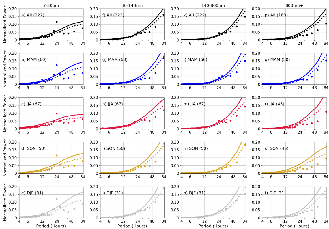
Figure 7: Normalized power spectra for N_{7-30\text{nm}} , N_{30-140\text{nm}} , N_{140-800\text{nm}} and N_{800\text{nm}+} for the entire period and by season. The descriptions of the symbols used are the same as in Figure 5.
