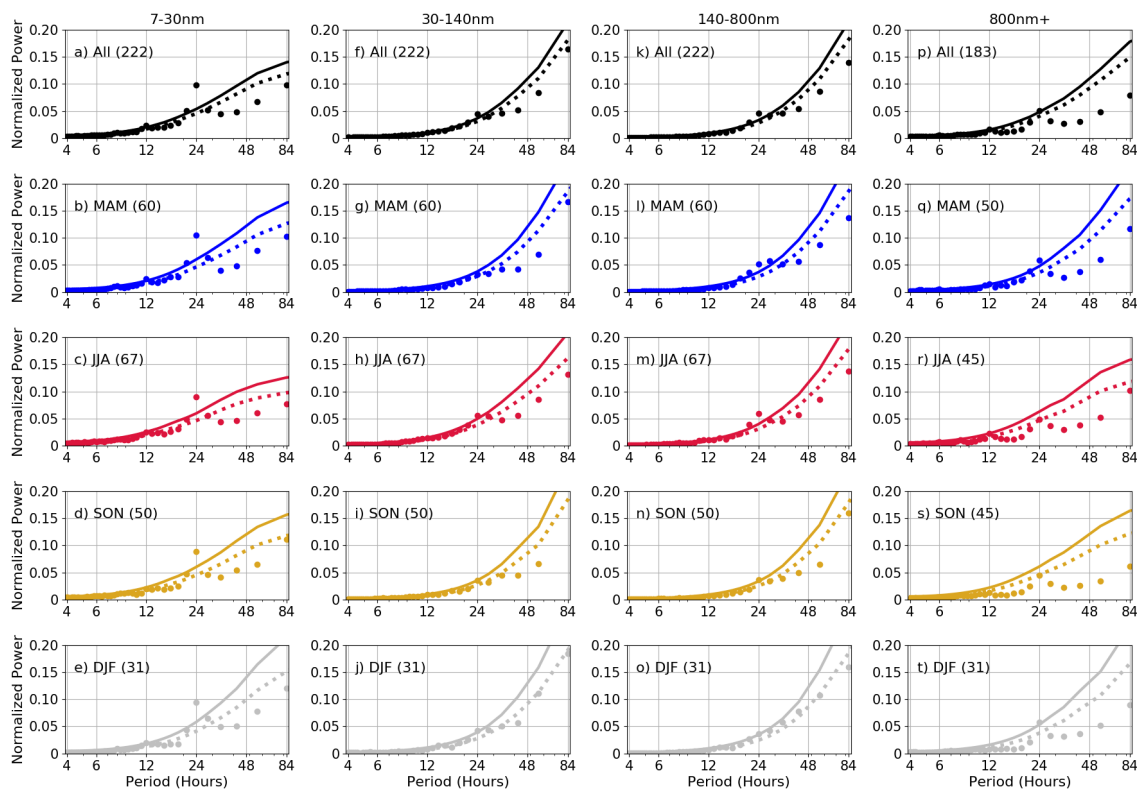
Figure 9: Normalized power spectra for V_{7-30\text{nm}} , V_{30-140\text{nm}} , V_{140-800\text{nm}} , and V_{800\text{nm}+} for the entire period and by season. The descriptions of the symbols used are the same as in Figure 5.
