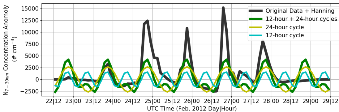
Figure 12: N_{7-30nm} for the weekly data chunk that had the highest power associated with the 12-hour cycle (22–29 February 2012). The aerosol data are shown as a concentration anomaly from the seasonal mean (black). The anomaly data are broken down into the 12-hour cycle component (cyan), the 24-hour cycle component (yellow), and the combination of the 12- and 24-hour cycles (green), as computed by the power spectral analysis.
