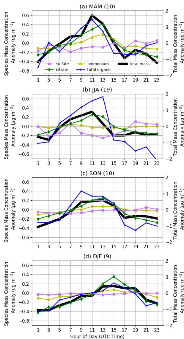
Figure 11: Diurnal cycle of aerosol mass concentration anomalies for sulfate, nitrate, ammonium, and organic aerosol species (left axis) and total mass concentrations (right axis) from the ACSM. The data were separated into seasons (a-d) and only included the weekly time periods where the power associated with the 24-hour cycle in integrated volume between 140 and 800nm ( V_{140-800nm} ) was greater than that of red noise. The number of these weekly time periods is shown in the parenthesis in the panel titles.
