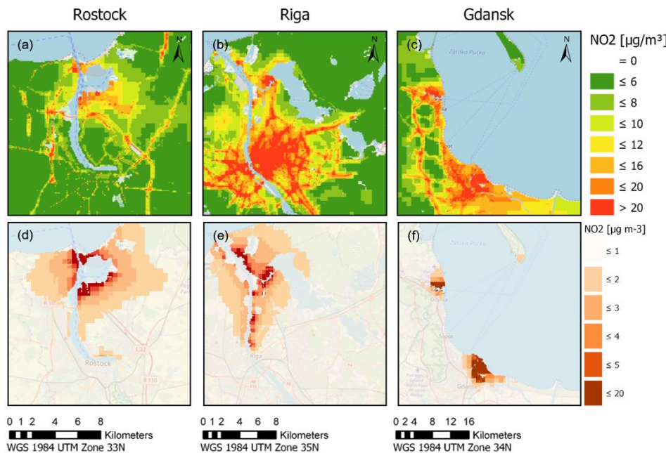
Figure 9: \text{NO}_2 annual mean concentrations in Rostock (a), Riga (b) and Gdansk-Gdynia (c), and contribution of local shipping to annual mean \text{NO}_2 concentration in Rostock (d), Riga (e) and Gdansk-Gdynia (f).
