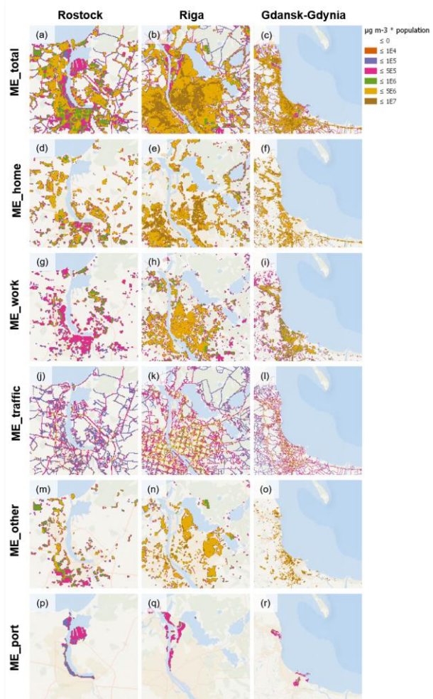
Figure 11: Exposure to NO 2 from all sources in all microenvironments and urban domains.
