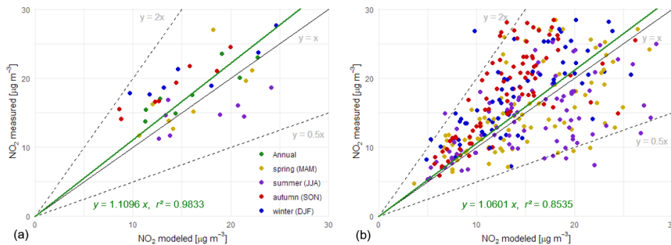
Figure 8: Modelled versus measured \text{NO}_2 concentrations at all available measurement stations in the Gdansk-Gdynia research domain. (a) Shows annual station averages with each dot indicating one station, while (b) shows daily averages with each dot indicating an average of all stations. For (a) and (b) the colours display seasons.
