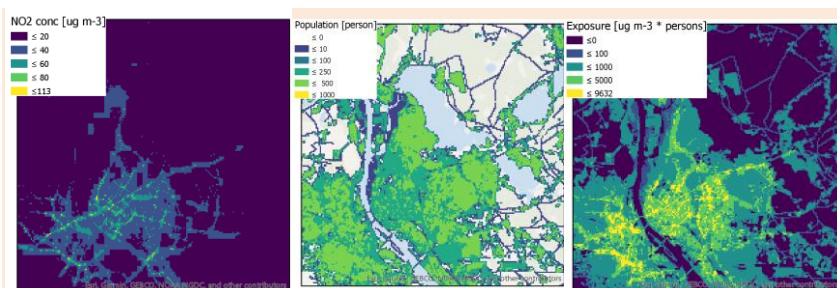
Figure 2: The predicted ambient air concentrations of NO 2 (ug m -3 ), the density of population (persons) and the average exposure of the population to NO 2 concentrations (ug m -3 * persons), evaluated for the afternoon time period, as an average value in March 2012 in Riga. The grid size is 100m x 100 m, the size of the depicted area is 20km x 20 km.
