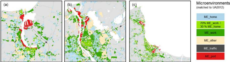
Figure 5: Urban Atlas Land use classifications, aggregated by colours according to microenvironment mapping presented in Table 2 for Rostock (a), Riga (b) and Gdansk-Gdynia (c).
