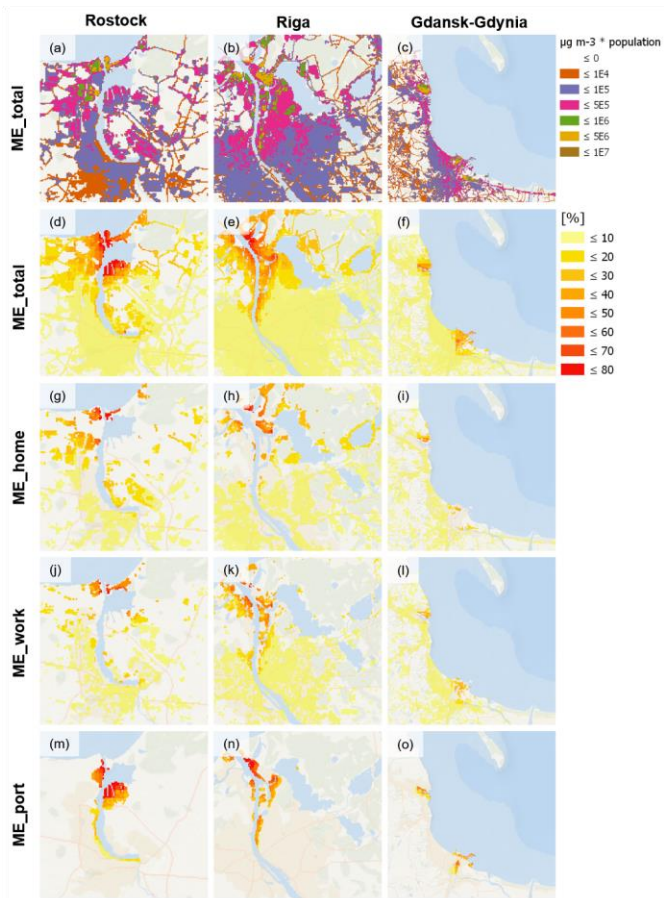
Figure 12: Exposure to NO 2 from local shipping as relative contribution to all microenvironments (d-f, ME_home (g-i), ME_work (j-l) and ME_port (m-o) of absolute contribution from shipping related NO 2 exposure (a-c).
