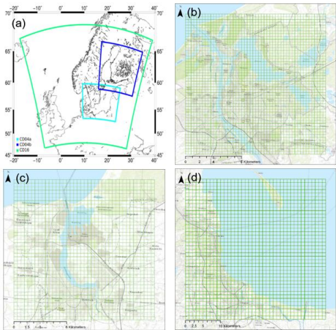
Figure 4: (a) Regional CTM simulation domains, which have been used to drive the local-scale EPISODE-CityChem simulation for the urban domains in (b) Riga and (c) Rostock with 400 m resolution for 20 × 20 km 2 and 16 × 16 km 2 extent, and (d) Gdansk-Gdynia with 1000 m resolution and 40 × 40 km 2 extent.
