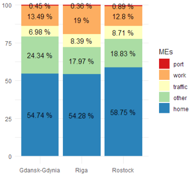
Figure 10: Relative distribution of total exposure in different microenvironments based on total annual averaged grid mean exposure to NO 2 in Rostock, Riga and Gdansk-Gdynia.
