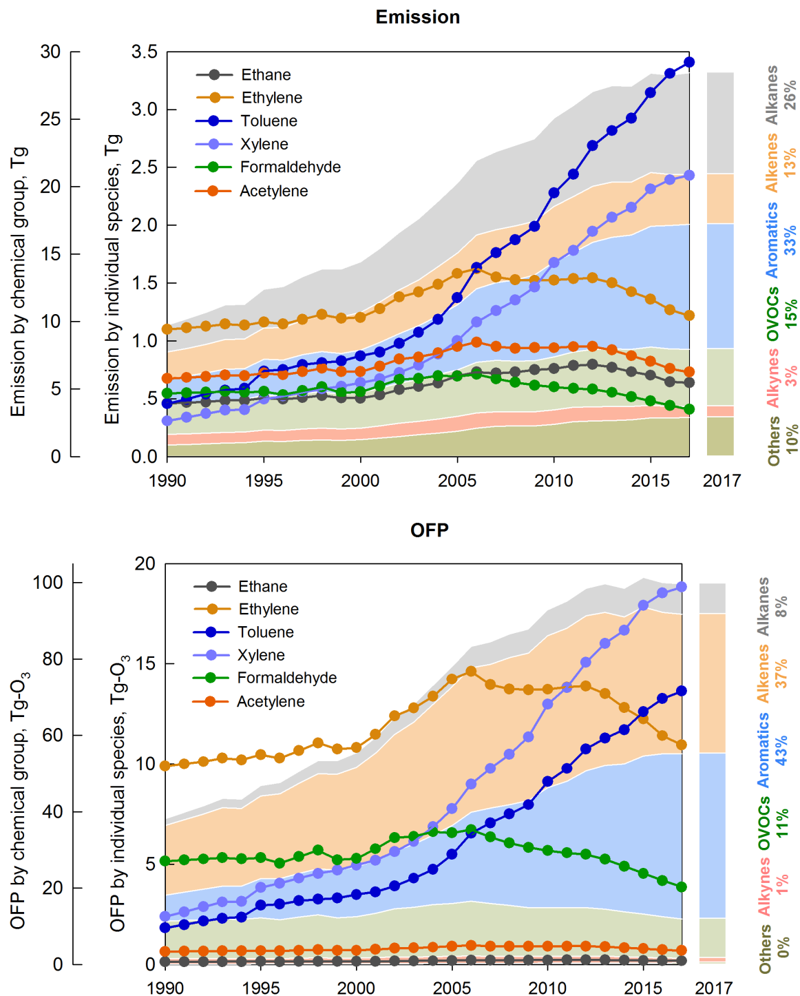
Figure 4. Emission trends for key chemical species (ethane, ethylene, toluene, xylene, formaldehyde, acetylene) during 1990-2017.
