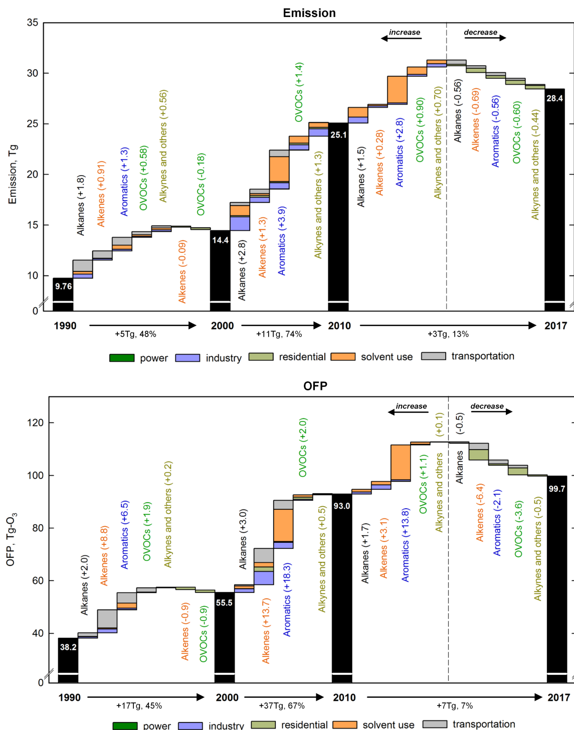
Figure 5. Decomposed changes by chemical group and sector for emission and OFP from 1990 to 2017.
