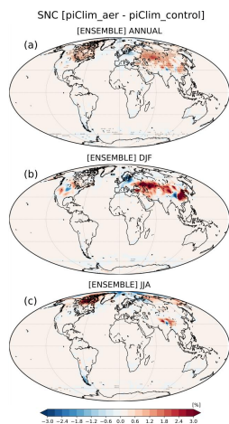
Figure IV: Differences between piClim-aer and piClim-control in snow cover fraction over land for the ensemble of 7 models on an annual basis (a), for DJF (b) and for JJA (c). The dot shading indicates areas in which the differences are statistically significant at the 95% confidence level.
