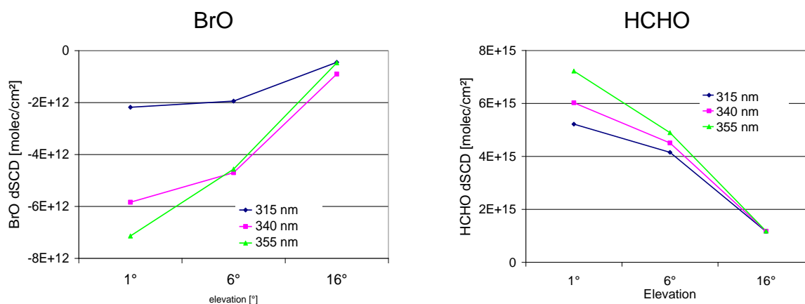
Fig. S13 Dependence of the simulated trace gas dSCDs for BrO ( left ) and HCHO ( right ) on the elevation angle for different wavelengths used for the AMF calculations.
