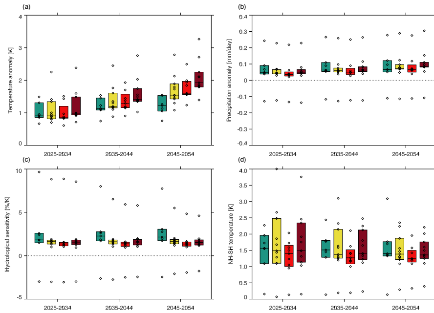
Figure 7. Global-mean annual-mean anomalies in (a): near-surface temperature [K]; (b): precipitation [mm day -1 ]; (c): hydrological sensitivity [% K -1 ] relative to 1980-2014. (d): Annual-mean anomalies in interhemispheric temperature gradient [K] relative to 1980-2014. Coloured bars show the interquartile range, and the horizontal bar within this shows the median. Diamonds show values from each model listed in Table 1 as having data availability for a given SSP. Where multiple ensemble members are available the model mean is used.
