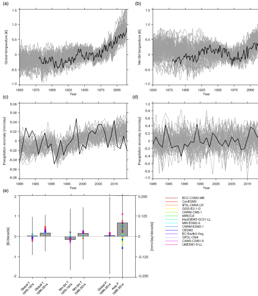
Figure 4. (a): Global-mean annual-mean temperature anomaly relative to 1951-1980 from CMIP6 (grey lines show individual members) and GISTEMP (black). (b): Annual-mean interhemispheric temperature gradient anomaly relative to 1951-1980 from CMIP6 (grey) and GISTEMP. (c): Annual-mean global-mean precipitation anomaly relative to 1980-2014 from CMIP6 (grey) and GPCP (black). (d): JJA mean Asia-mean precipitation anomaly relative to 1980-2014 from CMIP6 (grey) and GPCP (black). Asia is the region from 5-47.5^{\circ}\text{N} and 67.5-145^{\circ}\text{E} . (e): linear trends in annual-mean global-mean temperature and JJA-mean interhemispheric temperature gradient from CMIP6 (coloured diamonds) and GISTEMP (grey bars) for 1950-1974 and 1980-2014, and linear trends in annual-mean global-mean precipitation and JJA-mean Asia-mean precipitation for 1980-2014 (grey bars are GPCP). Error bars show plus or minus one standard error on the observed trend. Note that for Asian precipitation this extends beyond the range of the plot, and is an order of magnitude larger than the trend.
