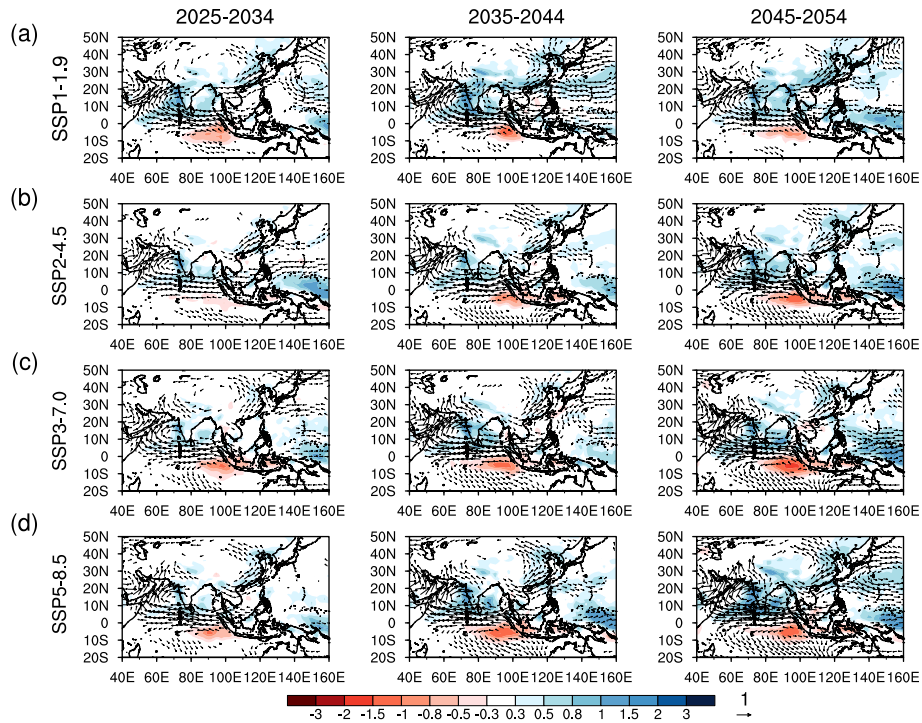
Figure 11. CMIP6-mean JJA-mean precipitation [mm day -1 ] and 850 hPa wind anomalies [m s -1 ] for 2025-2034, 2035-2044, and 2045-2054 vs. 1980-2014 from (a): SSP1-1.9; (b): SSP2-4.5; (c): SSP3-7.0; and (d): SSP5-8.5.
