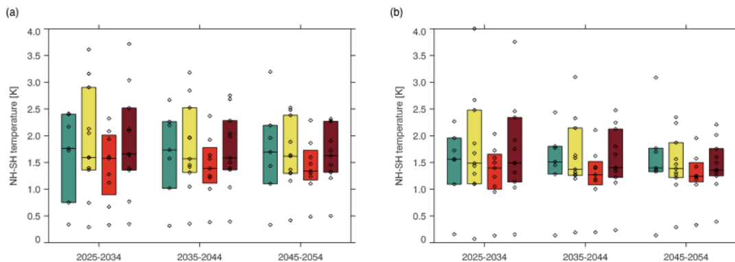
Fig. 2. (a): Annual-mean interhemispheric temperature gradient anomalies relative to 1980-2014 from SSP1-1.9, 2-4.5, 3-7.0, and 5-8.5 (as shown in the revised manuscript). (b): As for panel (a), but for JJA
