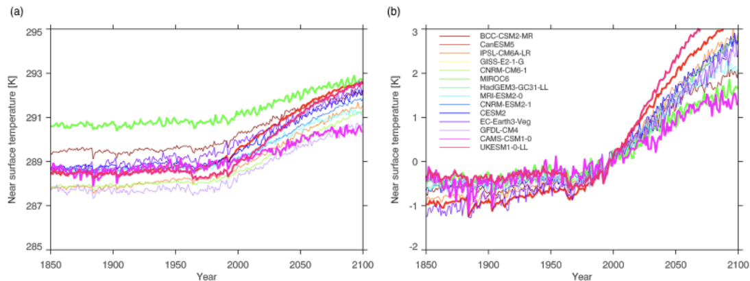
Fig. 1. (a): Annual-mean global-mean temperature time series for the historical simulation and SSP2-4.5. (b): The same data as shown in panel (a), but presented as an anomaly relative to 1980-2014.
