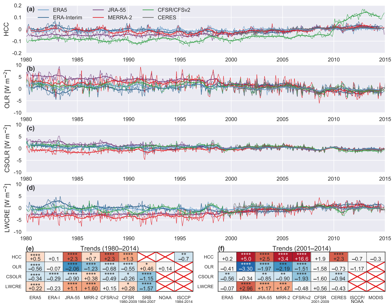
Figure 14. Time series of deseasonalized anomalies in monthly mean (a) HCC, (b) all-sky OLR, (c) clear-sky OLR, and (d) LWCRE averaged over the inner tropics (10°S–10°N) for 1980–2014 based on ERA5 (cyan), ERA-Interim (blue), JRA-55 (purple), MERRA-2 (red), and CFSR/CFSv2 (green). Observational analyses from CERES SYN1Deg (a; March 2000–December 2014) and CERES EBAF (b–d; March 2000–December 2014) are shown for context. Anomalies are calculated relative to the mean annual cycle during 2001–2014. Thick lines show time series after applying a 12-month uniformly-weighted rolling mean. Trends are listed for annual-mean anomalies during the (e) 1980–2014 and (f) 2001–2014 periods in percentage points per decade for HCC and units of \text{W m}^{-2} per decade for OLR, clear-sky OLR, and LWCRE. Stars indicate statistical significance at the 90% (*), 95% (**), 99% (***), and 99.5% (****) confidence levels. Light grey shading indicates that the 90% confidence interval of the Theil–Sen slope (Sen, 1968) contains zero. Blue colours mark negative trends and red colours positive trends, with darker shades signifying larger trend magnitudes (0 to 1, 1 to 2, 2 to 3, and greater than 3).
