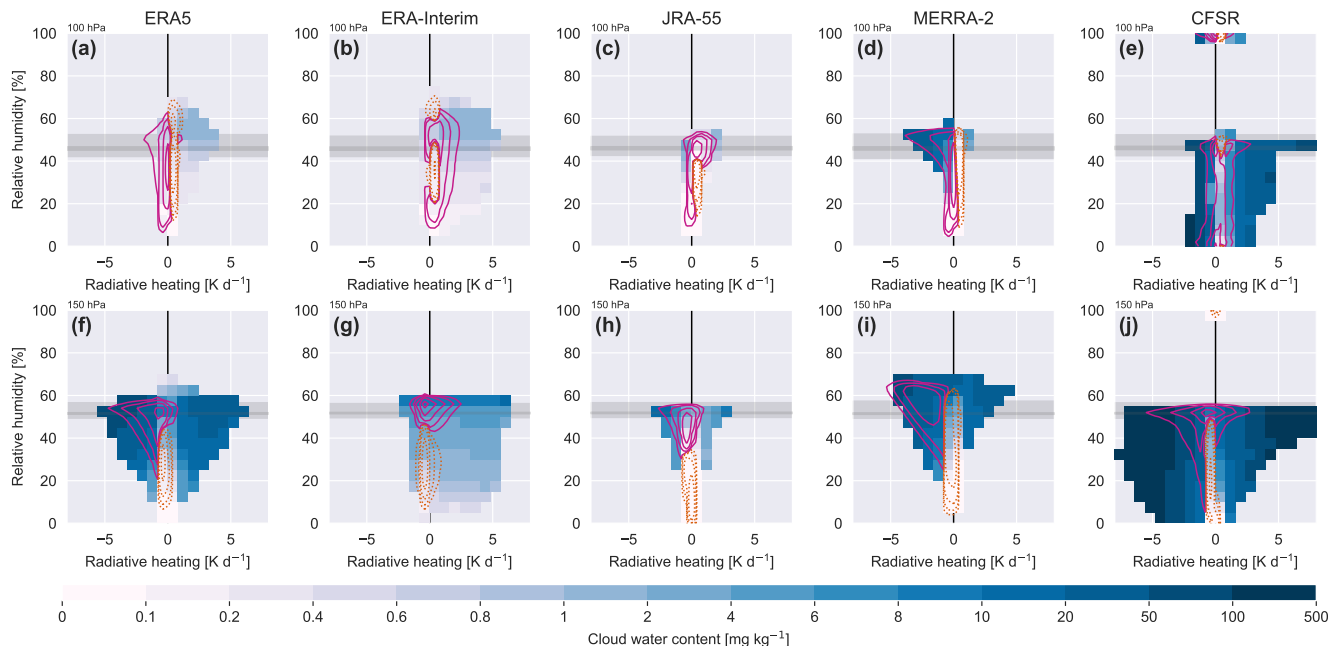
Figure 12. Composite distributions of daily-mean CWC as a function of radiative heating rate and grid-scale relative humidity (RH) in (a,f) ERA5, (b,g) ERA-Interim, (c,h) JRA-55, (d,i) MERRA-2, and (e,j) CFSR on the 100 hPa (upper row; a–e) and 150 hPa (lower row; f–j) isobaric surfaces. RH is calculated with respect to liquid water. Grey shaded regions in each panel mark ranges of ice saturation ratios ( e_i^*/e_l^* ) at these levels, with light shading marking the minimum and maximum and dark shading marking the interquartile range. Solid pink contours mark paired values of radiative heating and RH that are more commonly associated with cloudy conditions (Q4 of the daily-mean LWCRE) than with clear-sky conditions (Q1 of the LWCRE); dashed orange contours mark the opposite (values more commonly associated with Q1 than Q4). Composite mean CWCs are masked for bins containing fewer than 200 samples.
