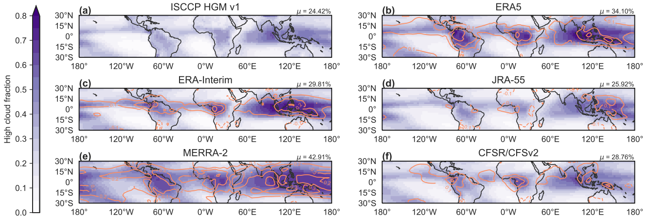
Figure 1. Climatological mean spatial distribution of high cloud cover (HCC) for (a) ISCCP HGM, (b) ERA5, (c) ERA-Interim, (d) JRA-55, (e) MERRA-2, and (f) CFSR/CFSv2 over 1984–2014. Differences relative to ISCCP HGM are shown for each reanalysis as orange contours (dashed for negative values) at intervals of 0.1. The area-weighted tropical mean (30°S–30°N) HCC based on each product is shown at the upper right corner of the corresponding panel.
