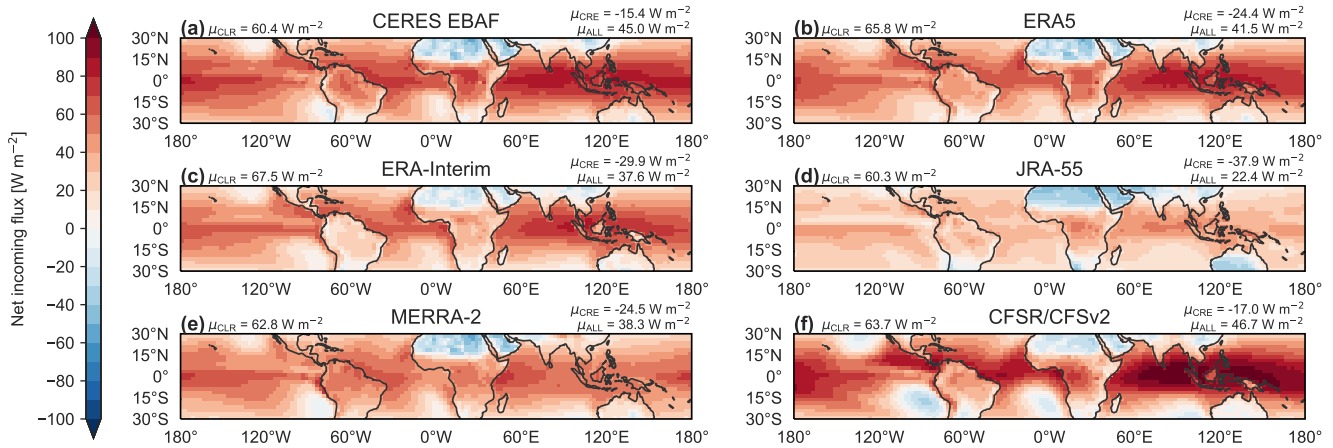
Figure 6. Climatological mean spatial distributions of all-sky net incoming radiation (ALL; shading) for (a) CERES EBAF, (b) ERA5, (c) ERA-Interim, (d) JRA-55, (e) MERRA-2, and (f) CFSR/CFSv2 during 2001–2014. Tropical mean ( 30^{\circ}\text{S} – 30^{\circ}\text{N} ) values of ALL and clear-sky net incoming radiation (CLR) based on each product are shown at the upper right and left corners, respectively, of the corresponding panel. Tropical mean values for the net cloud radiative effect ( \text{CRE} = \text{CLR} - \text{ALL} ) are listed above those for ALL.
