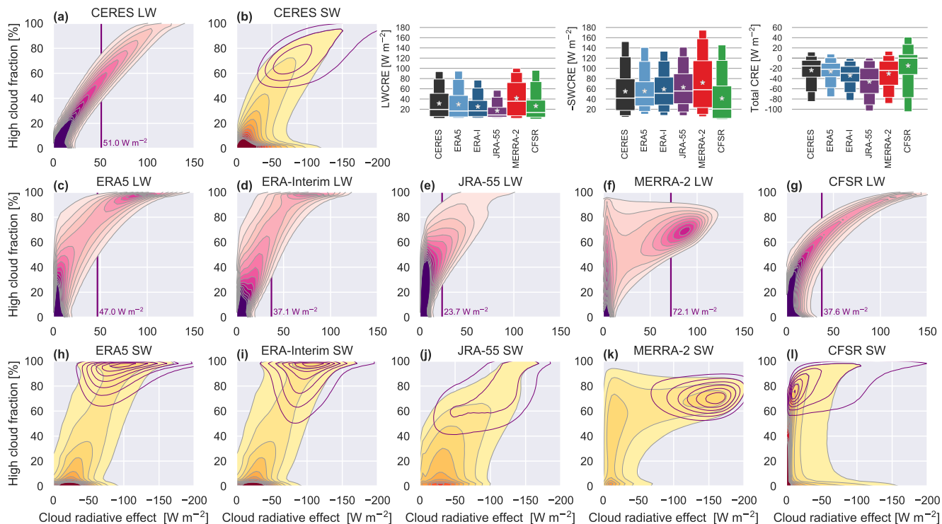
Figure 7. Joint distributions of daily-mean HCC against (a) LWCRE and (b) SWCRE based on CERES SYN1Deg using gridded data from 2001–2010. Corresponding joint distributions are shown for (c,h) ERA5, (d,i) ERA-Interim, (e,j) JRA-55, (f,k) MERRA-2, and (g,l) CFSR. The 75 th percentile of the LWCRE is marked in panels (a) and (c–g). Sub-distributions of HCC against SWCRE associated with the values of LWCRE that exceeded the corresponding 75 th percentile threshold are then shown as purple contours in panels (b) and (h–l). Distributions of the LWCRE, SWCRE, and total CRE are shown in the upper right, with SWCRE multiplied by -1 for convenience of presentation. The thickest boxes mark the interquartile ranges, with the medians marked as horizontal lines and the means marked as stars. The narrower extended boxes indicate the 5 th , 10 th , 90 th , and 95 th percentiles.
