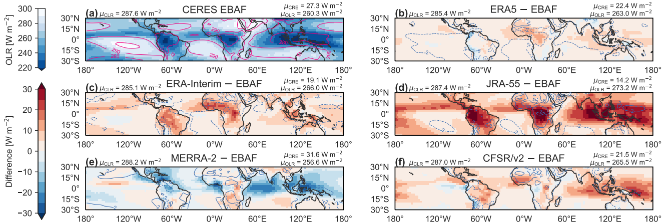
Figure 5. Climatological mean spatial distributions of all-sky outgoing longwave radiation (OLR; shading) and clear-sky outgoing longwave radiation (CLR; contours at intervals of 10 W m^{-2} ) for (a) CERES EBAF over 2001–2014. Differences relative to CERES EBAF for the same period are shown for (b) ERA5, (c) ERA-Interim, (d) JRA-55, (e) MERRA-2, and (f) CFSR/CFSv2. Contours in panels (c) through (f) cover the range within \pm 10 W m^{-2} at intervals of 4 W m^{-2} . Tropical mean ( 30^{\circ}S – 30^{\circ}N ) values of OLR and CLR based on each product are shown at the upper right and left corners, respectively, of the corresponding panel. Tropical mean values for the longwave cloud radiative effect ( LWCRE = CLR - OLR ) are listed above those for OLR.
