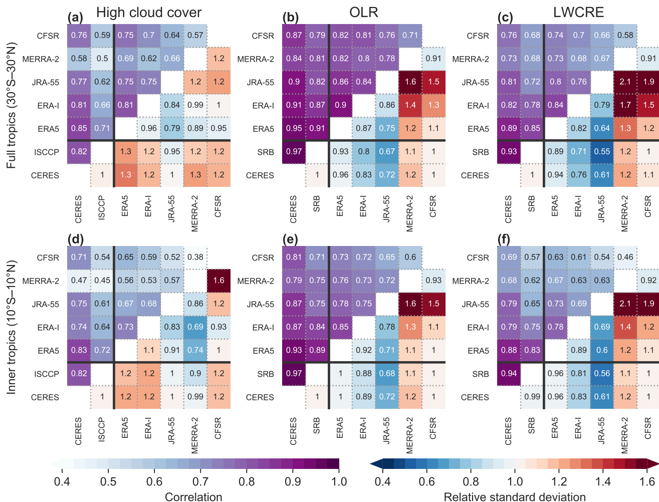
Figure 15. Metrics measuring agreement in monthly anomalies of (a,d) HCC, (b,e) OLR, and (c,f) the LWCRE among the reanalyses and observational data sets examined in this paper. The upper left triangle in each panel shows correlation coefficients between each pair of products, while the lower right triangle shows the standard deviation in the product marked on the horizontal axis relative to that in the product marked on the vertical axis. Both metrics are evaluated first for individual grid cells in the 2.5° common grid (see, e.g., Fig. 1) and then averaged. The upper row (a–c) shows results for the entire tropics (30°S–30°N), while the lower row (d–f) shows results for the inner tropics only (10°S–10°N). Solid black lines separate evaluations relative to the observational benchmarks based on CERES, ISCCP, and NASA-GEWEX SRB from those based on intercomparison of reanalysis products.
