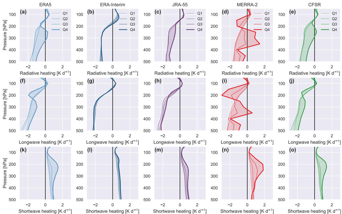
Figure 8. Composite mean profiles of daily-mean radiative heating rates as a function of pressure for the first through fourth quartiles (Q1–Q4) of LWCRE in the inner tropics ( 10^{\circ}\text{S} – 10^{\circ}\text{N} ; see also Fig. 7) based on (a) ERA5, (b) ERA-Interim, (c) JRA-55, (d) MERRA-2, and (e) CFSR during 2001–2010. Here Q1 refers to the bottom quartile (weak longwave CRE) and Q4 to the top quartile (strong longwave CRE). Total radiative heating rates (upper row; a–e) are separated into (f–j) longwave and (k–o) shortwave components in the lower two rows.
