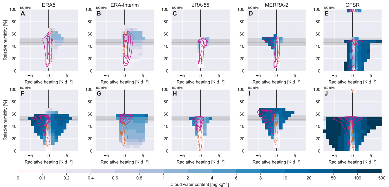
Figure 12. Composite distributions of daily-mean CWC as a function of radiative heating rate and grid-scale relative humidity (RH) in (A, F) ERA5, (B, G) ERA-Interim, (C, H) JRA-55, (D, I) MERRA-2, and (E, J) CFSR on the 100 hPa (upper row; A–E) and 150 hPa (lower row; F–J) isobaric surfaces. RH is calculated with respect to liquid water. Grey shaded regions in each panel mark ranges of ice saturation ratios ( e_i^*/e_l^* ) at these levels, with light shading marking the minimum and maximum and dark shading marking the interquartile range. Solid pink contours mark paired values of radiative heating and RH that are more commonly associated with cloudy conditions (Q4 of the daily-mean LWCRE) than with clear-sky conditions (Q1 of the LWCRE); dashed orange contours mark the opposite (values more commonly associated with Q1 than Q4). Composite mean CWCs are masked for bins containing fewer than 200 samples.
