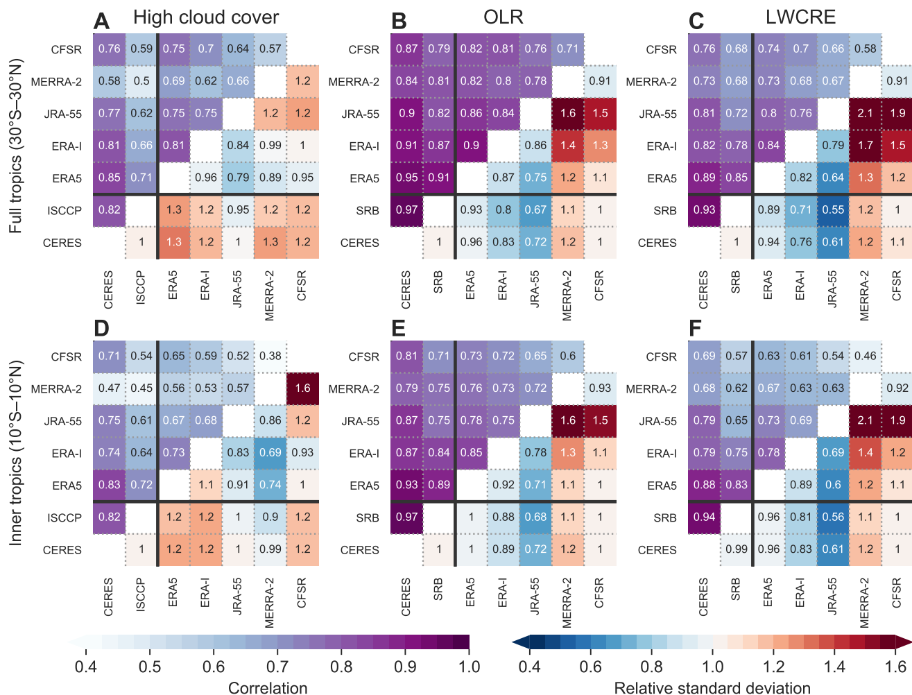
Figure 15. Metrics measuring agreement in monthly anomalies of (A, D) HCC, (B, E) OLR, and (C, F) the LWCRE among the reanalyses and observational data sets examined in this paper. The upper left triangle in each panel shows correlation coefficients between each pair of products, while the lower right triangle shows the standard deviation in the product marked on the horizontal axis relative to that in the product marked on the vertical axis. Both metrics are evaluated first for individual grid cells in the 2.5^\circ common grid (see, e.g., Fig. 1) and then averaged. The upper row (A–C) shows results for the entire tropics ( 30^\circ\text{S} – 30^\circ\text{N} ), while the lower row (D–F) shows results for the inner tropics only ( 10^\circ\text{S} – 10^\circ\text{N} ). Solid black lines separate evaluations relative to the observational benchmarks based on CERES, ISCCP, and NASA-GEWEX SRB from those based on intercomparison of reanalysis products.
