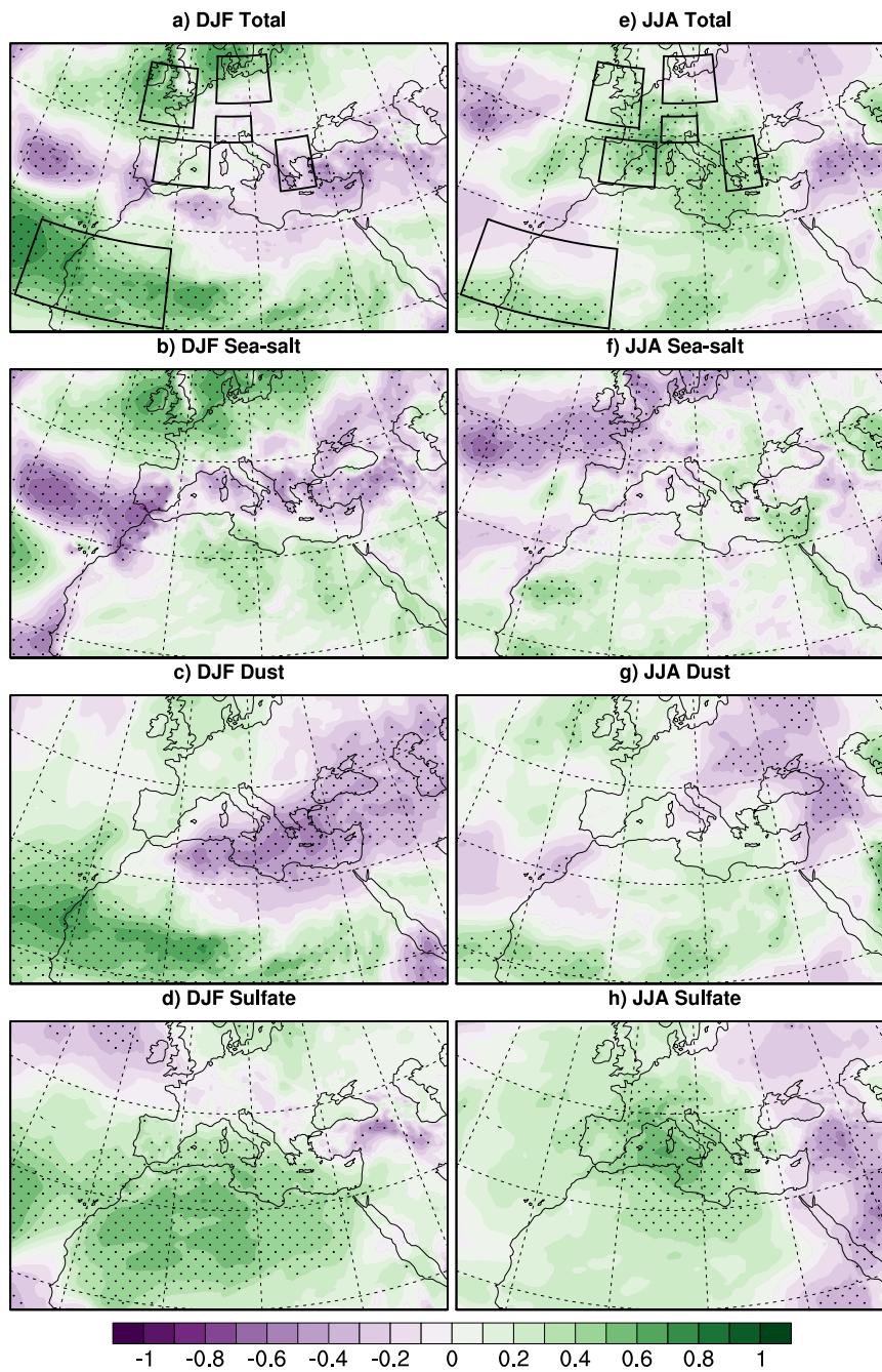
Figure 9. Correlation between NAO index and AOD (total and by aerosol type) at 550nm simulated by ALADIN over the period 1979-2018, separately for DJF (left, a-d) and JJA (right, e-h) seasonal means. Dotted areas are significant at the level 0.05
