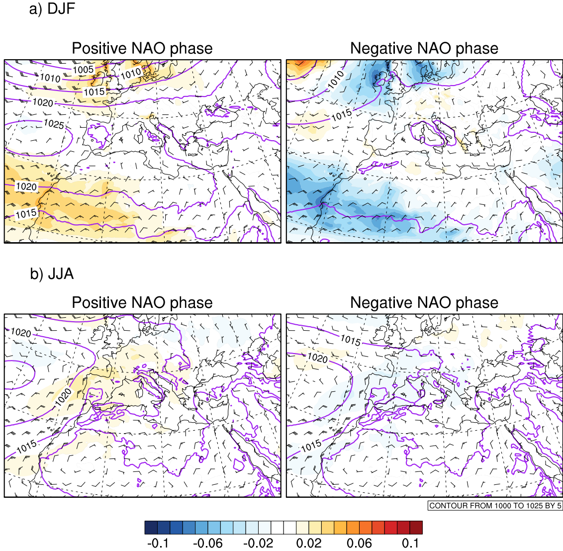
Figure 10. Averaged (1979-2018) atmospheric circulation (sea level pressure in hPa, purple lines, and surface wind with black wind barbs representing 2 \text{ km h}^{-1} ) with AOD anomalies (colors) simulated by ALADIN in winter (DJF, top) and in summer (bottom), respectively for the positive (left) and negative (right) phase of NAO.
