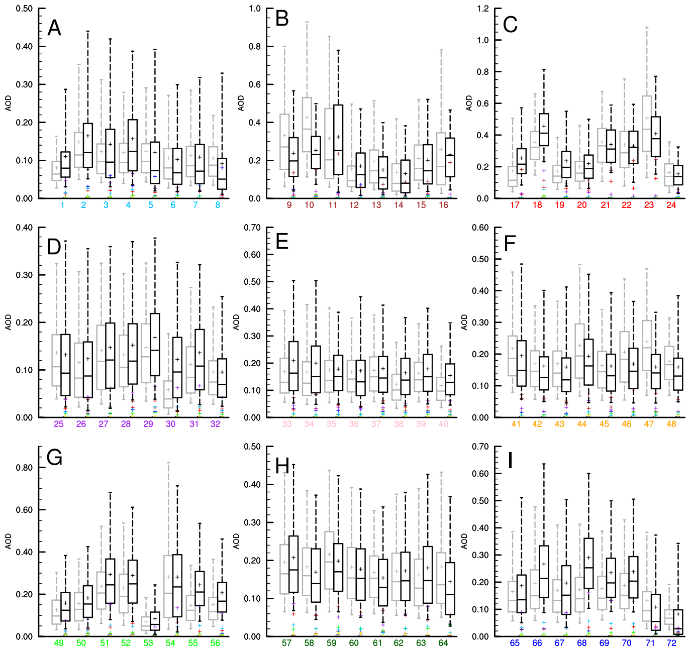
Figure 8. Box plots comparing daily AOD simulated by CNRM-ALADIN63 (in black) to AERONET measurements (in grey). The numbers in the x-axis correspond to the respective stations defined in Figure 1 and Table 2. The limits of each boxplot are given by the first and third quartiles, the inner horizontal line is the median, while the whiskers limited by the 5th and 95th percentiles. Colored crosses represent the average total AOD (AERONET in grey, ALADIN in black) and the contribution of each aerosol type in ALADIN (dust in brown, sea-salt in dark blue, sulphate in red, organic matter in green, black carbon in yellow, nitrates in purple and ammonium in light blue). Only the days where observations are available have been taken into account in the 45 model. Note that the AOD scale is adapted to each region.
