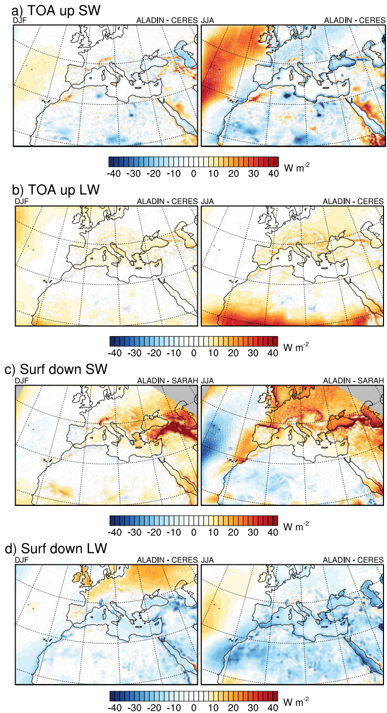
Figure 4. Winter (DJF, left) and summer (JJA, right) average differences between ALADIN and satellite data for shortwave (SW) and longwave (LW) radiation ( W m^{-2} ) at the top of the atmosphere (upward fluxes, a for SW, b for LW) and at the surface (downward fluxes, c for SW, d for LW). Satellite data used here are CERES (2000-2016) in a, b and d, as well as SARAH (1983-2015) in c.
