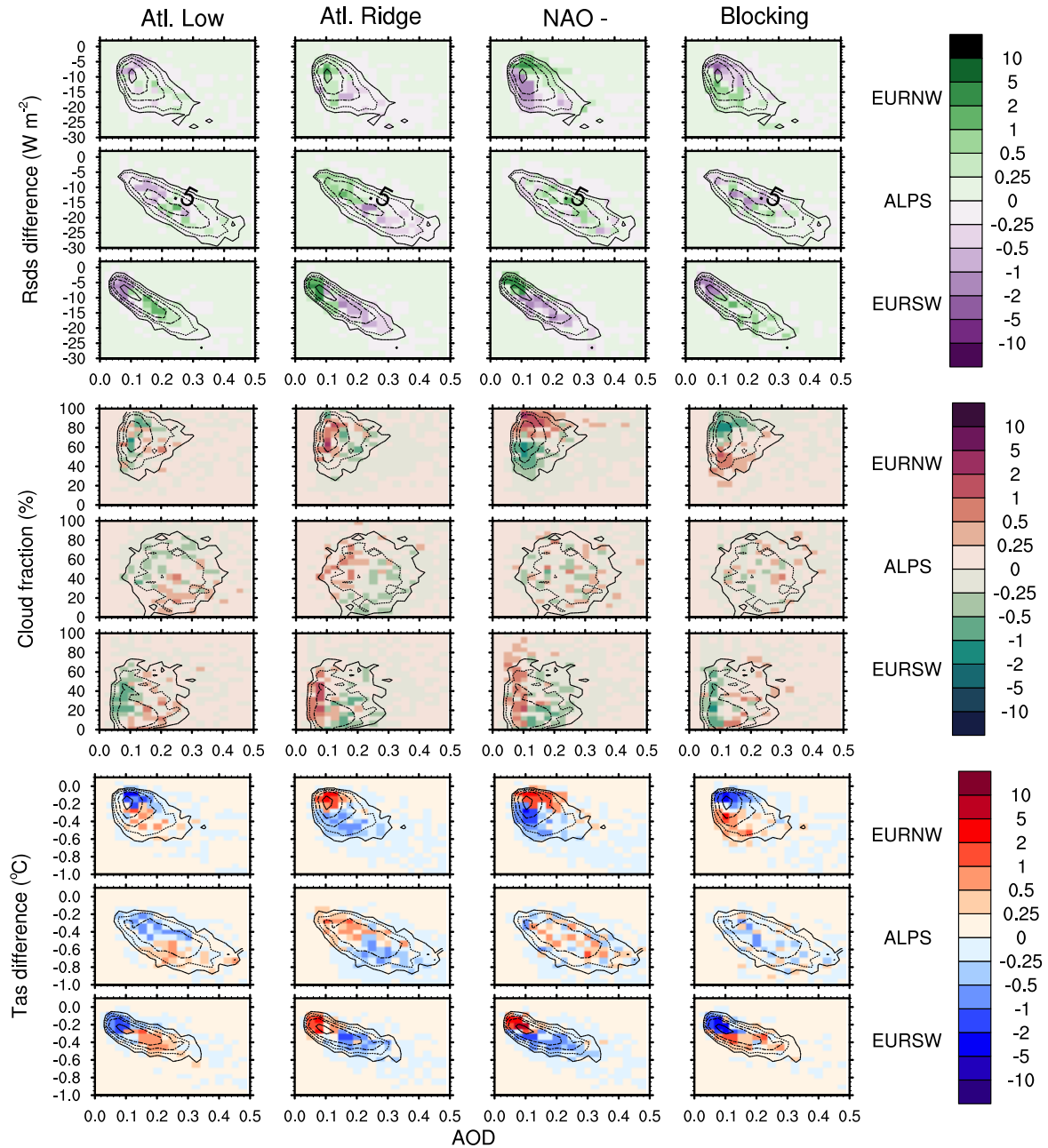
Figure 18. Same as Figure 17 but for summer (JJA).
