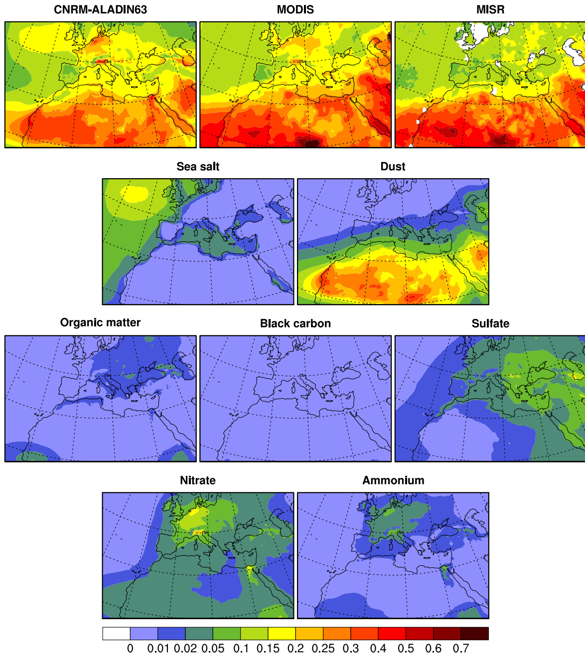
Figure 6. Averaged AOD (total and for each aerosol type) at 550 nm simulated by ALADIN-Chimat CNRM-ALADIN63 between 2003 and 2017. Total AOD from MODIS and MISR has been included on the first line.
