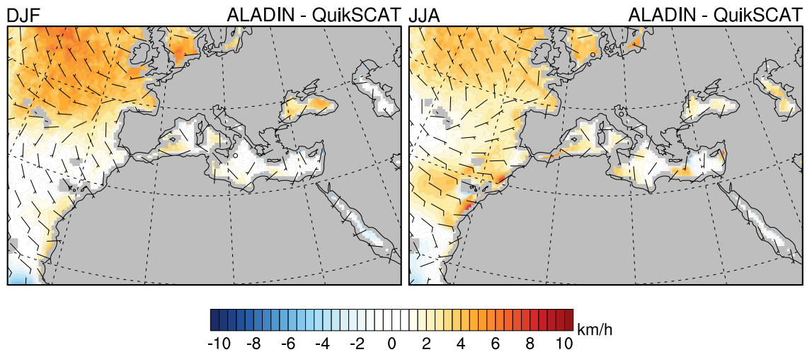
Figure 2. Winter (DJF, left) and summer (JJA, right) average differences between ALADIN and ERA-Interim for sea level pressure (hPa, 1979-2016, top), and between ALADIN and QuikSCAT for surface wind ( \text{km/h km h}^{-1} , 2000-2009, bottom). \odot Wind speed representation as in meteorological maps, one wind barb represents 2 \text{ km/h km h}^{-1} . In the upper left figure, the PRUDENCE boxes (Christensen and Christensen, 2007) used for the evaluation of the model (see Table 3) are shown in black lines, the land Europe and Mediterranean Sea domains in purple lines.
