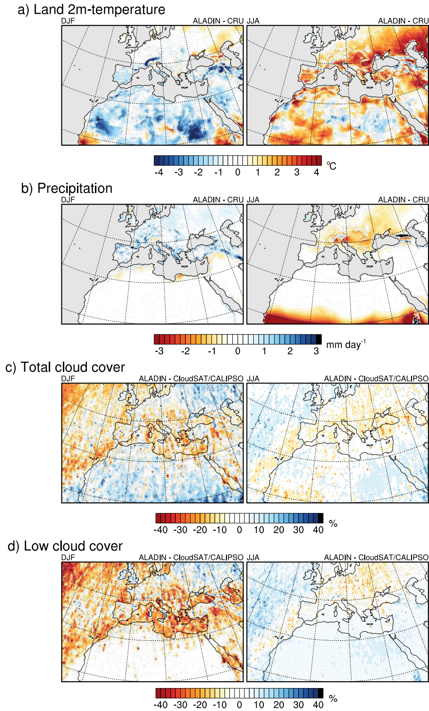
Figure 3. Winter (DJF, left) and summer (JJA, right) average differences between ALADIN and observations (CRU and CloudSAT/CALIPSO) for 2m-temperature (°C, 1979-2015, a), precipitation ( \text{mm/day} \text{mm day}^{-1} , 1979-2015, b) and cloud cover (% , 2006-2011, total fraction in c, low fraction in d).
