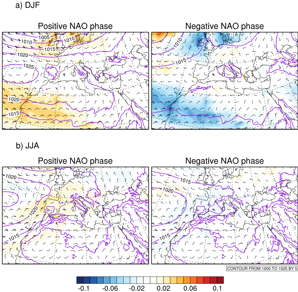
Figure 10. Averaged (1979-2018) atmospheric circulation (sea level pressure in hPa, purple lines, and surface wind with black wind bars representing 2 \text{ km h}^{-1} ) with AOD anomalies (colors) simulated by ALADIN in winter (DJF, top) and in summer (bottom), respectively for the positive (left) and negative (right) phase of NAO.
