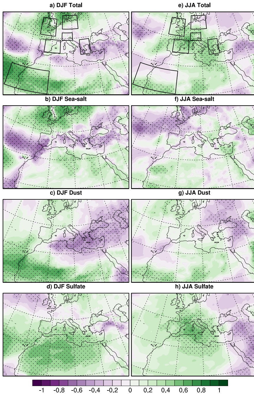
Figure 9. Correlation between NAO index and AOD (total and by aerosol type) at 550nm simulated by ALADIN- Climat over the period 1979-2018, separately for DJF ( left , a-d) and JJA ( right , e-h) seasonal means . Dotted areas are significant at the level 0.05
