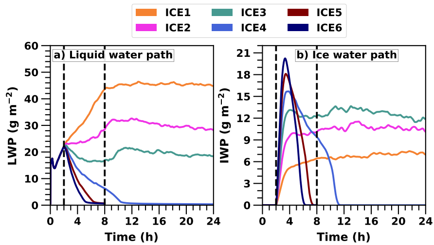
Figure 3. Liquid and ice water path time series in UCLALES-SALSA simulations with fixed ice number concentrations of 1, 2, 3, 4, 5 and 6 L -1 (ICE1, ICE2, ICE3, ICE4, ICE5 and ICE6, respectively).
