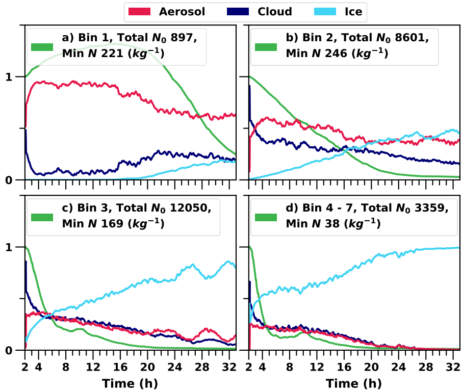
Figure 6. Relative proportions of hydrometeors at each time step in the cloud layer. Cloud layer is defined when both cloud liquid water and ice mixing ratios are over 0.001 ( g\ kg^{-1} ). Black Green line represents relative change of the total number concentration in each bin.
