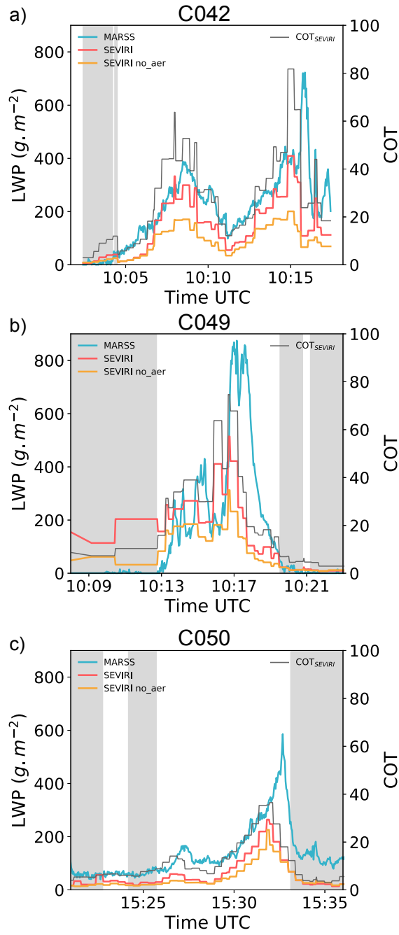
5 Figure 11: Comparison of the LWP measured from MARSS (blue) during straight level run above the clouds from flight C042 (a), C049 (b) and C050 (c) and collocated LWP from SEVIRI calculated based on the COT and CER retrieved with (red) and without (orange) taking into account the absorption of aerosol above clouds. The COT retrieved by SEVIRI taking into account the overlying aerosols is plotted in black. The grey areas correspond to the SEVIRI pixels that are rejected because of the filters on cloud inhomogeneity, cloud edges and/or unsatisfying fit of the measurements by the forward model.
