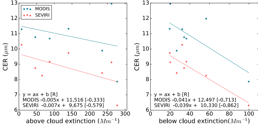
Figure 9: CER (in \mu\text{m} ) retrieved by SEVIRI (red) and MODIS (blue) as a function of the dry extinction (in \text{Mm}^{-1} ) measured by EXSCALABAR at 405 nm and averaged over 100m directly above (a) and below the cloud (b). The linear regression fits are defined by the slope a , the intercept b and the Pearson's correlation coefficient R .
