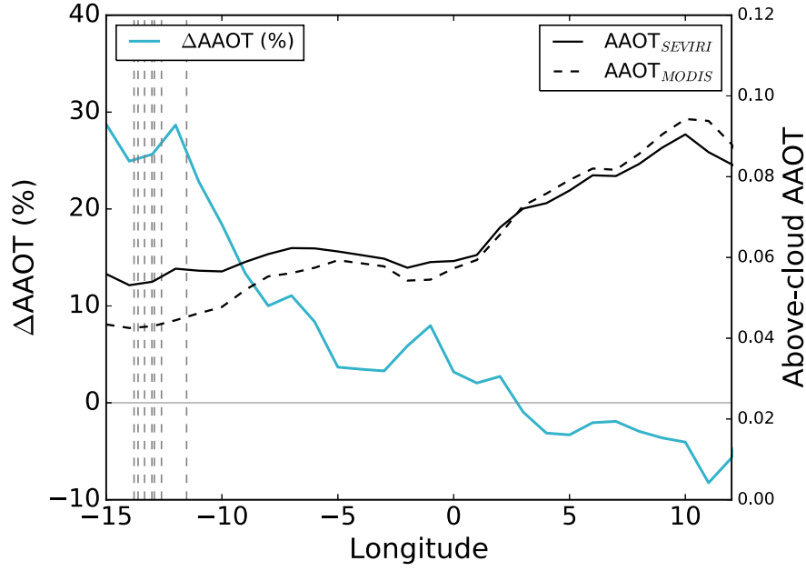
Figure 7: Longitudinal variation of the above-cloud AAOT from SEVIRI (black solid line), MODIS (black dashed line) and the difference \Delta\text{AAOT} in percentage (blue line) for the data used in Figure 3, removing \text{AAOT}_{\text{SEVIRI}} lower than 0.03. The dashed vertical lines correspond to the location of the dropsondes used in Figure 6.
