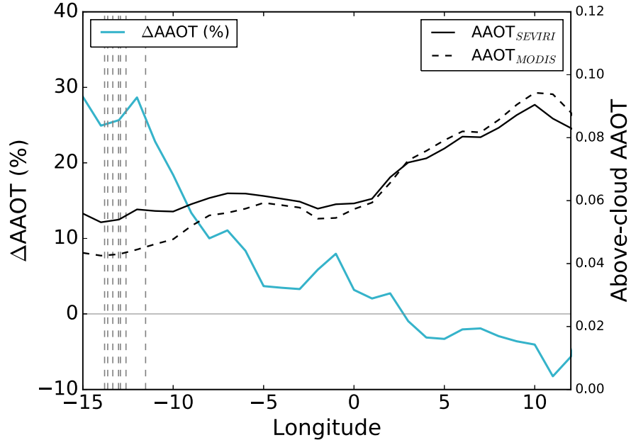
Figure 67: Longitudinal variation of the difference \Delta\text{AAOT} (in %) between the SEVIRI and MODIS AAOT above-cloud AAOT from SEVIRI (black solid line), MODIS (black dashed line) and the difference \Delta\text{AAOT} in percentage (blue line) for the data used in Figure 3, removing \text{AAOT}_{\text{SEVIRI}} lower than 0.03. The dashed vertical lines correspond to the location of the dropsondes used in Figure 56.
