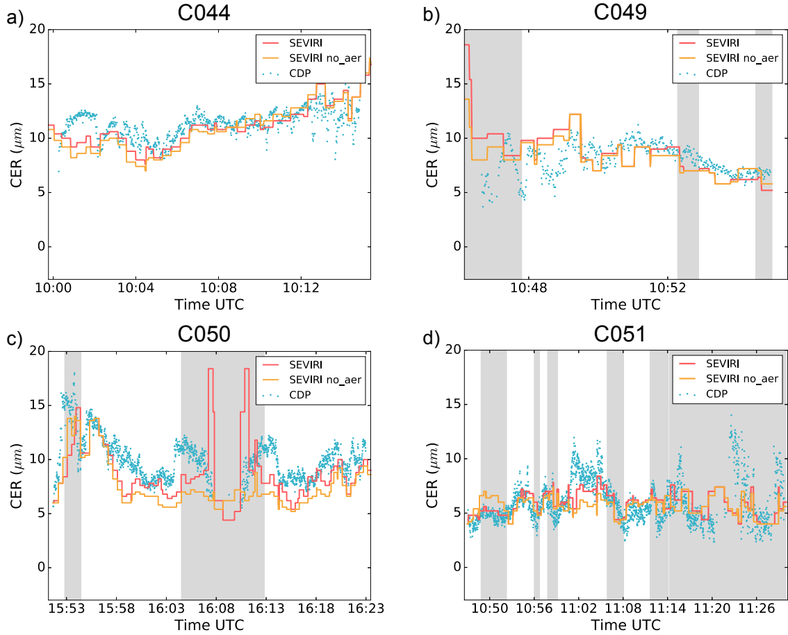
Figure 910: Comparison of the CER measured by the CDP during straight level run through clouds and from flight C044 (a), C049 (b), C050 (c) and C051 (d) and the collocated SEVIRI retrievals with and without taking into account the absorption of aerosol above clouds. The grey areas correspond to the SEVIRI pixels that are rejected because of the filters on cloud inhomogeneity, cloud edges and/or unsatisfying fit of the measurements by the forward model.
