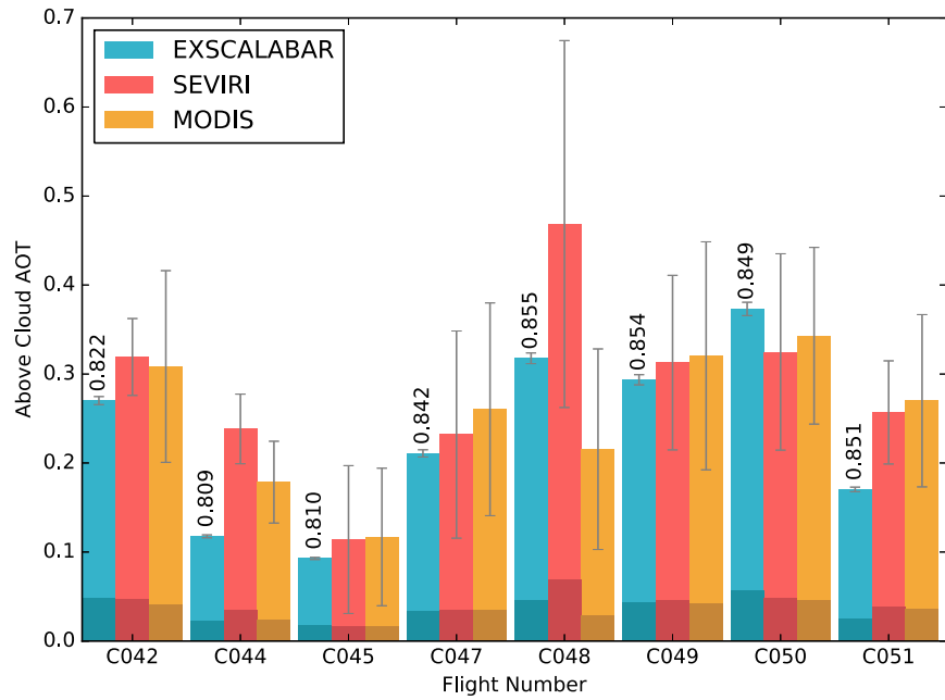
Figure 78: Comparison of the above-cloud AOT (lighter shades) and AAOT (darker shades) retrieved by SEVIRI and MODIS and measured by EXSCALABAR during descent profiles. The error bars represent the uncertainties of the EXSCALABAR measurements and the standard deviation of the satellite product within a 60 km radius around the aircraft measurements for SEVIRI and MODIS. The SSA has been calculated at 0.55 \mu\text{m} from the EXSCALABAR observations and included as an annotation over the EXSCALABAR above-cloud AOT.
