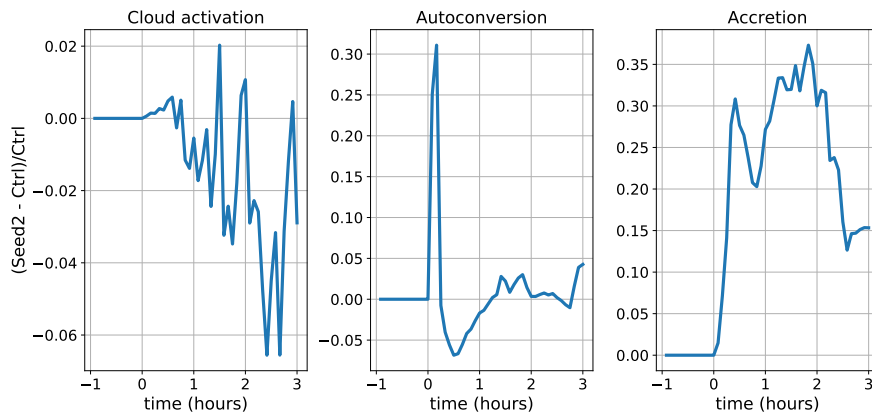
Figure 13. Relative change in process rates between the Ctrl and Seed2 configurations in per cent, calculated from the mean values taken across the ensemble simulations as a function of time (since the seeding injection). Starting from the left, the panels show the change in cloud activation, autoconversion (drizzle formation) and accretion rates.
