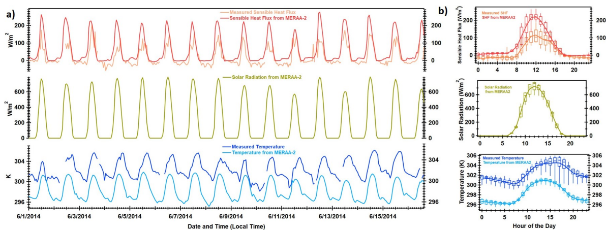
Figure 2. a) Timeseries and b) diel box and whisker plots for the measured air temperature and sensible heat flux (SHF) along with estimated air temperature, solar radiation and sensible heat flux obtained from MERA-2. The timestamp in the X-axis of Figure 2b represents the start-time of the respective hourly data bin (e. g. 6 for data averaged between 6 and 7).
