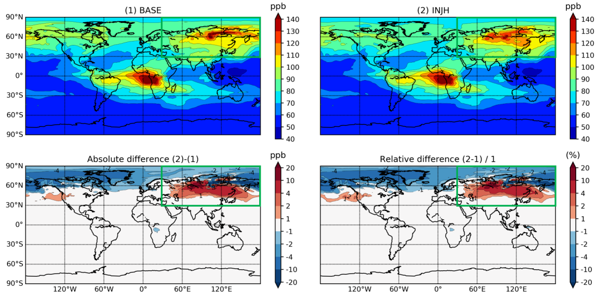
Figure 9. Monthly mean differences of CO mixing ratios between the BASE and IJNH MOCAGE simulations on 350 hPa iso-surface for the month of August 2013. The green box indicate the area used for the zonal mean.
