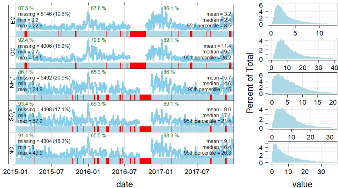
Fig. 2. Fig. S2. NO 3 - , SO 2 , NH 4 + , OC (organic carbon) and EC (element carbon) data quality assurance and control.
