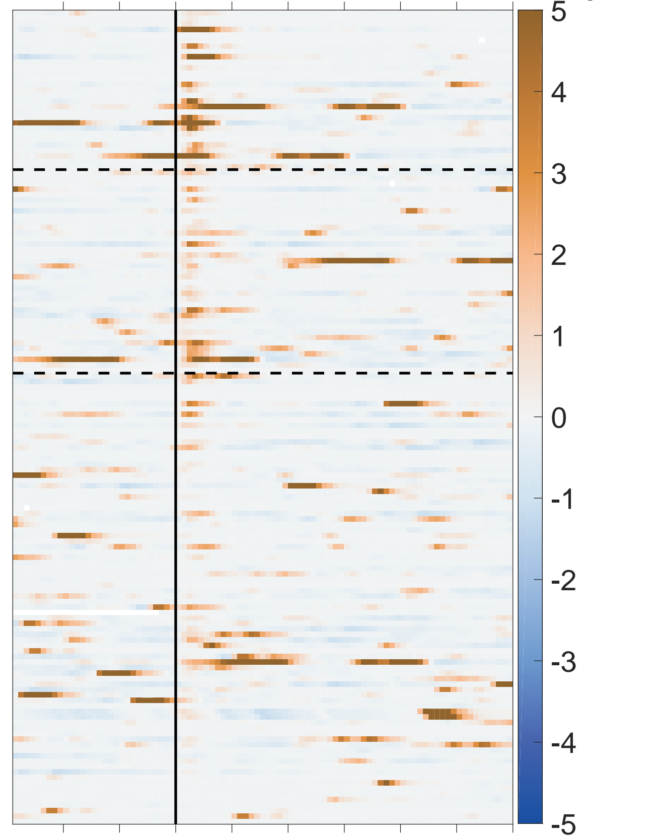
HNO 3 Southern hemisphere
