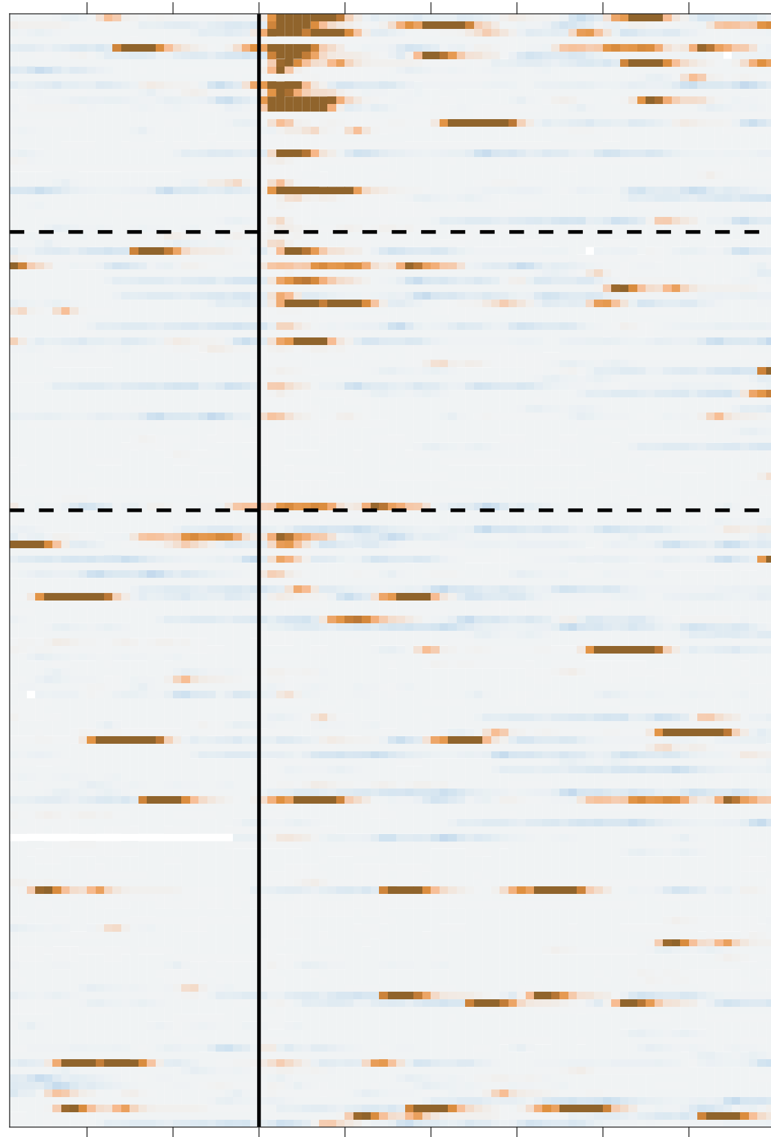
HNO 3 Northern hemisphere
