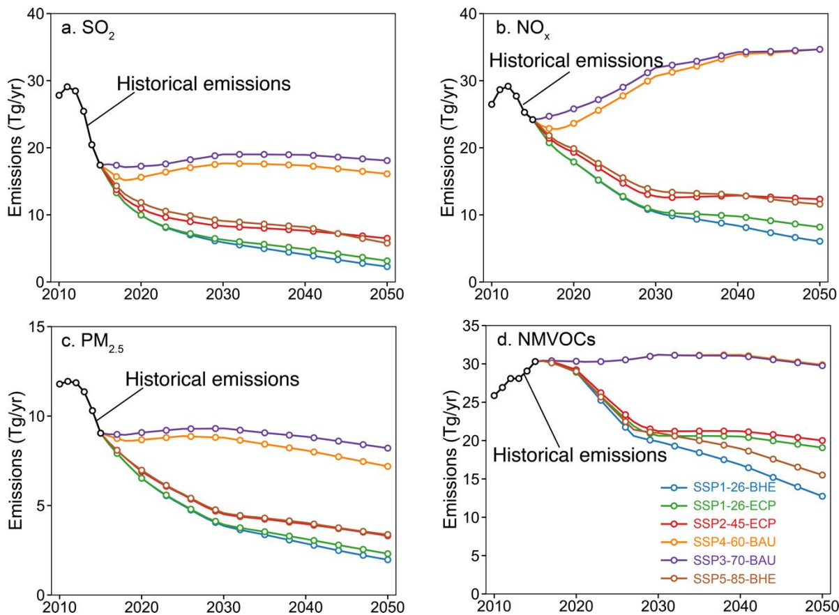
Figure 7: Emissions of major air pollutants in China from 2010 to 2050. The species plotted here include (a) SO 2 , (b) NO x , (c) PM 2.5 , (d) NMVOCs. This figure shows the historical annual emission data from 2010-2015 and emission projections (one dot every three years) under six designed scenarios during 2015-2050 (SSP1-26-ECP, SSP1-26-BHE, SSP2-45-ECP, SSP3-70-BAU, SSP4-60-BAU, and SSP5-85-BHE scenarios).
