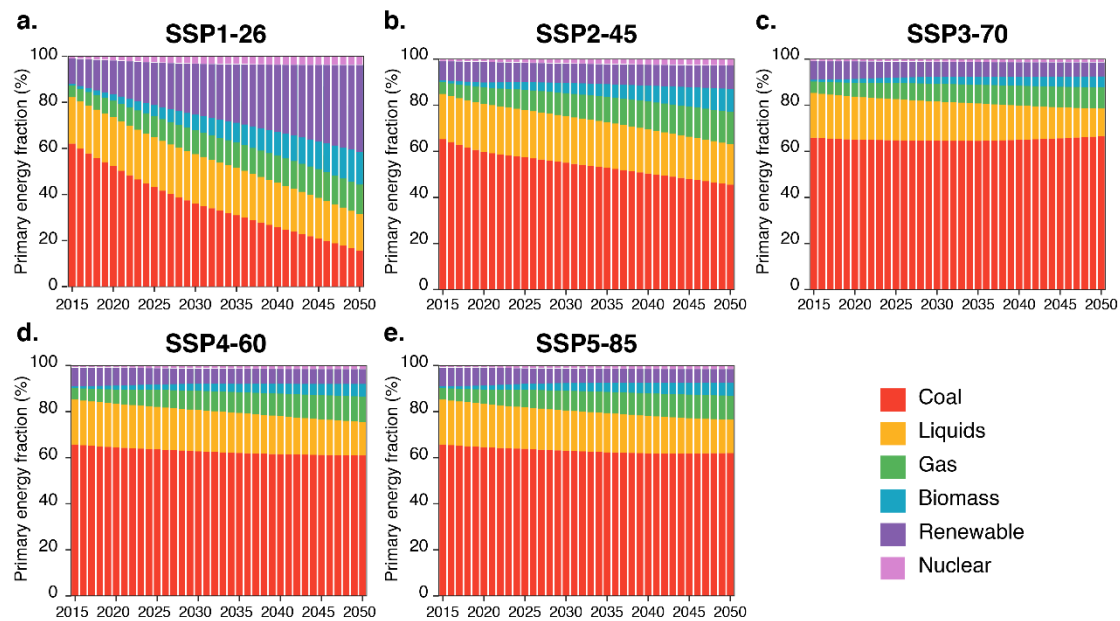
1170 Figure 5: Evolution of primary energy structure under different scenarios. The scenarios plotted here include (a) SSP1-26, (b) SSP2-45, (c) SSP3-70, (d) SSP4-60, (e) SSP5-85 scenarios. This figure shows the yearly changes of primary energy (coal, liquids, gas, biomass, renewable, and nuclear) structure under five combined social-economic-energy scenarios during 2015-2050.
