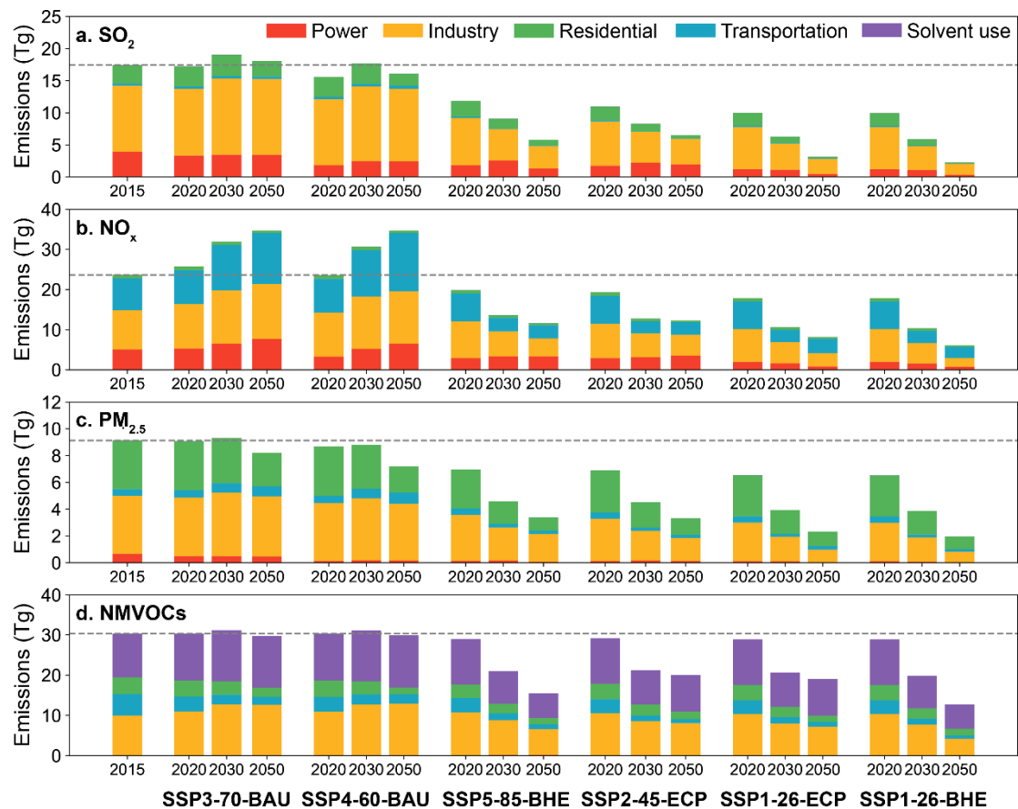
Figure 8: China's future anthropogenic emissions by sector in the year of 2030 and 2050 under six scenarios. The species plotted here include (a) SO 2 , (b) NO x , (c) PM 2.5 , (d) NMVOCs. Emissions are divided into five source sectors (stacked column chart): power, industry, residential, transportation, and solvent use.
