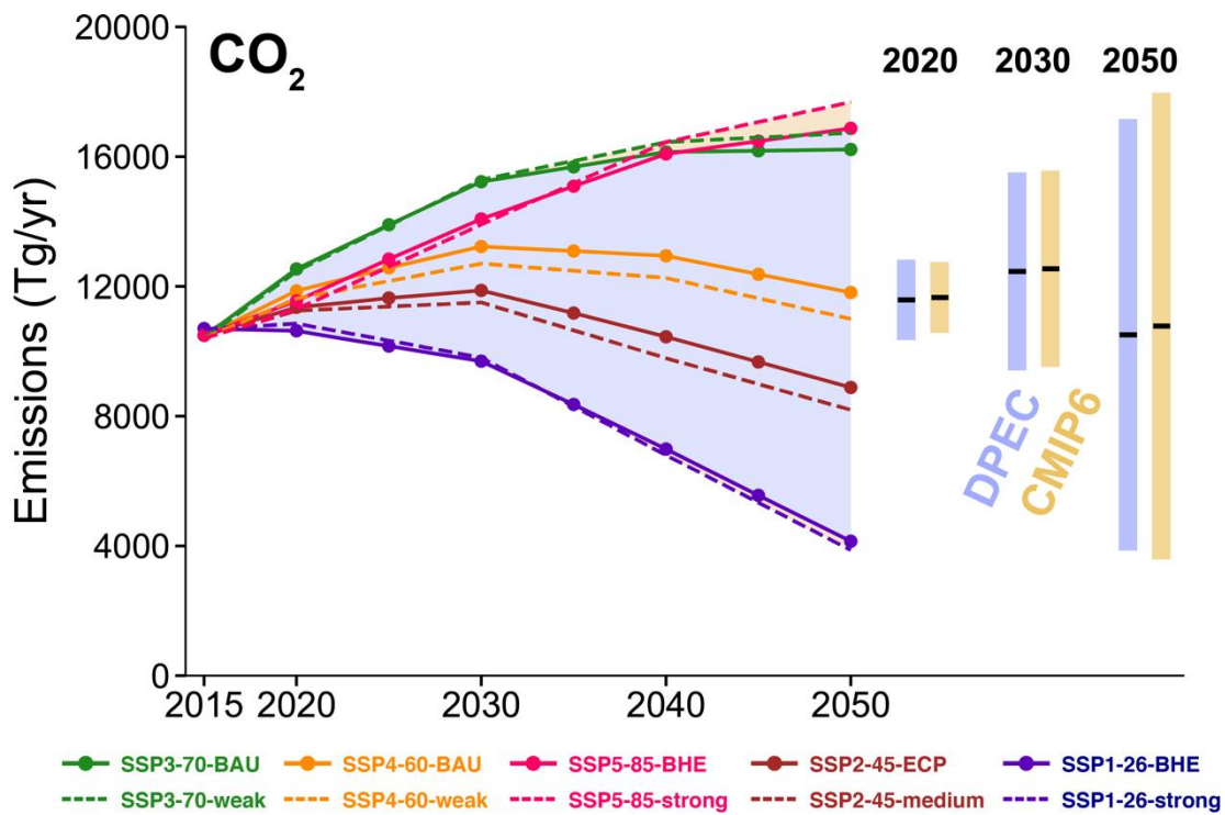
1190 Figure 10: Comparison of future CO 2 emissions estimated in this study with estimates from CMIP6 database. The scenario includes SSP1-26-BHE, SSP2-45-ECP, SSP3-70-BAU, SSP4-60-BAU, and SSP5-85-BHE scenarios from this study, and the corresponding SSP1-26-strong, SSP2-45-medium, SSP3-70-weak, SSP4-60-weak, and SSP5-85-strong scenarios from CMIP6 report.
