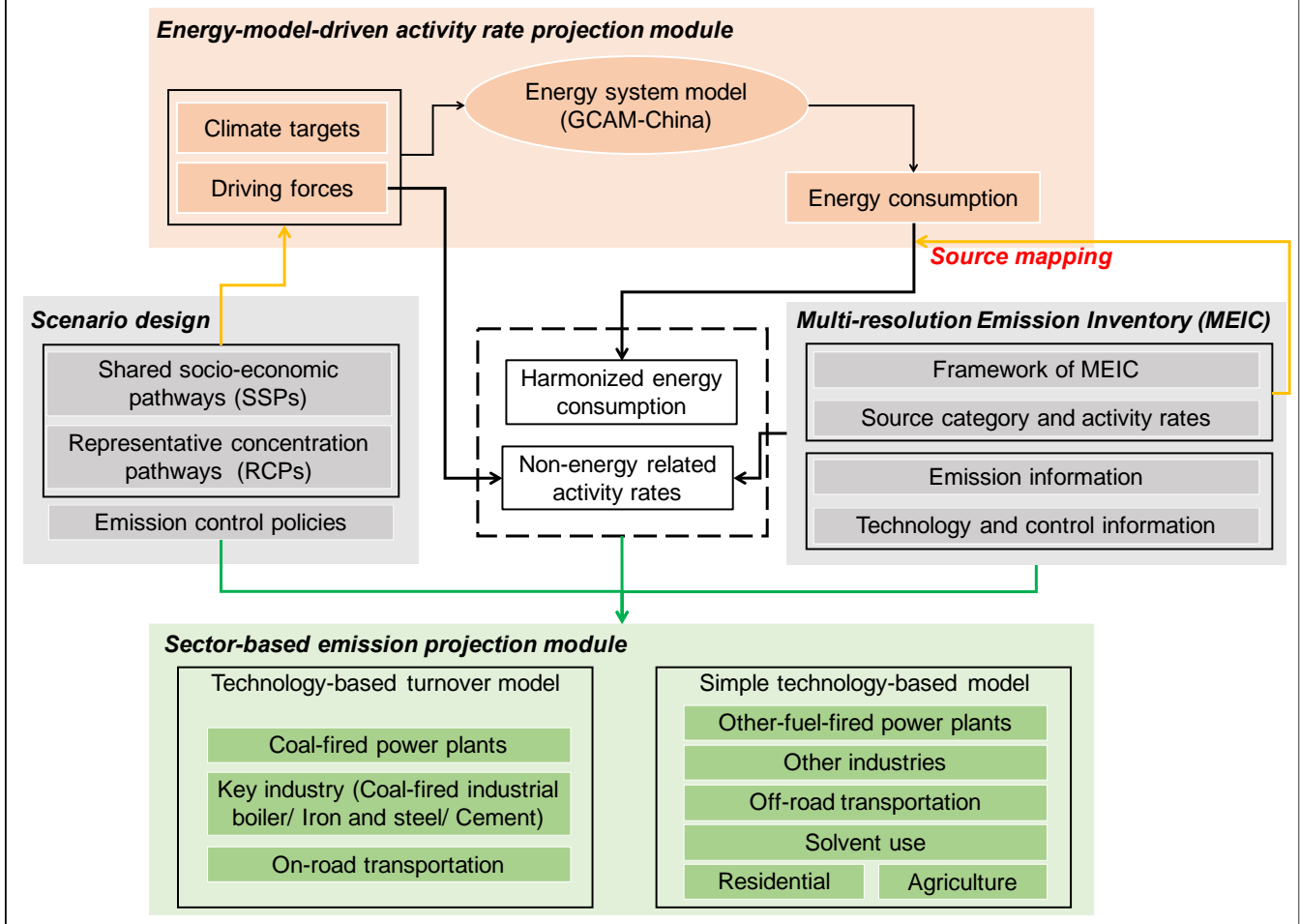
1145 Figure 1: Framework of the Dynamic Projection model for Emissions in China (DPEC).
