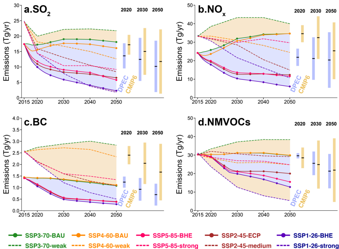
1185 Figure 9: Comparison of future emissions estimated in this study with estimates from CMIP6 database. The species plotted here include (a) SO 2 , (b) NO x , (c) BC, (d) NMVOCs. The scenario includes SSP1-26-BHE, SSP2-45-ECP-SSP3-70-BAU, SSP4-60-BAU, and SSP5-85-BHE scenarios from this study, and the corresponding SSP1-26-strong, SSP2-45-medium, SSP3-70-weak, SSP4-60-weak, and SSP5-85-strong scenarios from the CMIP6 database.
