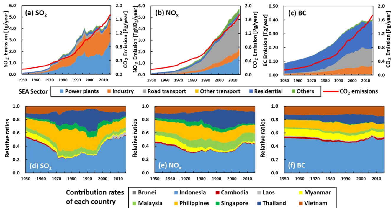
1335 Figure 6. Emissions of (a) SO 2 , (b) NO x , and (c) BC from each major sector in SEA (upper panels) and (d, e, f) relative ratios of emissions from each country in SEA (lower panels) during 1950-2015. Red lines in the upper panels are total CO 2 emissions.
