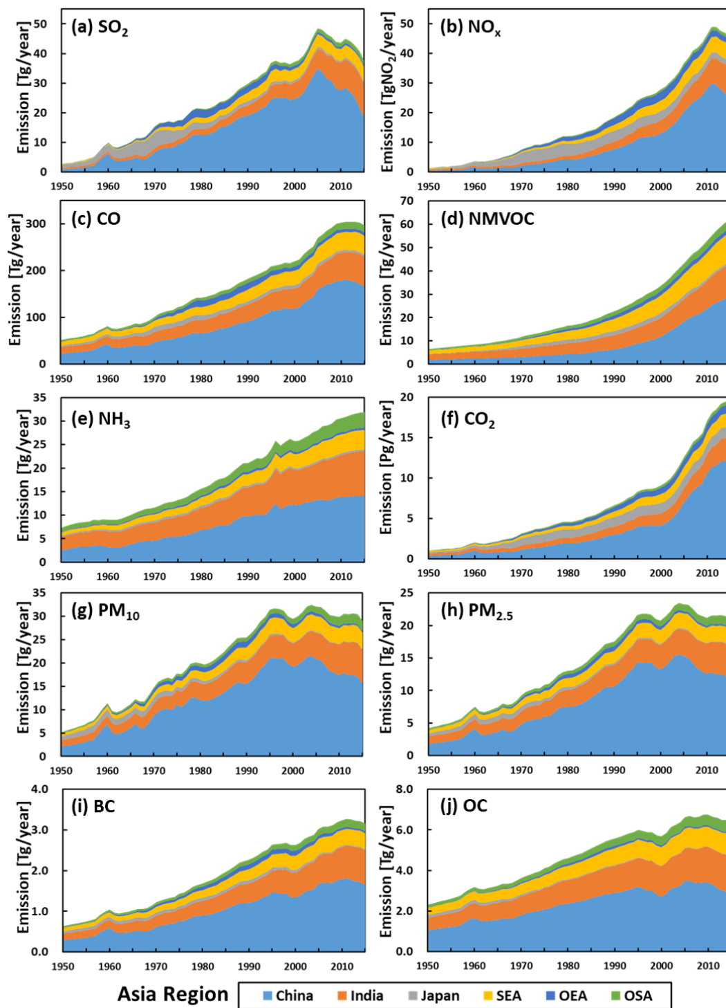
1320 Figure 2. Trends of (a) \text{SO}_2 , (b) \text{NO}_x , (c) \text{CO} , (d) \text{NMVOC} , (e) \text{NH}_3 , (f) \text{CO}_2 , (g) \text{PM}_{10} , (h) \text{PM}_{2.5} , (i) \text{BC} , and (j) \text{OC} emissions in Asia during 1950-2015 for each region. See Fig. 1 for countries included in SEA, OEA, and OSA.
