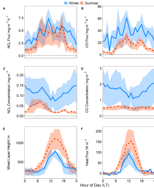
Figure 5. Average diurnal profiles for A) \text{NO}_x flux, B) CO flux, C) \text{NO}_x concentration, D) CO concentration and E) mixed layer height and F) heat flux. Blue, solid lines are for measurements taken during the winter campaign and the orange, dashed lines are measurements taken during the summer campaign. The shaded areas represent the 25 th and 75 th percentiles. For the \text{NO}_x and CO fluxes, only stationary data has been used but no u_* filtering has been applied when doing the diurnal averaging, as described in section 2.5.1.
