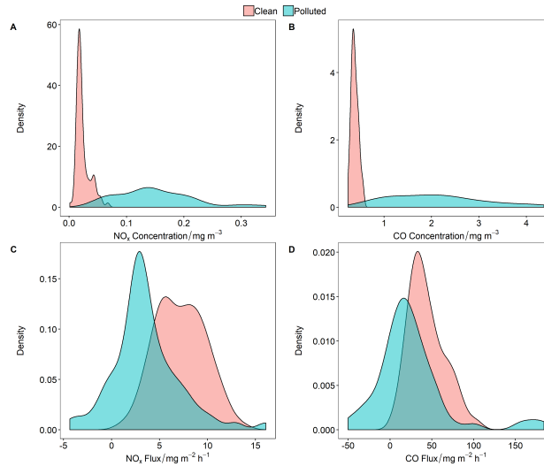
Figure 6. The density distribution of \text{NO}_x and CO concentrations and fluxes during the “clean” period (21 November 2016 – 23 November 2016) and “polluted” period (24 November 2016 – 27 November 2016). Only fluxes for which u_* values are over 0.175 \text{ m s}^{-1} and which meet the 60 % stationarity criteria are presented to allow a valid comparison.
