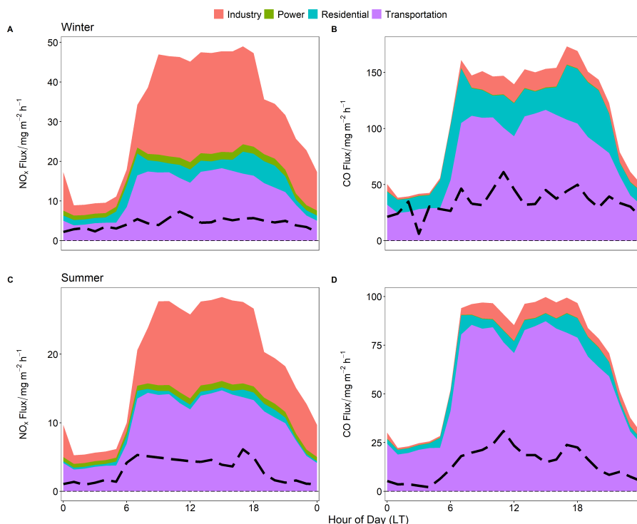
Figure 10. Measured diurnal trend (dashed black line) and predicted diurnal trend using the MEIC inventory (filled areas by sector) for \text{NO}_x and CO emissions. MEIC inventory data has been reduced by 30 % for comparison with the winter 2016 campaign and by 43 % for comparison with the summer 2017 campaigns to take account of expected emissions reductions indicated in Cheng et al. (2019). Panels A and B show emissions for the winter campaign and panels C and D show emissions from the summer campaign.
