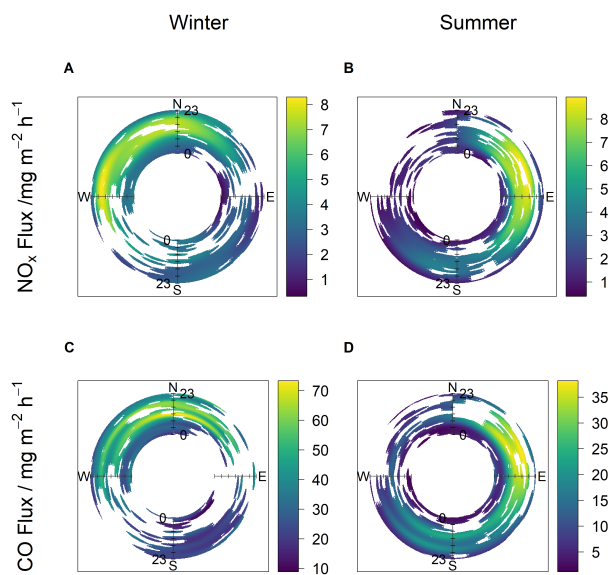
Figure 8. Polar annulus plots for \text{NO}_x and CO fluxes for both campaigns, showing the relationship between mean diurnal flux and wind direction. 0 – 23 refers to hour of day and the colour scale shows flux in \text{mg m}^{-2} \text{h}^{-1} .
