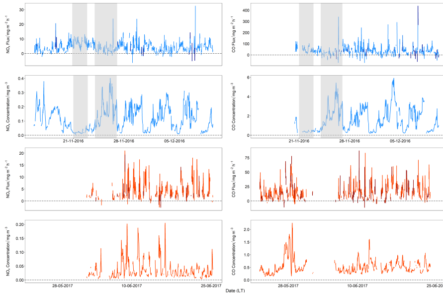
Figure 4. Time series data for 30 minute averaged \text{NO}_x and CO fluxes for the winter (blue trace) and summer (orange trace) campaigns with fluxes outside of the 60 % stationarity criteria shown in darker colours. Gaps in the time series are due to instrument problems. The two contrasting periods discussed in section 3.2 are highlighted in grey.
