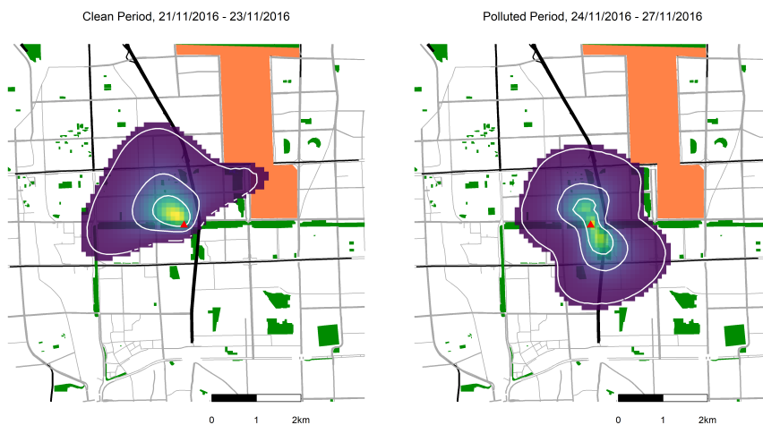
Figure 7. Average footprints for the “clean” period, 21 November 2016 – 23 November 2016 (left) and the “polluted” period, 24 November 2016 – 27 November 2016 (right). Map was built using data from © OpenStreetMap contributors 2019. Distributed under a Creative Commons BY-SA License.
