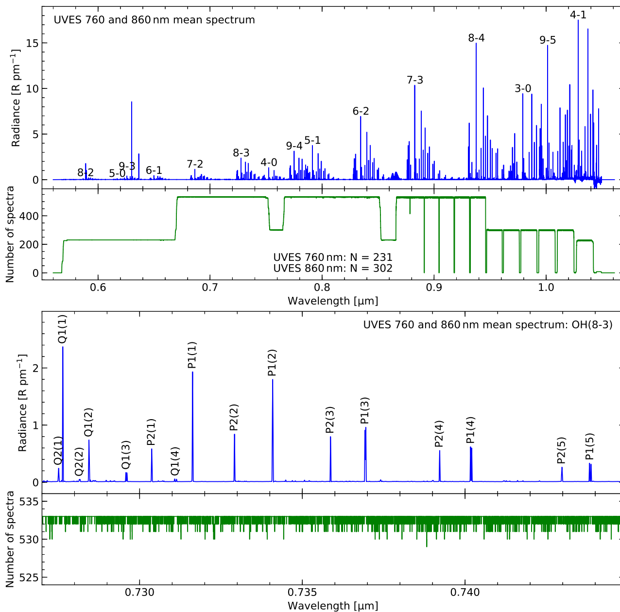
Figure 1. UVES mean spectrum in rayleighs per picometre. The full spectral range with labelled OH bands is shown at the top. At the bottom, a narrower wavelength range focussing on the Q and P branch of OH(8-3) is plotted. The lines are labelled. The wavelength-dependent number of spectra involved in the calculation of the mean spectrum is indicated in additional subpanels. This number varies due to the use of two set-ups centred on 760 and 860 nm (with some variation) and the \sigma -clipping procedure for the mean calculation.
