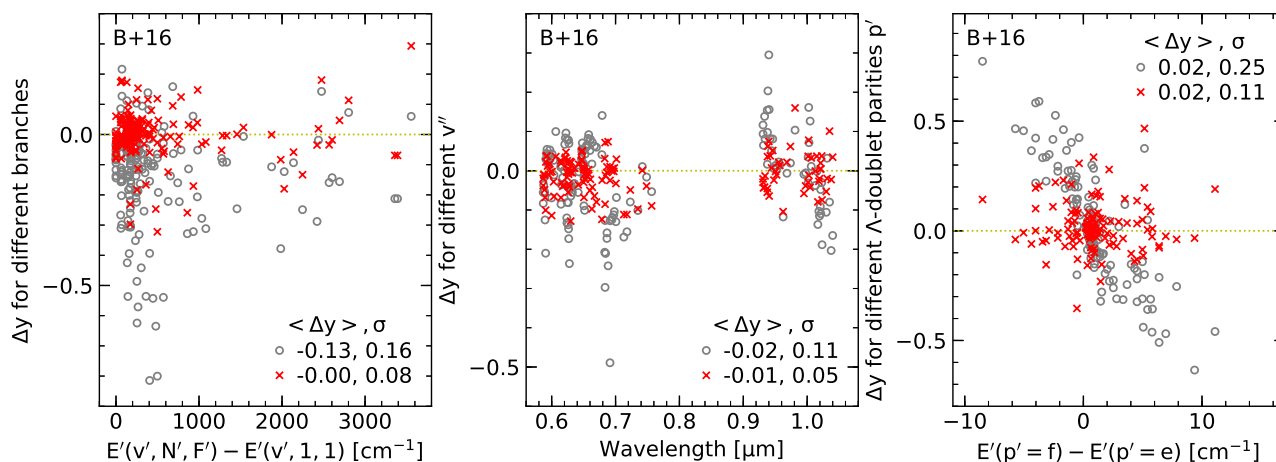
Figure 11. Correction of Brooke et al. (2016) Einstein-A coefficients. The measured (circles) and corrected (crosses) OH level population ratios \Delta y are given for changes in the branch (left; c.f. Fig. 6), lower vibrational level v'' (middle; c.f. Fig. 8), and the \Lambda -doublet component (right; c.f. Fig. 9). Each plot lists the mean \Delta y and standard deviation \sigma for the measured and corrected data.
