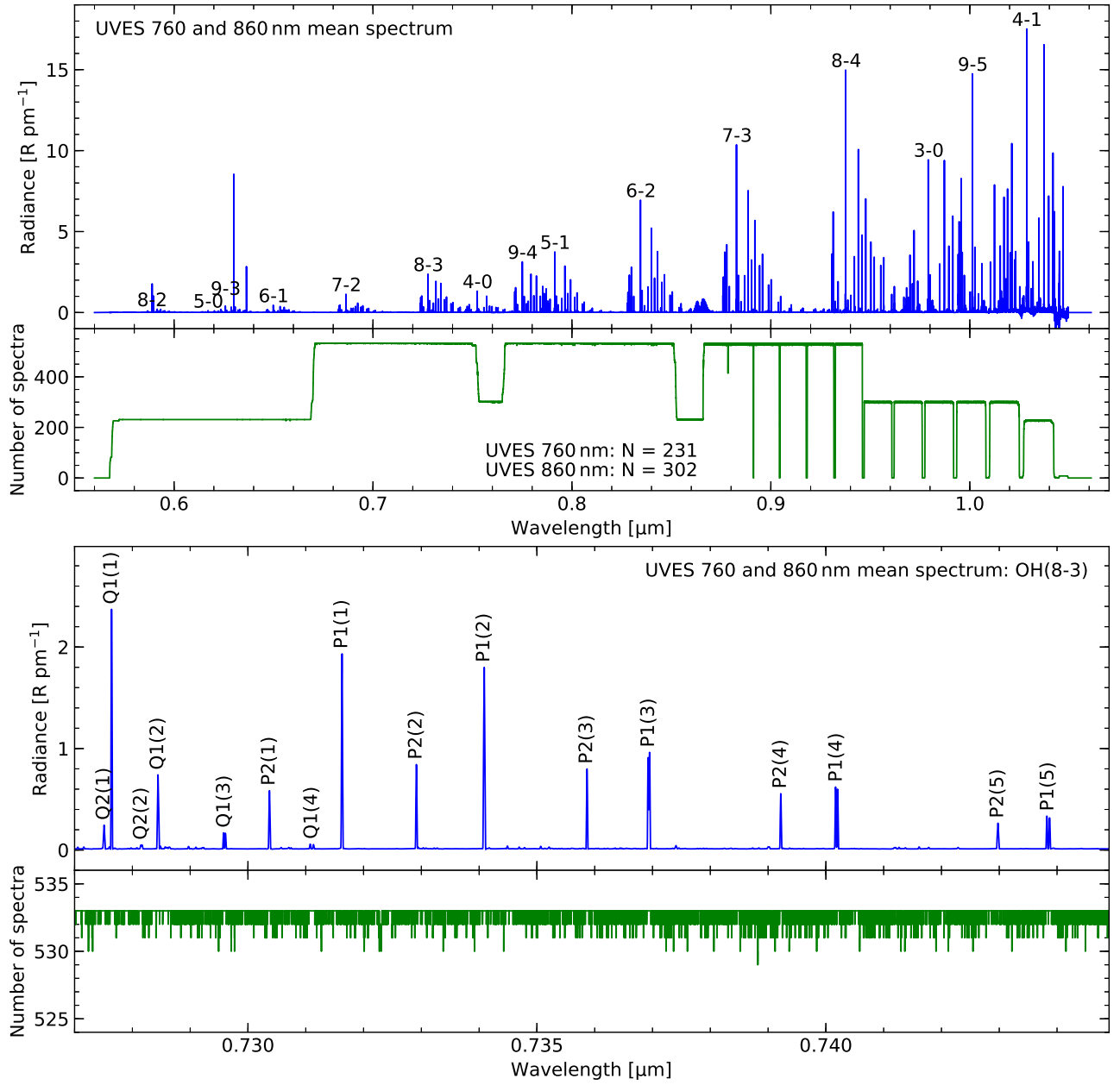
Figure 1. UVES mean spectrum in rayleighs per picometre. The full spectral range with labelled OH bands is shown at the top. At the bottom, a narrower wavelength range focussing on the Q and P branch of OH(8-3) is plotted. The lines are labelled. The wavelength-dependent number of spectra involved in the calculation of the mean spectrum is indicated in additional subpanels. This number varies due to the use of two set-ups centred on 760 and 860 nm (with some variation) and the \sigma -clipping procedure for the mean calculation.
