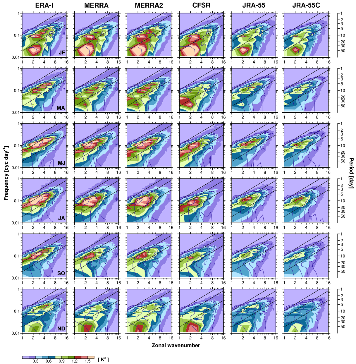
Figure A1. The same as in Fig. 1 except for the 100-hPa spectra in different months: January–February, March–April, May–June, July–August, September–October, and November–December (JF, MA, MJ, JA, SO, and ND, respectively, from top to bottom).
