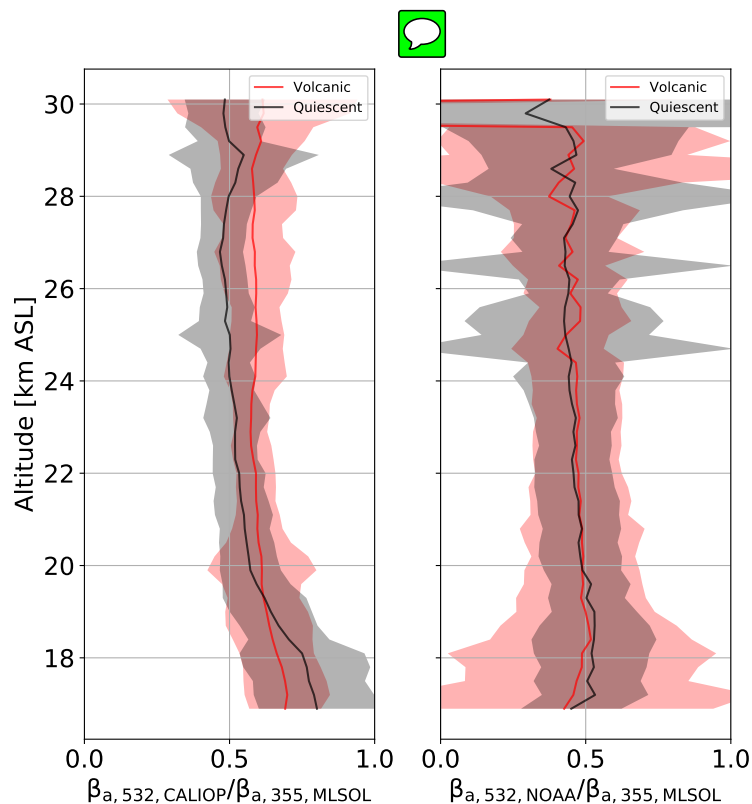
Figure 5. Average color ratio for the volcanic (solid, red) and second quiescent (solid, black) periods derived from CALIOP and MLSOL measurements (left), and NOAA lidar and MLSOL measurements (right).
