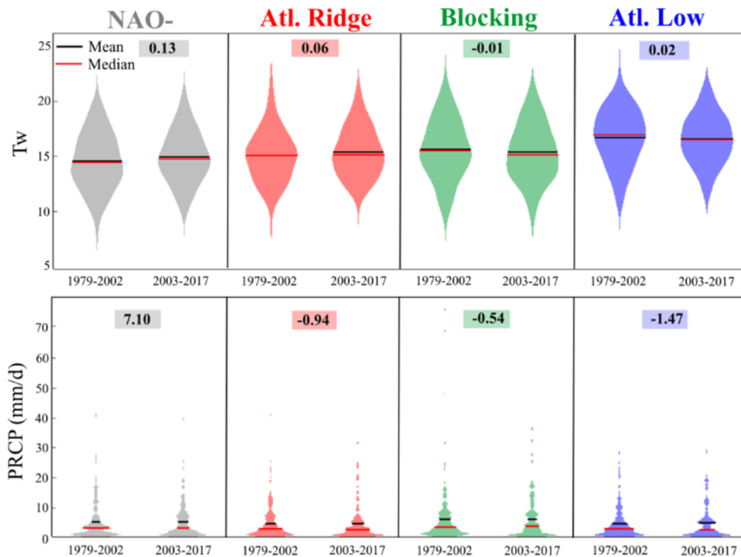
Fig. 5. Violin plot of daily Tw (first line) and PRCP (second line) for the four weather regimes between the periods 1979-2002 and 2003-2017. Box numbers represent trends in unit decade -1 over the period 1979
