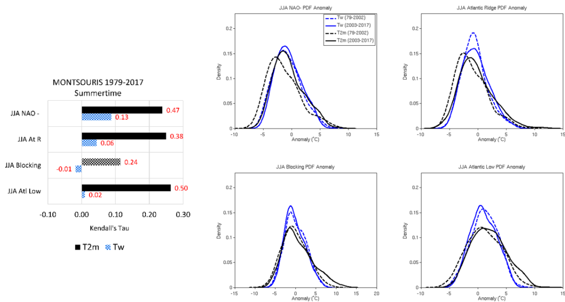
Fig. 4. Same as Figure 3 but for summer weather regimes
