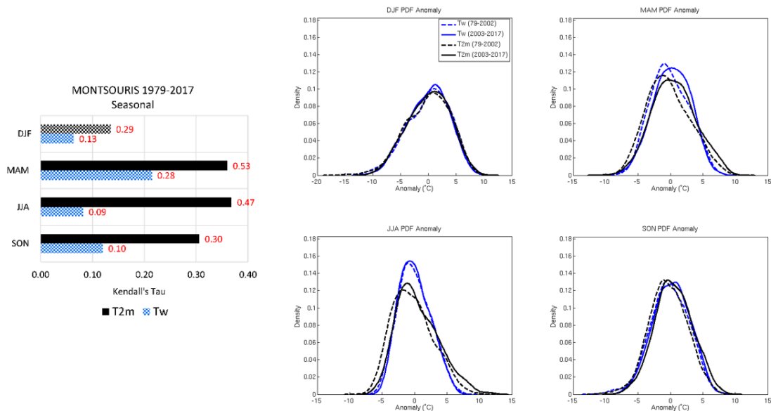
Fig. 3. Left: Mann Kendall seasonal trends for T2m in black and Tw in blue. The red value represents the Sen slope in units per decade. A solid bar indicates a significant trend for a confidence interval of p
