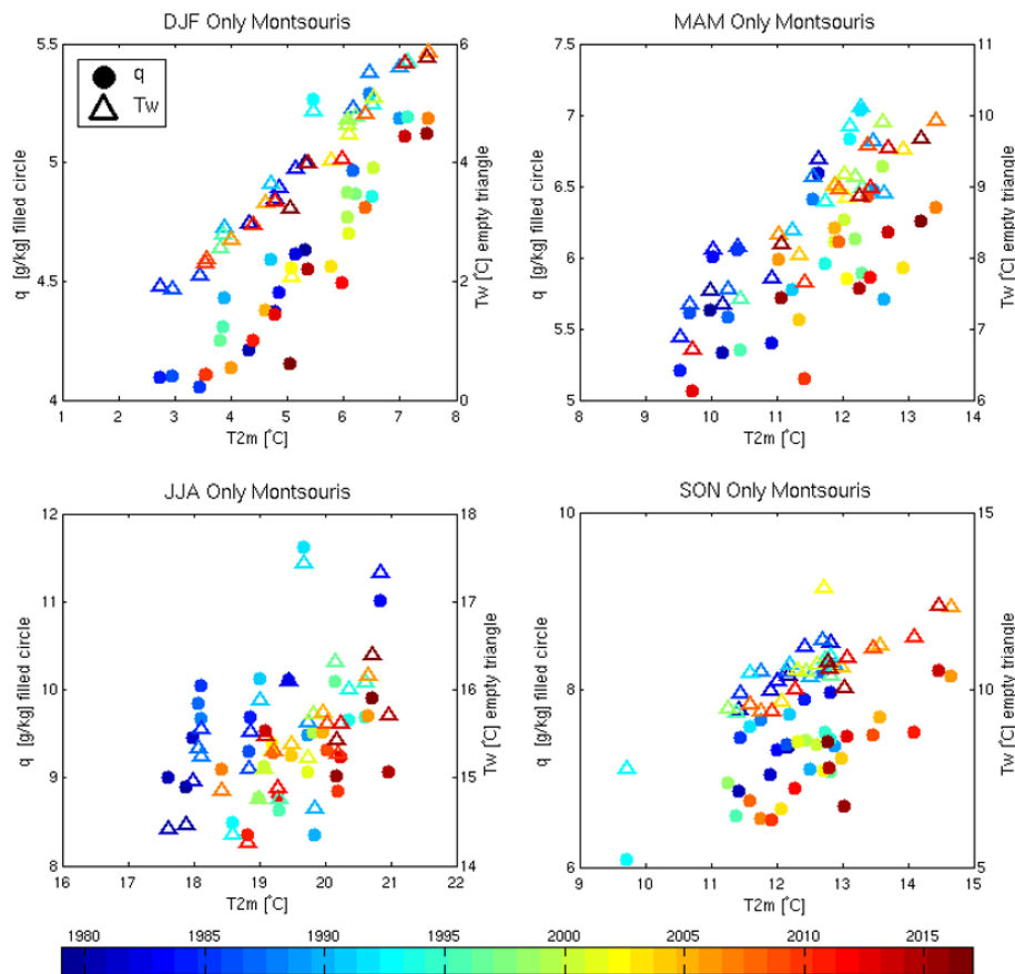
Fig. 6. T_{2m} – q seasonal relationship in Montsouris in filled circle, and T_{2m} – T_w seasonal relationship in Montsouris in empty triangle. Each point represents the seasonal average of one year.
