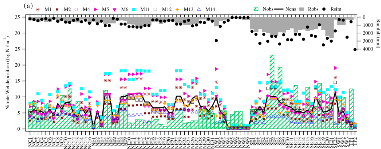
6 Figure S1. Yearly flux of N_{ox} wet deposition simulated by participant models in MICS-Asia III and observation in China (a)
