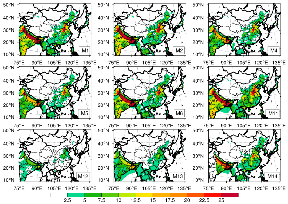
16 Figure S4. Same as Figure S3 but for N_{rd} dry deposition
