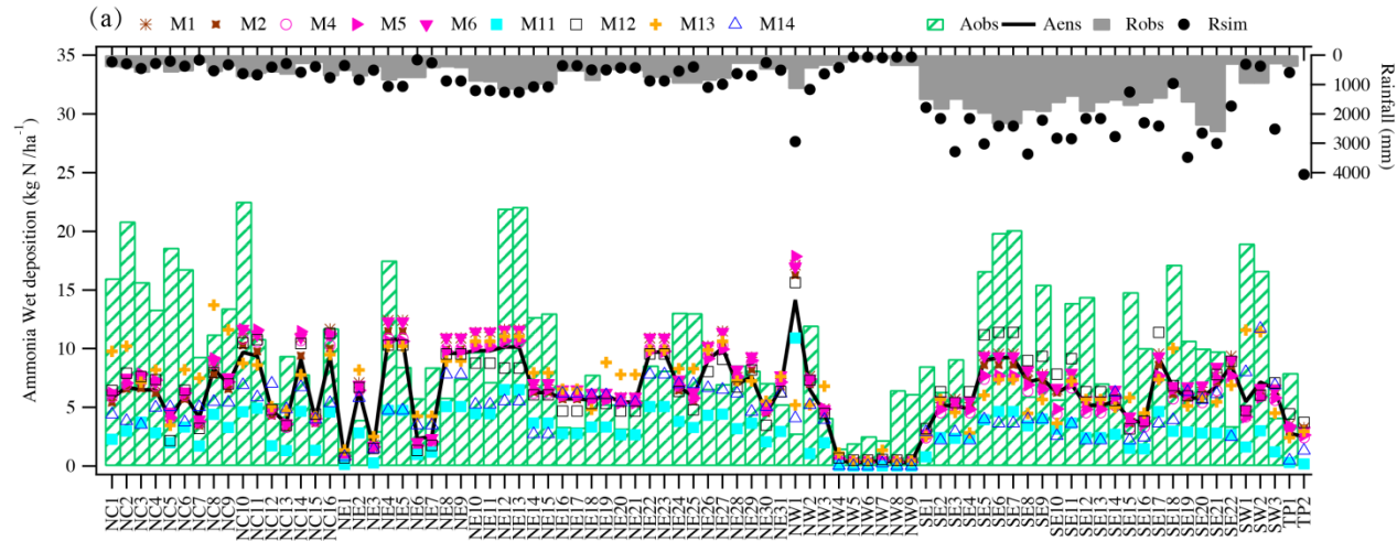
Figure S2. Same as Figure S1 but for N_{rd} wet deposition
