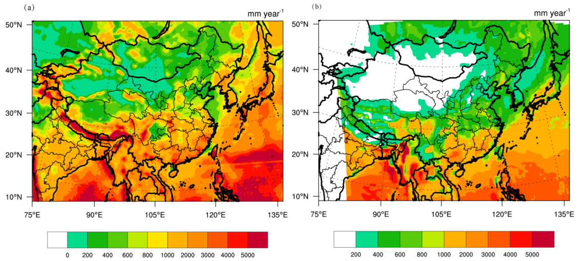
Figure S5. Annual rain volume simulated by WRF (a) and RAMS(b) during in MICS-Asia III
